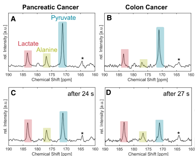
Figure 2. 1D 13 C NMR spectra of maximal pyruvate and lactate signals of a mouse bearing a pancreatic tumor-xenograft (A,C) and of a mouse bearing a colon cancer tumor-xenograft (B,D). A,B: Maximal pyruvate signal 15 s after injection of pyruvate into a mouse bearing a pancreatic tumor-xenograft (A) and into a mouse bearing a colon cancer tumor-xenograft (B). C: Maximal lactate signal 24 s after injection into pancreatic tumor-xenograft. D: Maximal lactate signal 27 s after injection into colon cancer tumor-xenograft. The pyruvate signal (blue) is at 171.1 ppm, the alanine signal (green) at 176.8 ppm and the lactate signal (red) at 183.3 ppm. The signal marked with an asterisk is from a urea reference.
