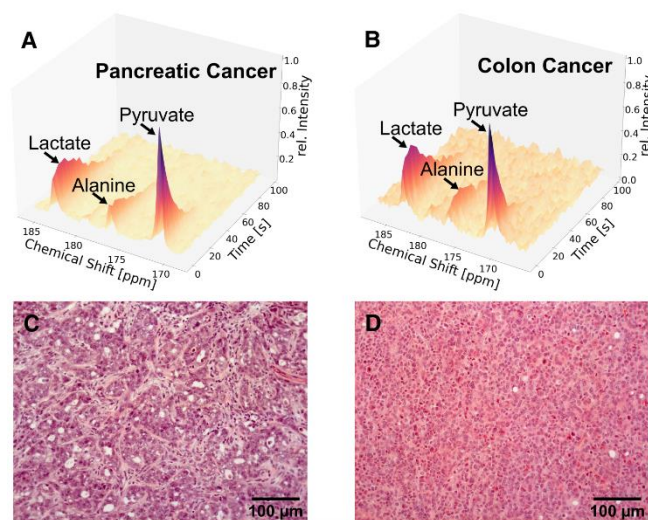
Figure 1. 13 C NMR spectra upon injection of hyperpolarized 1- 13 C-pyruvate-d 3 into a mouse bearing pancreatic (A) or colon cancer (B) tumor-xenografts. The pyruvate signal appears at 171.1 ppm, the alanine signal at 176.8 ppm and the lactate signal at 183.3 ppm. The spectra were acquired 15 s after injection, every 3 s with a flip angle of 22°. Signals were normalized to the highest intensity. Tissue sections from a pancreatic (C) and a colon cancer tumor-xenograft (D) were stained with H&E.
