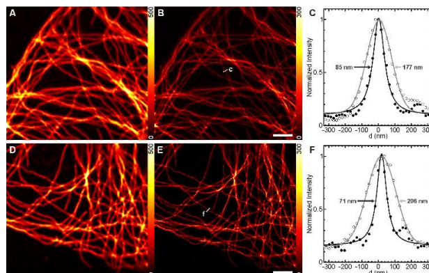
Figure 5. Confocal (A, D) and STED (B, E) images of U2OS cells stained with a primary antibody against tubulin and a secondary nanobody labeled with DPP-COOH-Male and mounted in PBS supplemented with CB7. STED was performed with a 655 nm laser (B) or with a 595 nm laser (E), both at approximately same power. (C, F) Confocal (empty symbols) and STED (filled symbols) line-profiles across a single filament from the indicated positions. Data was fit to a Gaussian function (Confocal) and a Lorentzian function (STED), with the corresponding FWHM indicated. Scale bars: 2 \mu\text{m} .
