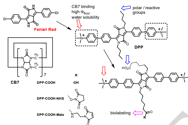
Figure 1. Fluorophore design related to Ferrari Red pigment. The structures of guest molecules prepared in this work - 3,6-diaryl-2,5-dihydropyrrolo[3,4-c]pyrrole-1,4-diones ( DPP ), DPP-COOH ; as well as amino and thiol reactive probes ( DPP-COOH-NHS and DPP-COOH-Male , respectively); the host cucurbit[7]uril molecule ( CB7 ).
