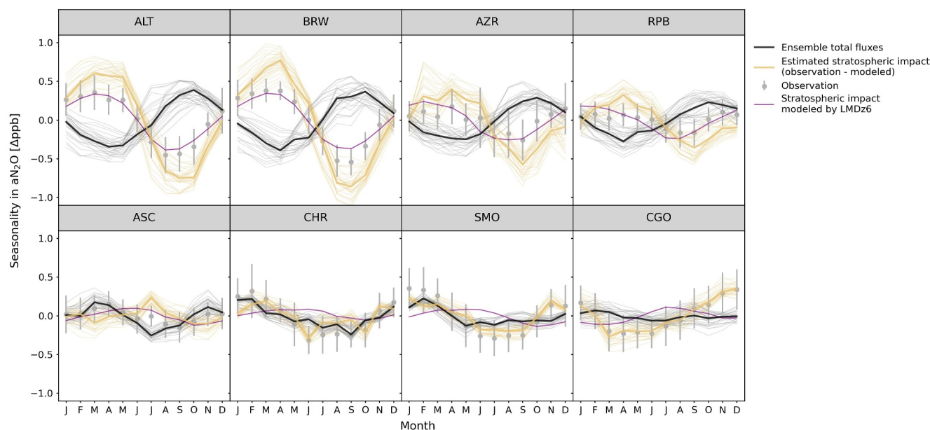
Figure 4. Mismatch (yellow lines) between observed (solid gray circles) and modeled aN 2 O seasonality (black lines) at different NOAA/CCGG flask stations (ALT: Alert, BRW: Barrow, AZR: Terceira Island, RPB: Ragged Point, ASC: Ascension Island, CHR: Christmas Island, SMO: Samoa, CGO: Cape Grim) for present day (2001–2020). Thick lines indicate multi-model median and thin lines indicate individual models. Vertical lines on gray circles indicate the standard deviation from temporal variability weighted by measurement uncertainty. The observation-model mismatch (observed—modeled N 2 O mixing ratio) provides an estimate of the stratospheric contribution to aN 2 O seasonality from N 2 O loss and resulting stratosphere-troposphere net fluxes. A modeled stratospheric tracer of N 2 O indicating stratospheric contribution for the same period using the chemistry-transport model, LMDz6 (see Ruiz and Prather (2022) for methods), is shown in purple lines for comparison.
