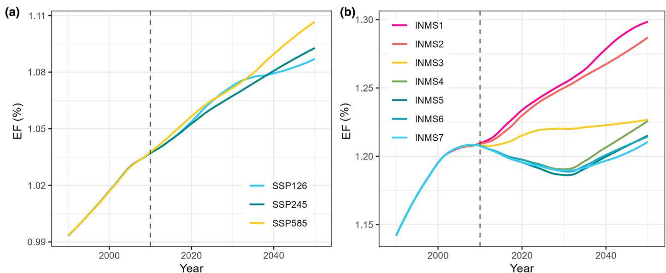
FIGURE 6 Global cropland and pasture emission factor (EF) changes under different scenarios. This figure displays smoothed lines reflecting changes in EF. (a) The change in EF compared to the average EF during 1990–2010, excluding nitrogen fertilizer impacts under scenarios SSP126, SSP245, and SSP585. (b) The change in EF compared to the average EF during 1990–2010 including nitrogen fertilizer effects under scenarios INMS1 to INMS7.
