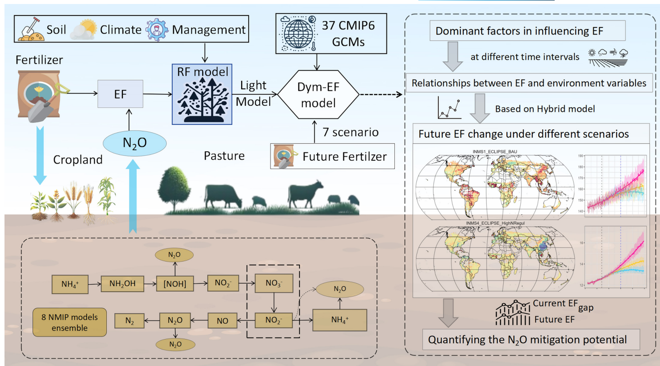
FIGURE 1 Modeling framework integrating machine learning and process-based model ensembles (NMIP2) for assessing global nitrogen fertilizer input-induced nitrous oxide ( \text{N}_2\text{O} ) emission factors (EFs) and projecting EF change under various climate and N management scenarios. The NMIP2 was performed under 0.5^\circ \times 0.5^\circ resolution. This modeling framework was used to emulate the NMIP2 ensemble behaviors rather than individual NMIP2 models. RF, Random Forest model; seven scenarios including INMS1, business-as-usual; INMS2, low N regulation (Low ambition); INMS3, medium N regulation (moderate ambition); INMS4, high N regulation (High ambition); INMS5, best case (High ambition); INMS6, best-case plus (High ambition); INMS7, Bioenergy (High ambition); NMIP, global \text{N}_2\text{O} model intercomparison project. Dym-EF, Dynamic EF.
