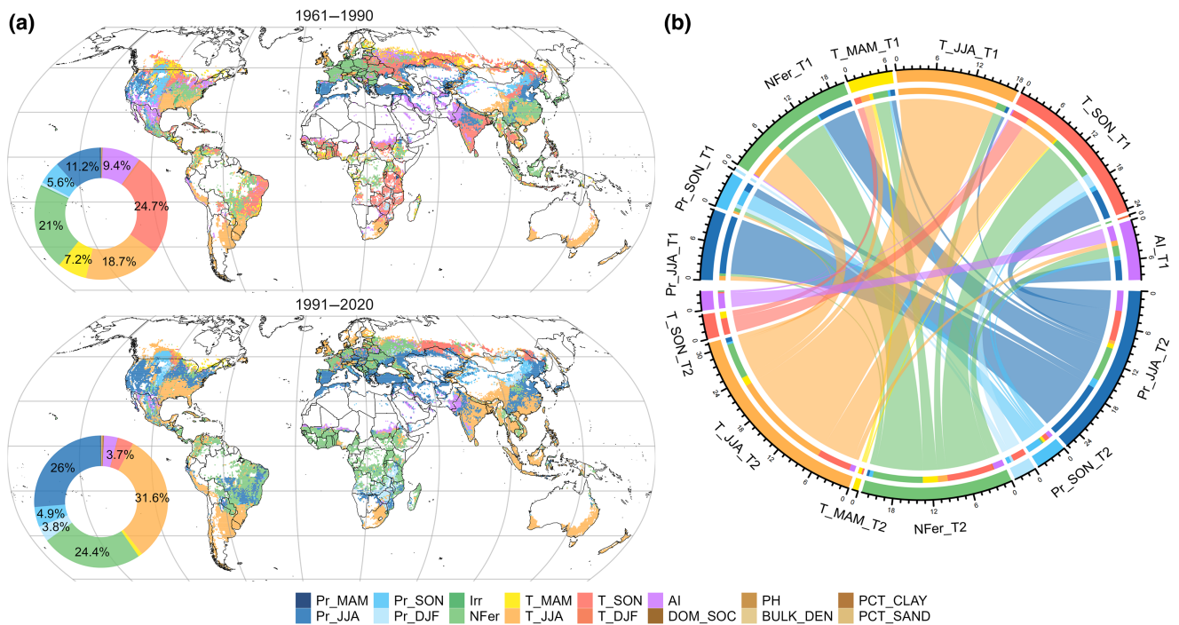
FIGURE 2 The dominant driver of N_2O emission factor (EF) at each pixel and the partial dependence of EF on different variables. (a) Spatial map showing the primary factors influencing EF, with pie charts depicting the percentage area of dominant factors across different time intervals and scenarios. (b), Chord diagram to demonstrate the shift of the dominant factor in influencing EF from T1 (1961–1990, upper half of circle) to T2 (1991–2020, lower half of circle). Numbers represent the percentage of the area influenced by each variable, with different colors indicating different variables. Linked variables (such as T_SON_T1 to NFer_T2) illustrate the shift in dominant factors from T1 to T2. Variables consist of Irr (irrigation rate), NFer (nitrogen fertilizer), Pr_MAM (total precipitation in March, April, and May), Pr_JJA (total precipitation in June, July, and August), Pr_SON (total precipitation in September, October, and November), Pr_DJF (total precipitation in December, January, and February), T_MAM (mean temperature in March, April, and May), T_JJA (mean temperature in June, July, and August), T_SON (mean temperature in September, October, and November), T_DJF (mean temperature in December, January, and February), and AI (aridity index); DOM_SOC, soil organic carbon; BULK_DEN, soil bulk density. Map lines delineate study areas and do not necessarily depict accepted national boundaries.
