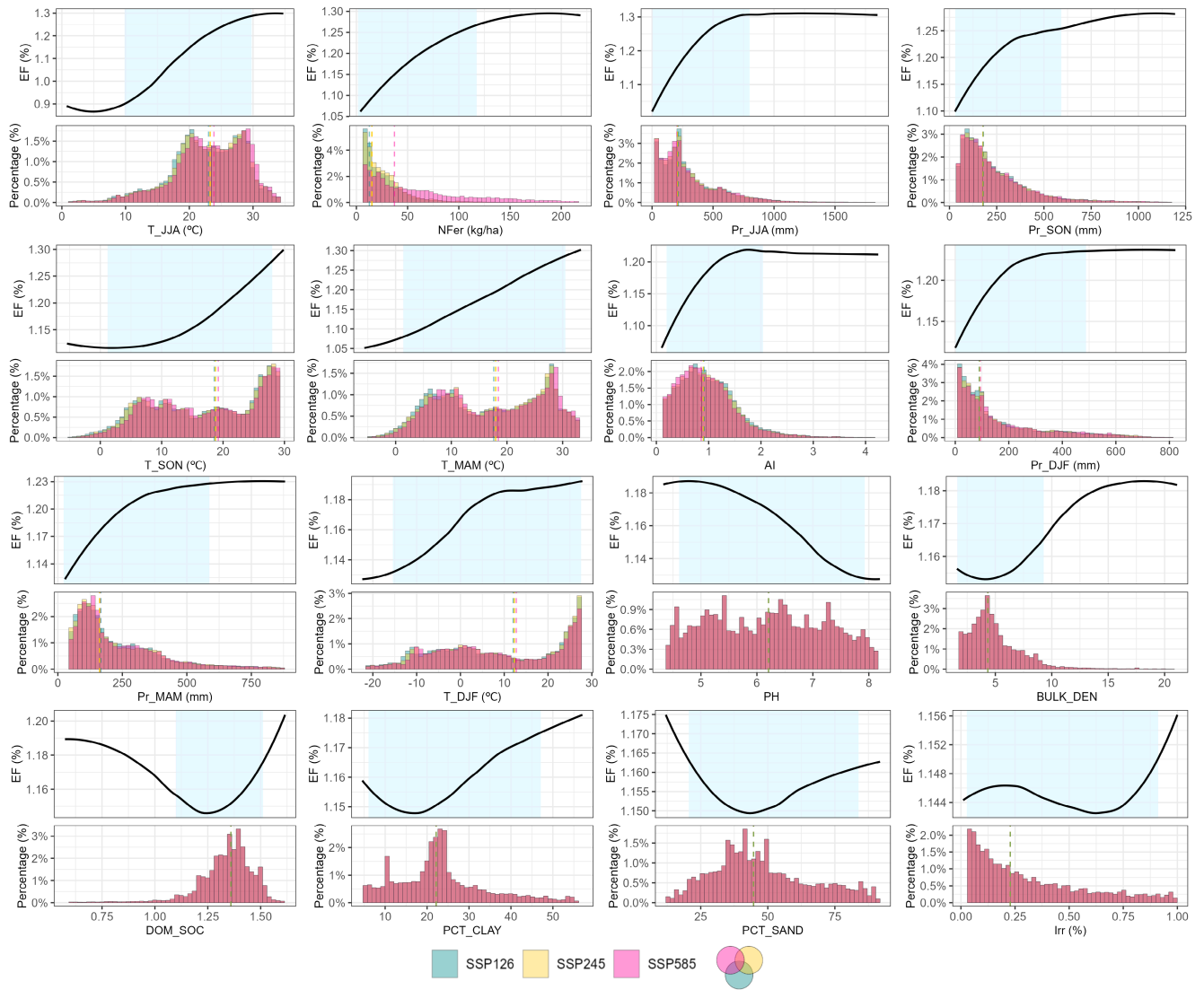
FIGURE 3 Partial dependence plots for annual emission factor change across different predictors (ranked by feature importance see Figure S7). The smooth black lines depict the average model's response, alongside fitted values for the calibration data. Histograms display the probability distributions for the indices of SSP126, SSP245, and SSP585 scenarios in 2050. The blue shaded area denotes calibration data ranging between the 5th and 95th percentiles.
