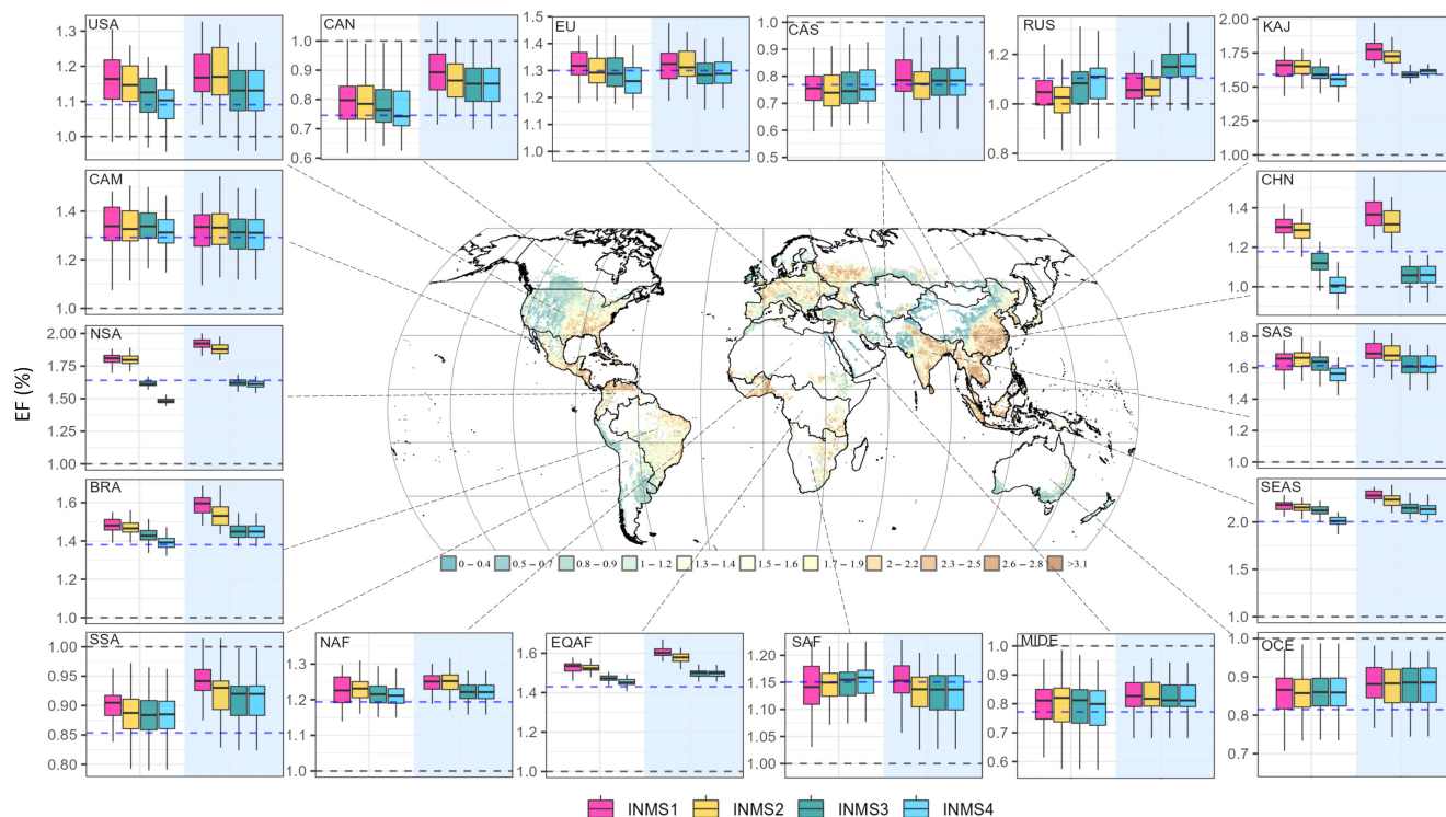
FIGURE 4 Projected \text{N}_2\text{O} emission factor (EF) across various subregions in 2030 (white area) and 2050 (blue-shaded area). The spatial map indicates the median EF estimated by NMIP ensembles in 2010. The black dashed line in each panel represents the Tier-1 EF (1%), and the blue dashed line indicates the 2010 EFs based on a multi-model median (extracted from the central map). INMS1–S4 represents four nitrogen management scenarios (Table 1). Box boundaries show the 25th and 75th percentiles of EF estimates, and whiskers below and above the box indicate the estimate range driven by climate data from 37 GCMs. The median is indicated by the black line within each box. BRA, Brazil; CAM, Central America; CAN, Canada; CAS, Central Asia; CHN, China; EQAF, Equatorial Africa; EU, Europe; KAJ, Korea and Japan; MIDE, Mideast; NAF, Northern Africa; NSA, Northern South America; OCE, Oceania; RUS, Russia; SAF, Southern Africa; SAS, South Asia; SEAS, Southeast Asia; SSA, Southwest South America; USA, The United States of America.
