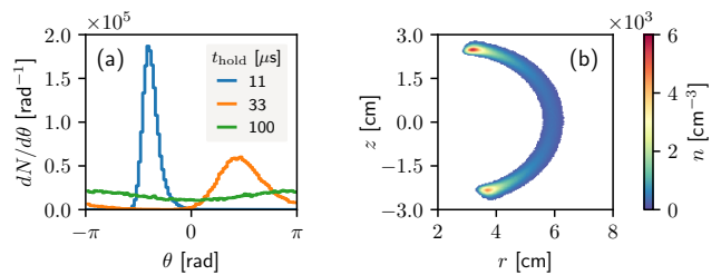
FIG. 5. Simulated (a) toroidal and (b) poloidal distribution of N = 10^5 e^+ in the dipole trap with U_m = +14 V. The color range in (b) has been clipped to show 90% of the distribution, which occupies a volume of \sim 160 \text{cm}^3 .
