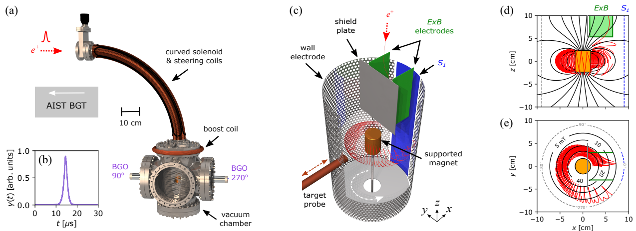
FIG. 1. (a) Dipole trap and \gamma -ray detectors; the target probe mounts to the nearside flange that has been omitted from the illustration to reveal the trap location. (b) Example of the delayed annihilation signal that signifies successful injection. (c) Supported magnet (orange), E×B (green), S_1 (blue), and wall electrodes (partial cutaway view), shield plate, and retractable target probe. The red path represents a calculated trajectory for a 6-eV positron in static injection fields; the white curved arrow (dash-dot) shows the drift direction. The trajectory is projected onto the xz and xy planes in (d) and (e), respectively. (d) Dipole magnetic field lines ( y = 0 ). (e) Contours of magnetic field strength [mT] in the midplane of the magnet ( z = 0 ).
