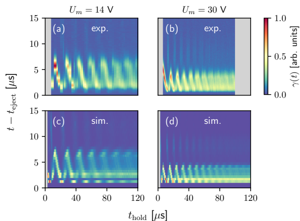
FIG. 4. (a, b) Measured (sum of all three BGO detector data sets) and (c, d) simulated annihilation signal for a range of short hold times in the dipole trap with the magnet case biased to either (a, c) U_m = +14 V or (b, d) +30 V.
