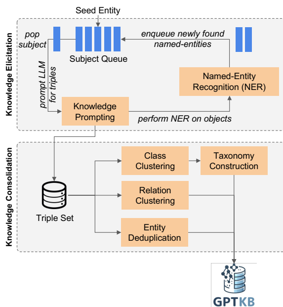
Figure 1: Overview of our approach for LM-based KB construction.
