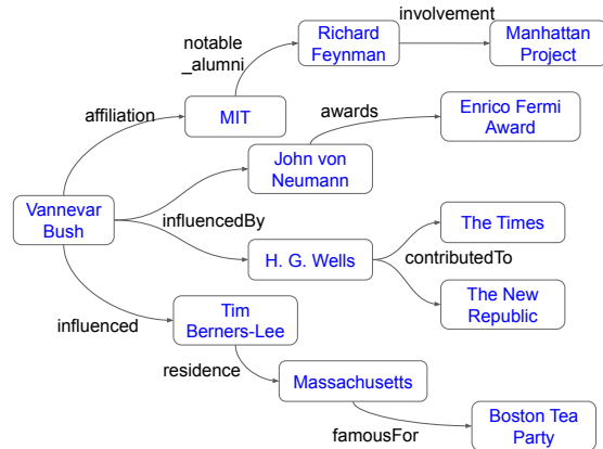
Figure 2: Graph exploration from seed entity Vannevar Bush .
