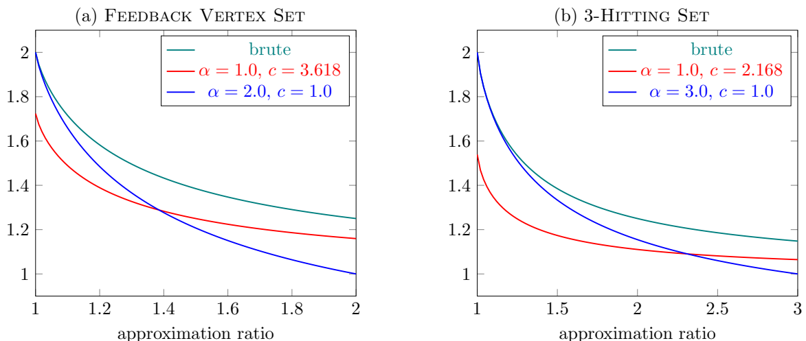
Figure 2: The figure shows running times for FEEDBACK VERTEX SET and 3-HITTING SET. A dot at (\beta, d) means that the respective algorithm outputs an \beta -approximation in time O^*(d^n) .
