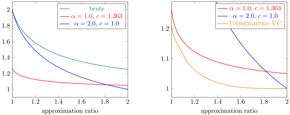
Figure 1: The left figure shows running times for WEIGHTED VERTEX COVER and right side provides a comparison to UNWEIGHTED VERTEX COVER. A dot at (\beta, d) means that the respective algorithm outputs an \beta -approximation in time \mathcal{O}^*(d^n) .
