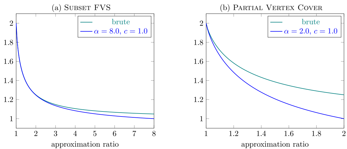
Figure 4: The figure shows running times for SUBSET FVS and PARTIAL VERTEX COVER. A dot at (\beta, d) means that the respective algorithm outputs an \beta -approximation in time O^*(d^n) .
