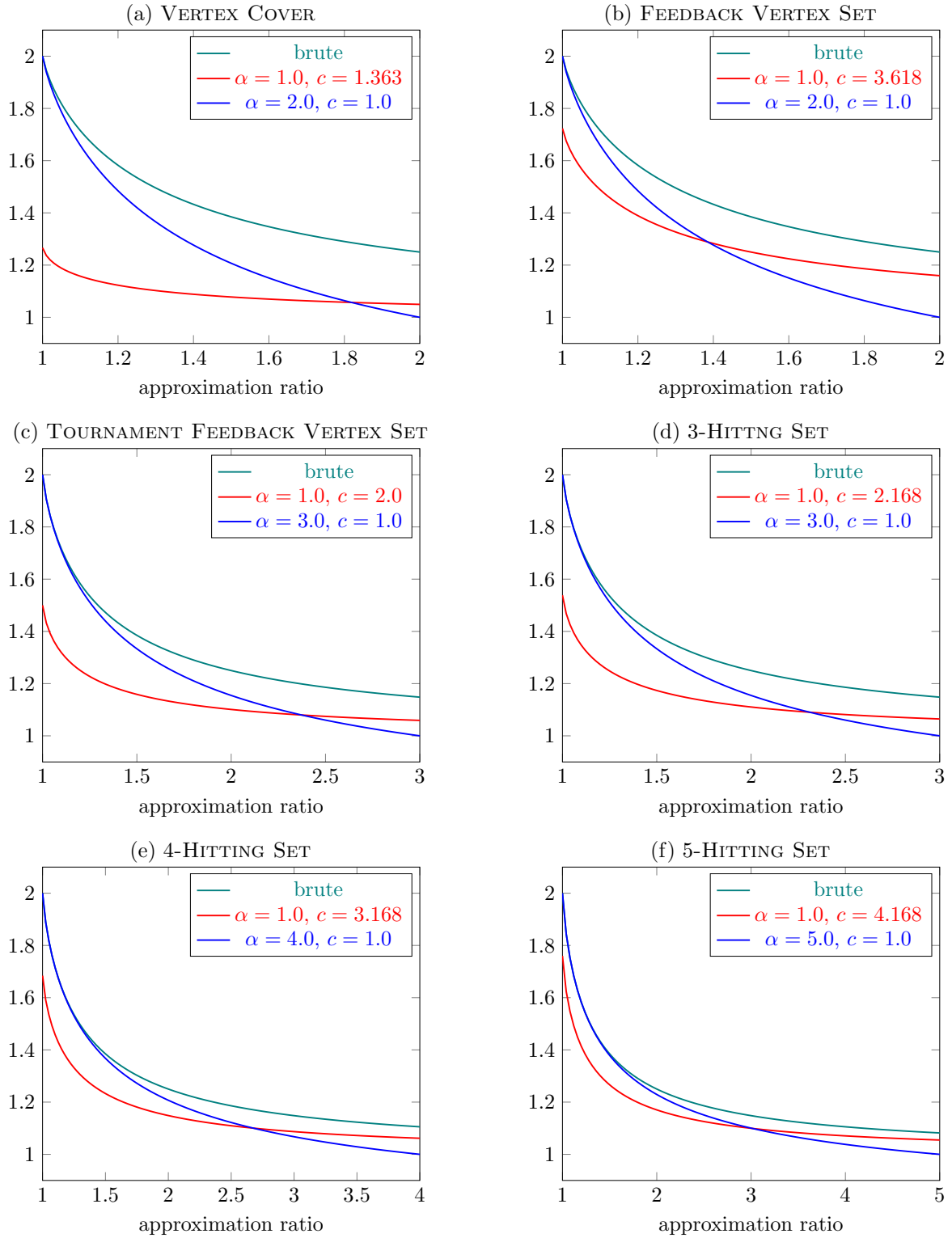
Figure 3: The figure shows running times for VERTEX COVER, FEEDBACK VERTEX SET, TOURNAMENT FEEDBACK VERTEX SET, 3-HITTING SET, 4-HITTING SET and 5-HITTING SET. A dot at (\beta, d) means that the respective algorithm outputs an \beta -approximation in time O^*(d^n) .
