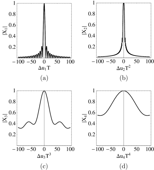
FIG. 4. Estimating the number of global-correlation hypersurfaces which contribute significantly to the detection statistic. In each plot both axes are dimensionless. Further details are given in the text.
