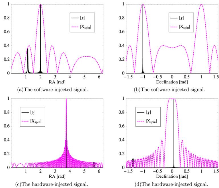
FIG. 10 (color online). Comparison of |X| (solid curves) computed using \Phi_{\text{orb}}(t) and |X_{\text{spin}}| (dashed curves) calculated using \phi_{\text{spin}}(t) as functions of sky position. In (a) and (b) the signal's phase parameters correspond to the software injection of Sec. V A, and (c) and (d) refer to the hardware-injected signal introduced in Sec. V B. In (a) and (c), |X| and |X_{\text{spin}}| are shown as functions of right-ascension template-value \alpha for the given signal-value \alpha_S , while fixing the remaining template parameters to perfectly match the signal's parameters, \delta_S = \delta , f_S = f , and f_S^{(1)} = f^{(1)} . Whereas in (b) and (d), |X| and |X_{\text{spin}}| are shown as functions of declination template-value \delta , while the remaining template parameters coincide with the signal's phase parameters. One can see that |X| decreases much more rapidly compared to |X_{\text{spin}}| . Therefore |X| dominantly determines the global maximum structure of the detection statistic.
