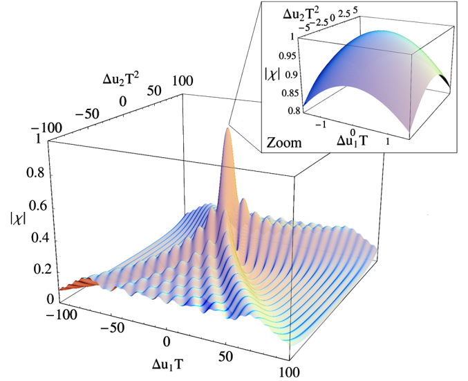
FIG. 2 (color online). Illustration of the simplified detection-statistic amplitude |\mathcal{X}| for m \leq 2 , given by Eq. (38), as a function of the dimensionless parameters \Delta u_1 T and \Delta u_2 T^2 .
