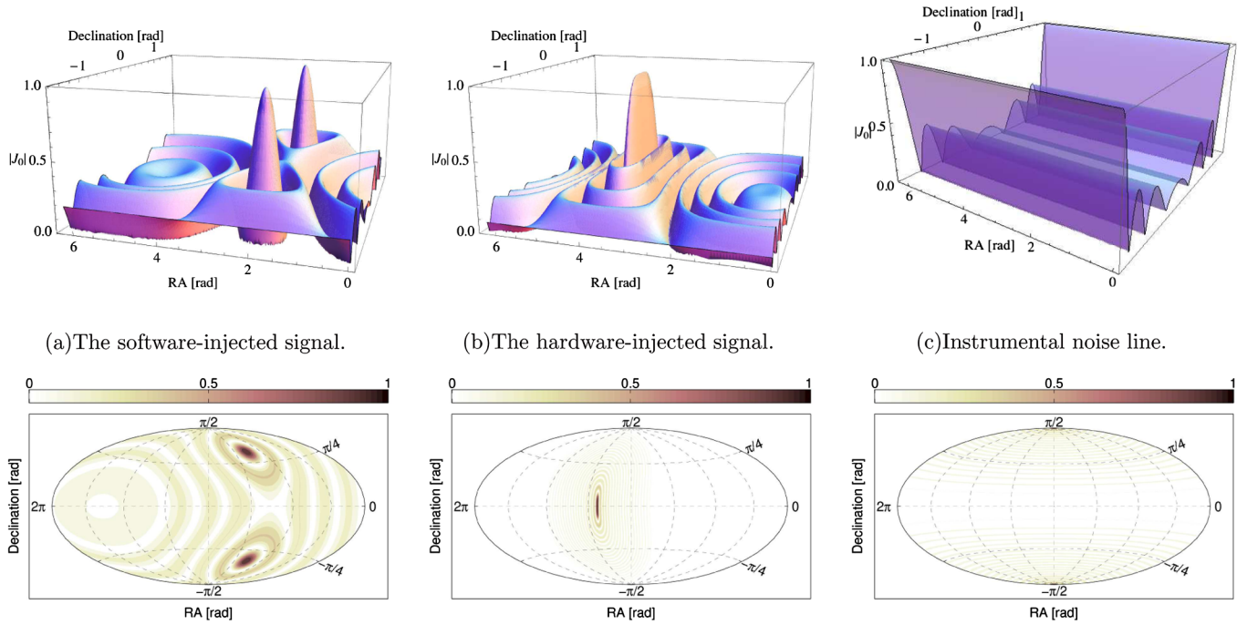
FIG. 9 (color online). Shown is |X_{\text{spin}}| \approx |J_0(\Delta u_{\text{spin}})| over the entire sky using equatorial coordinates of right-ascension \alpha and declination \delta for the three different examples studied previously in this work. The first column corresponds to the software-simulated signal (cf. Fig. 5), the second column to the hardware-injected signal [cf. Fig. 6(a)], and the third column to the instrumental-noise line [cf. Fig. 7(a)]. In the top row, three-dimensional plots of |J_0(\Delta u_{\text{spin}})| as functions of \alpha and \delta are shown, and in the bottom row two-dimensional Hammer-Aitoff projections of the sky are given illustrating the contours of |J_0(\Delta u_{\text{spin}})| .
