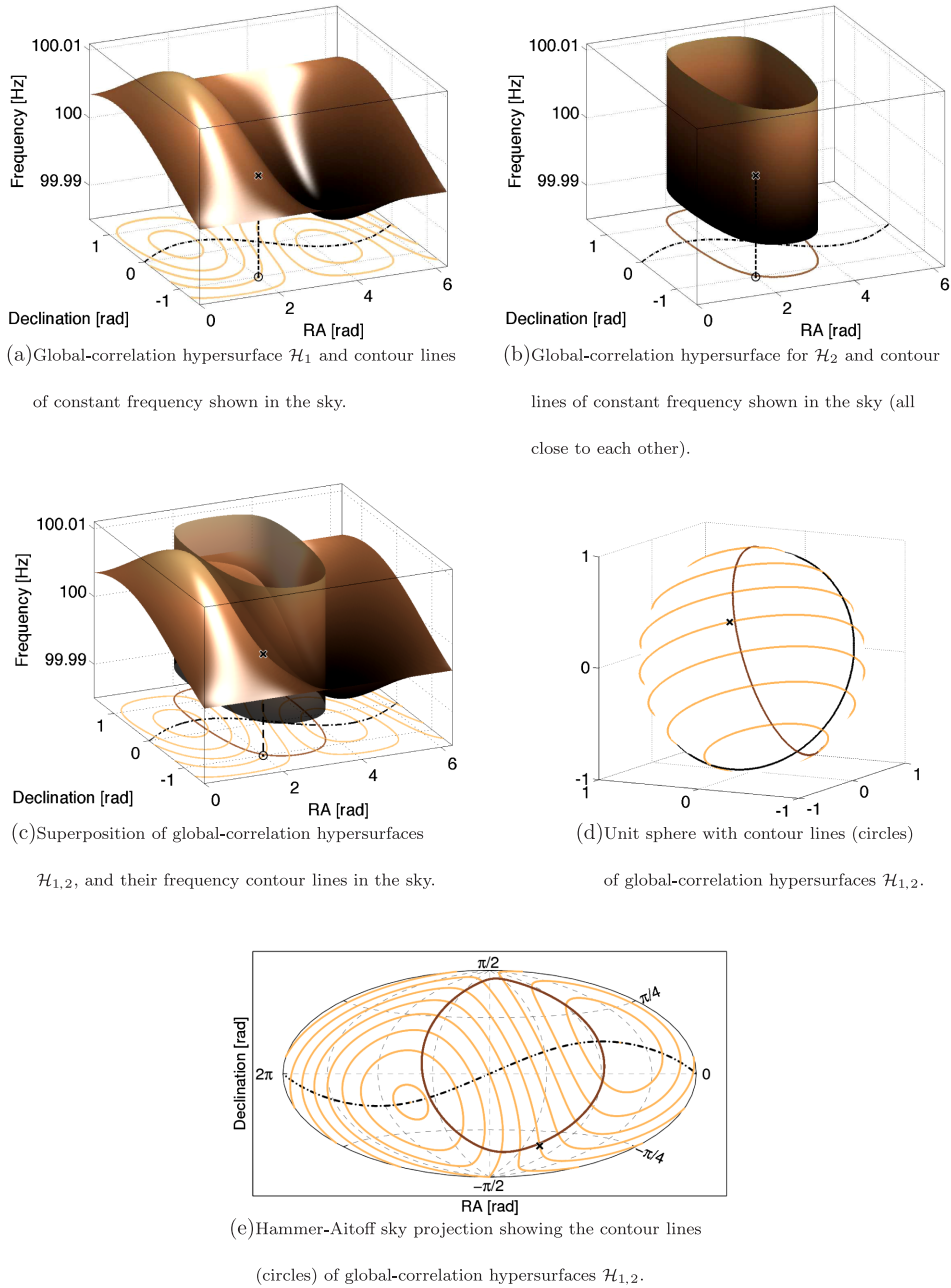
FIG. 3 (color online). The global-correlation hypersurfaces \mathcal{H}_1 ( \Delta u_1 = 0 ) and \mathcal{H}_2 ( \Delta u_2 = 0 ) for a given CW signal shown in the three-dimensional subspace \{f, \mathbf{n}\} at the fixed target spin-down of f^{(1)} = -10^{-11} Hz/s. Each plot refers to GPS time 793555944 s. The phase parameters of the signal are \alpha_S = 2.0 rad, \delta_S = -1.0 rad, f_S = 100.0 Hz, f_S^{(1)} = -10^{-10} Hz/s, as indicated by the black cross (black circle) in the subspace \{f, \mathbf{n}\} (in the sky plane). In (c) the superposition of (a) and (b) illustrates the locations of expected maximum detection statistic along the intersection curve of both hypersurfaces. In each plot the light solid contour lines in the sky of constant f (and f^{(1)} ) are of \mathcal{H}_1 , the dark solid contour lines are the ones of \mathcal{H}_2 . These contours of both hypersurfaces, shown in a Hammer-Aitoff projection in (e), actually describe circles on the three-dimensional unit sphere as is visualized by (d). In the sky subspace of this example, the intersection curve approximately coincides with the contours of \mathcal{H}_2 , and due to the mismatch in spin-down the intersection curve does not pass through the signal's true sky-location. The black dotted-dashed curve represents the ecliptic.
