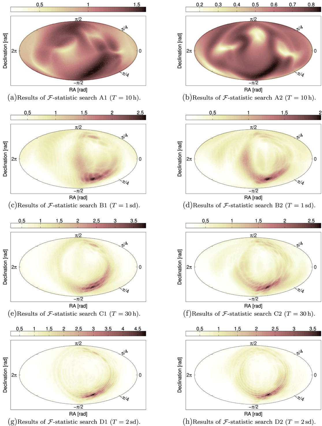
FIG. 5 (color). Hammer-Aitoff sky projections of results from fully coherent \mathcal{F} -statistic searches in the data sets described by Table II. Each data set contained one of the two software-simulated CW sources defined in Table I, where both signals 1 and 2 have identical phase parameters, but different amplitude parameters. The plots of the left (right) column show candidate events registered in the different searches A1, B1, C1 and D1 (A2, B2, C2 and D2) above a threshold of 2\mathcal{F} \geq 2000 ( 2\mathcal{F} \geq 1250 ). The colorbar indicates the values of 2\mathcal{F} \times 10^{-4} . The corresponding analytical prediction by the global-correlation equations has been illustrated earlier by Fig. 3(e).
