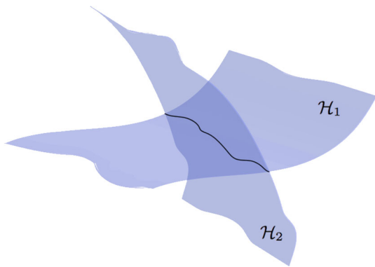
FIG. 1 (color online). Schematic drawing of intersection of two representative global-correlation hypersurfaces \mathcal{H}_1 and \mathcal{H}_2 . The region of intersection, shown by the solid black curve, describes the global maximum-structure of the simplified detection-statistic \mathcal{F}^* , because the expectation value of \mathcal{F}^* is maximal in these locations. For illustration purposes only two hypersurfaces are shown, whereas in general one might need to consider more hypersurfaces.
