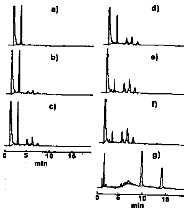
Figure 1. Supercritical fluid chromatograms of the course of photo-oxidation of nimbin, at a) zero time, b) 15 min, c) 30 min, d) 45 min, e) 60 min, f) 75 min and g) after the addition of DABCO and chromatography on a silica gel Chromatotron plate. The two large peaks in g) are from the left, nimbinolide and isonimbinolide.
