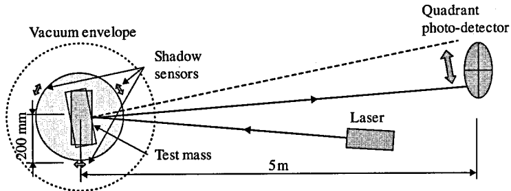
Figure 11.17 The optical lever setup, using a quadrant photodiode placed outside the vacuum envelope.
