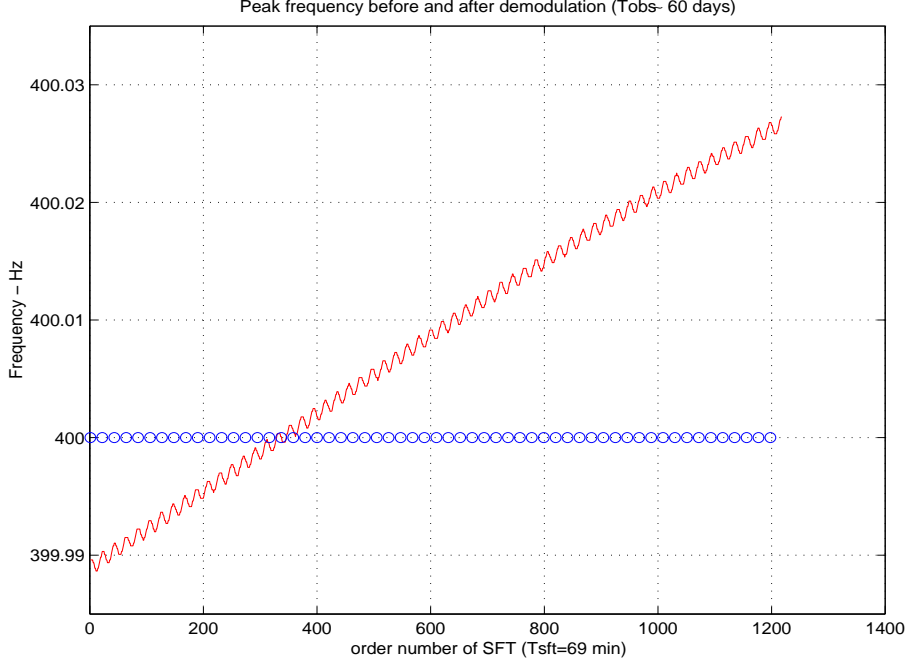
Figure 1: The continuous line shows the position of the instantaneous frequency of a signal coming from a position in the sky with ecliptic coordinates (\beta, \lambda) = (0.0^\circ, 0.0^\circ) and no spin-down parameters. The time-baseline of the SFTs is \sim 1 hour. The circles show the position of the instantaneous frequency after the demodulation procedure. The time-baseline of the DeFTs is \sim 1 day. The intrinsic emission frequency is 400 Hz. Perfect match between template source and signal source was supposed.
