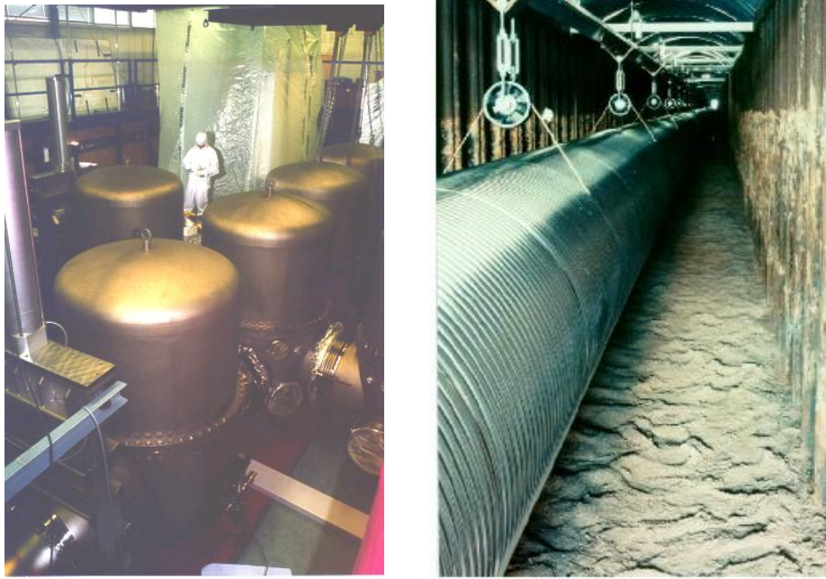
Figure 1. The buildings of GEO 600 are split into three regions with different cleanroom classes: The so-called gallery where people can work with normal clothes, the inner section which has a cleanroom class of 1000 and a movable cleanroom tent installed over open tanks with a class 100 cleanroom. The convolute beam tube has a diameter of 60 cm and a wall thickness of 0.8 mm. The tanks are 2 m tall and accommodate the triple-pendulum suspensions of the interferometer mirrors.
