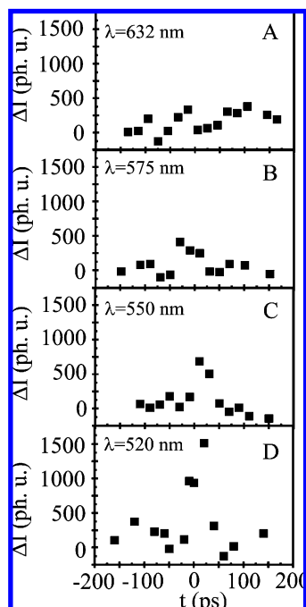
Figure 9. Modulation of the integral intensity of the (012) Bragg diffraction peak as a function of optical excitation wavelength: (A) 632, (B) 575, (C) 550, and (D) 520 nm. The laser power was set to 15 \mu\text{J} for all measurements. The deviation of the values is at maximum 200 counts, an error within the size of the symbols used.
