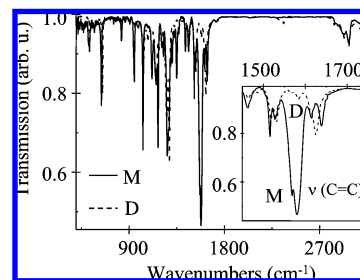
Figure 4. IR transmission spectra of \alpha -styryl(TFMS) in KBr in the monomer (solid line) and dimer phases (dashed line). The strong absorption band at 1580 \text{cm}^{-1} corresponds to the stretching mode of the C=C double bond in the monomer molecule. Its disappearance upon illumination is a strong indicator for the dimerization as the C=C double bond opens to form the cyclobutyl ring.
