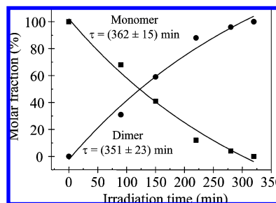
Figure 7. Slow transformation kinetics: time-resolved analysis of the photocrystallographic experiments (580 nm excitation wavelength, 20 mW power). After 350 min of irradiation, the whole crystal has transformed completely from the monomer to the dimer. The determined transformation rates are \tau_{\text{mono}} = 362 \pm 15 min for the decrease of the monomer molar fraction and \tau_{\text{dimer}} = 351 \pm 23 min for the increase of the dimer molar fraction. The experiment was performed under irreversible switching conditions.
