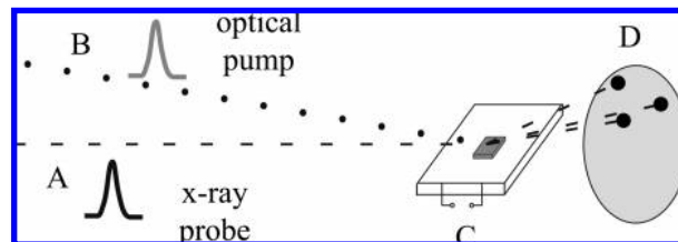
Figure 2. Schematic plot of the grazing incidence setup for the picosecond time-resolved X-ray diffraction experiment. The monochromatized synchrotron X-ray pulses (50 ps pulse width) were selected by a chopper to a frequency of 1 kHz (A). The X-ray beam was focused down to 70 \times 200 \mu\text{m} (vertically \times horizontally), overlapping with a 500 \mu\text{m} focused optical laser beam (B). The energy of the 100 fs laser pulses (1 kHz repetition frequency) was varied between 1 and 25 \mu\text{J} , and the wavelength was chosen between 520 and 632 nm. The sample was grown on an electric heating device ( T = 370 K) (C). The experiment was performed in stroboscopic manner, and the X-ray reflection signals were two-dimensionally collected with an X-ray-sensitive CCD camera (D).
