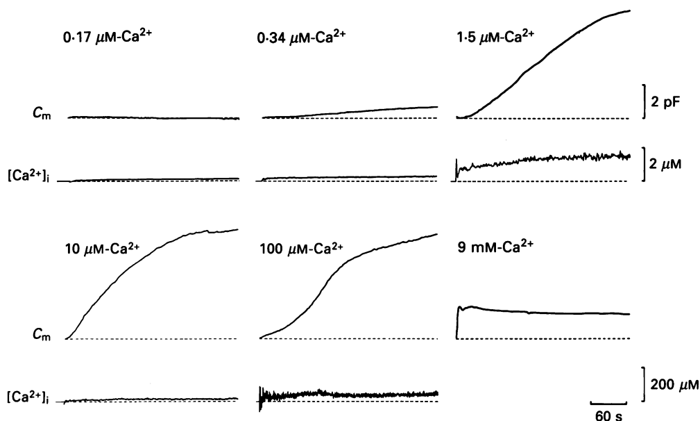
Fig. 3. Changes in C_m induced by dialysis of buffered Ca^{2+} solutions. Elevating [Ca^{2+}]_i produced concentration-dependent changes in the maximum level and rate of rise of C_m . [Ca^{2+}]_i was measured with Fura-2 (upper set of records) or Furaptra (lower set of records). Each pair of C_m and [Ca^{2+}]_i records was taken from a different cell dialysed with internal solutions buffered to the indicated Ca^{2+} concentrations. Initial values for C_m , measured at breakthrough, are indicated by dashed lines.
