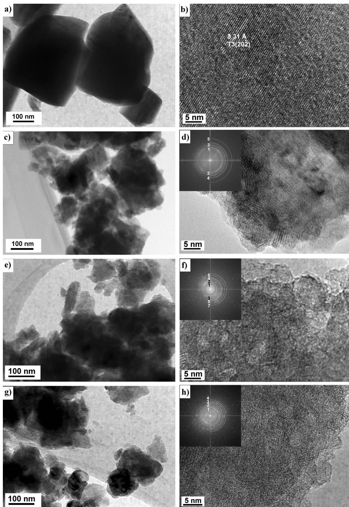
Fig. 3: TEM and HRTEM of hydrogen trititanate crystalline powder. Fast Fourier transform (FFT) of the large area of HRTEM images are shown as the insets with denoted rings. a) TEM and b) HRTEM of sample before milling; T3 – presents \text{H}_2\text{Ti}_3\text{O}_7 ; c) TEM and d) HRTEM 10-min milled sample; e) TEM and f) HRTEM 20-min milled sample; g) TEM and h) HRTEM 40-min milled sample. Assignments of the FFT rings are denoted in text.
