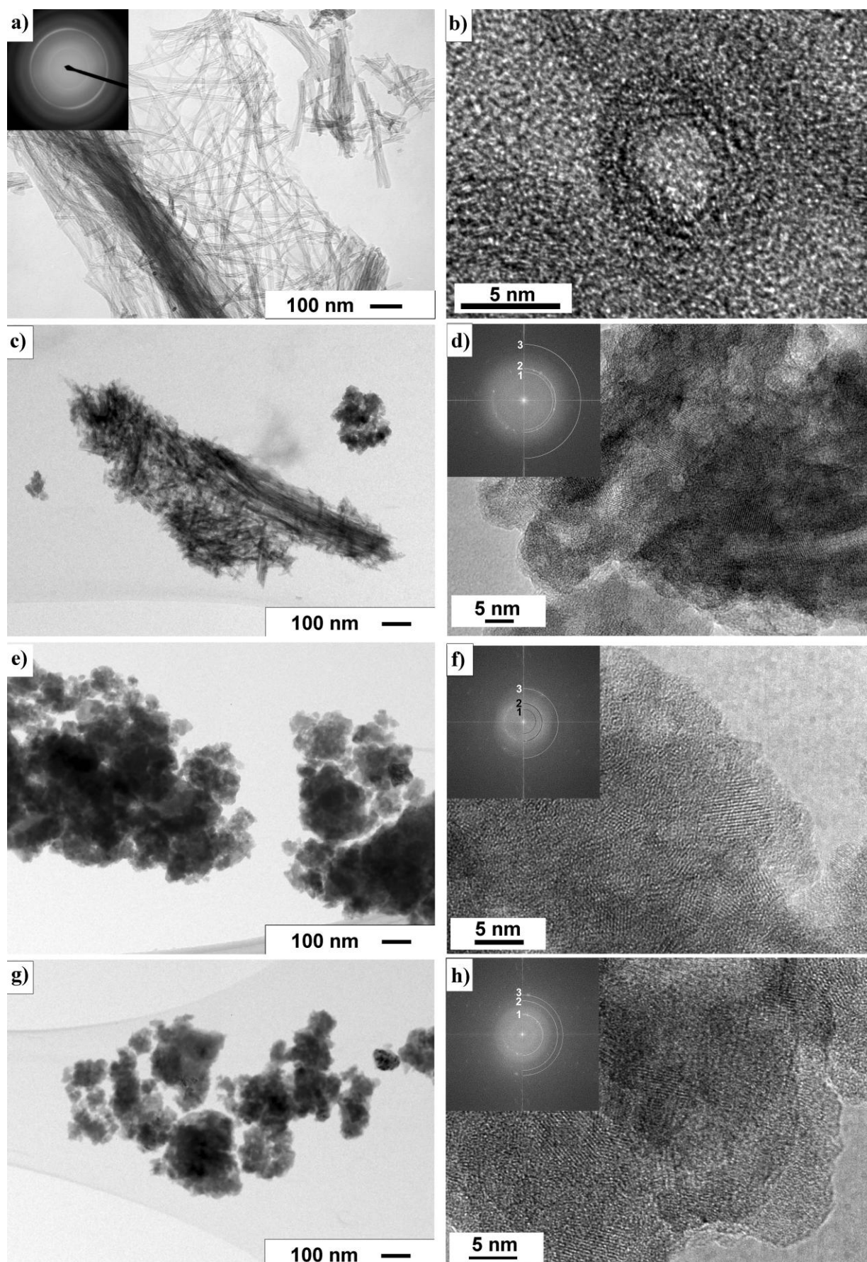
Fig. 4: TEM and HRTEM of hydrogen titanate nanotubes: a) TEM and b) HRTEM of nanotube's cross section before milling; c) TEM and d) HRTEM 10-min milled sample; e) TEM and f) HRTEM of 20-min milled sample; g) and h) milled 40-min. Assignments of the FFT rings are denoted in text.
