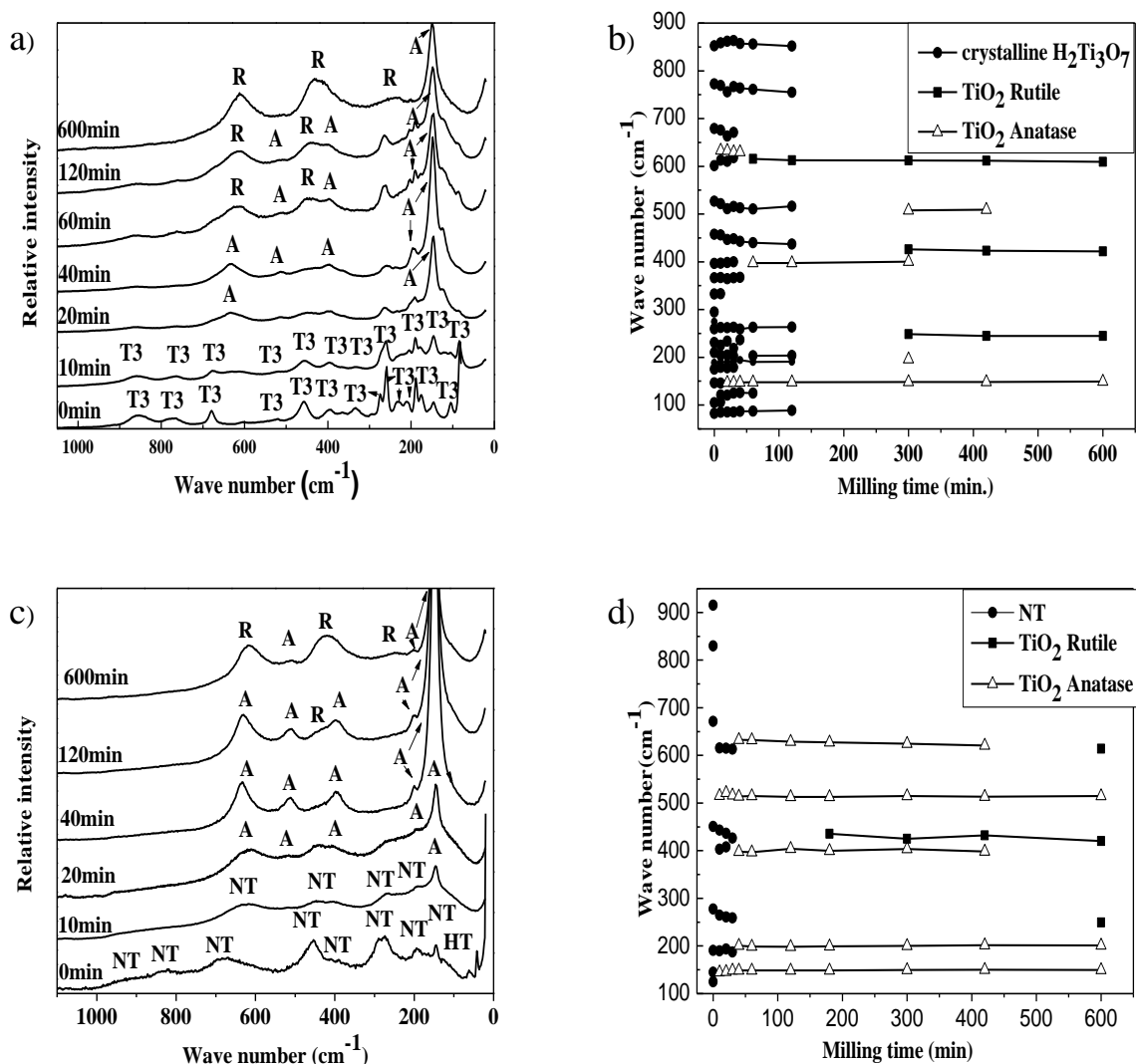
Fig. 1: a) Raman spectra of high-energy ball-milled hydrogen titanate, \text{H}_2\text{Ti}_3\text{O}_7 (T3) crystalline powder b) Raman-band positions as a function of milling time of crystalline sample. c) Raman spectra of high-energy ball-milled hydrogen titanate nanotubes (NT). d) Raman-band positions as a function of milling time of nanotubes. T3 denotes \text{H}_2\text{Ti}_3\text{O}_7 bands, A denotes anatase \text{TiO}_2 bands, R denotes rutile \text{TiO}_2 bands, NT denotes nanotubes bands.
