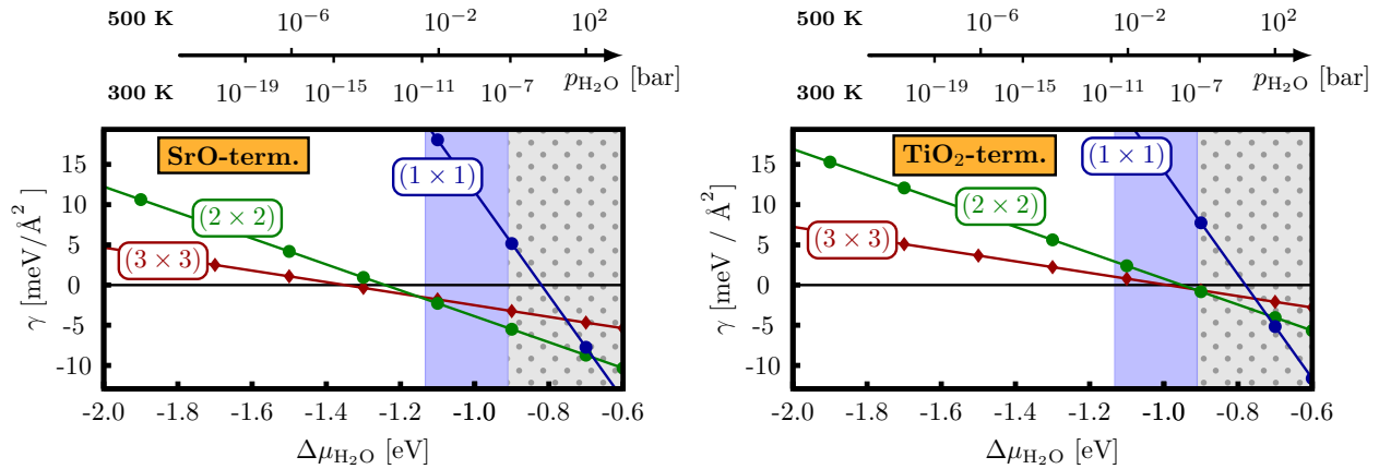
FIG. 8: (Color online) Surface free energies, cf. eq. (2), of the most stable water adsorption geometries at the different coverages at the SrO-termination (left) and TiO 2 -termination (right). In the top x -axis, the dependence on the water chemical potential is converted into pressure scales at 300 K and 500 K. The plain (blue) background boxes mark the region of gas-phase conditions probed by Iwahori et al. in their FFM experiments 6 , while the dotted (gray) boxes indicate the region above the H 2 O-rich limit, i.e. where the present approach assuming equilibrium with water vapor is no longer strictly applicable.
