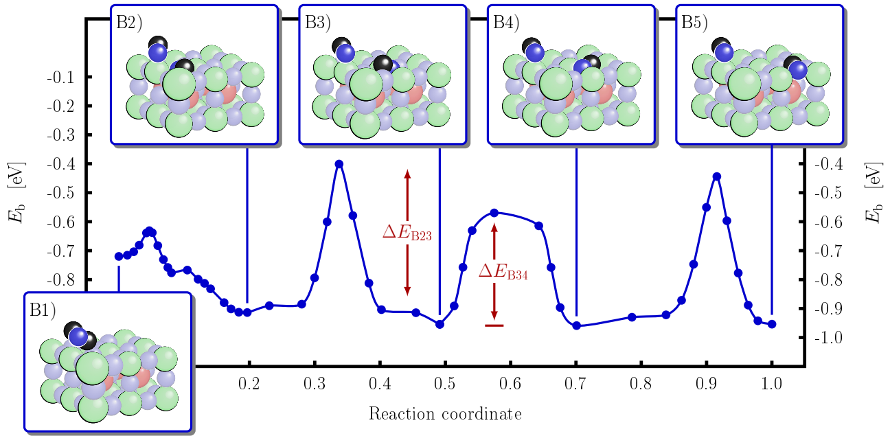
FIG. 7: (Color online) Energy profile for surface diffusion of the split-off H 2 atom over the TiO 2 -terminated surface. The initial states B1 and B2 correspond to the molecular precursor and dissociated hydroxyl-pair shown in Fig. 5. Further disintegration takes place via a hop of the surface H 2 atom to an adjacent lattice O anion (B3) with a barrier \Delta E_{B23} = 0.51 eV, followed by a flip of the orientation of the newly formed hydroxyl group towards the neighboring surface unit-cell (B4) with a barrier \Delta E_{B34} = 0.38 eV. The ensuing equivalent hop to an even more distant lattice O anion (B5) exhibits essentially the same energy profile, indicating overall only small longer-range lateral interactions between the hydroxyl groups.
