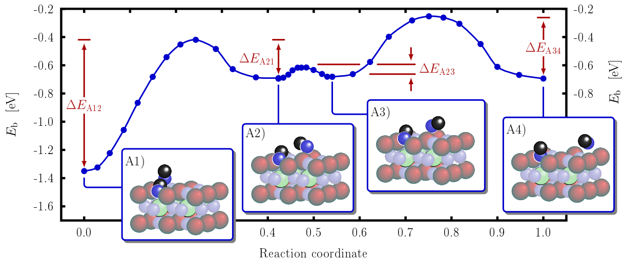
FIG. 4: (Color online) Energy profile for surface diffusion of the protruding O1-H1 hydroxyl group over the SrO-terminated surface. The initial state A1 corresponds to the hydroxyl-pair after the immediate water dissociation process shown in Fig. 3. The transition from state A1 to A2 breaks the hydroxyl-pair and is accompanied by a substantial energetic barrier. Configurations A2 and A3 differ essentially in the mutual orientation of the two hydroxyl-groups, whereas in state A4 the diffusing species has further increased the distance to its original position A1 by hopping to the adjacent binding site.
