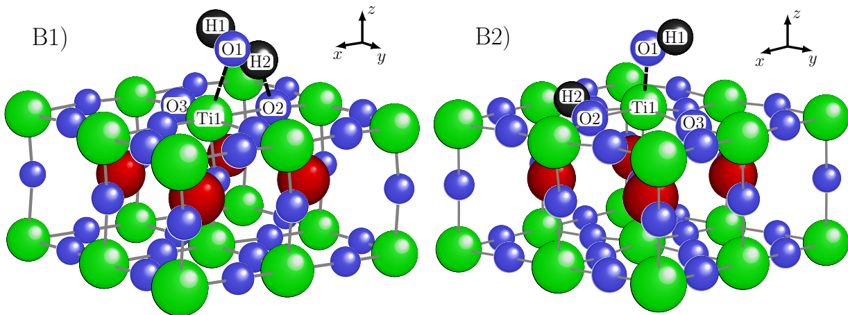
FIG. 5: (Color online) Perspective view of the molecular B1 (left) and dissociated B2 (right) adsorption geometry at the TiO 2 -termination. Atoms discussed in the text and Table I are labeled. In a second dissociated state (not shown), which is energetically equivalent to the state B2, the O1-H1 group is rotated by 180° degrees and thus points in the same direction as the tilted O2-H2 hydroxyl.
