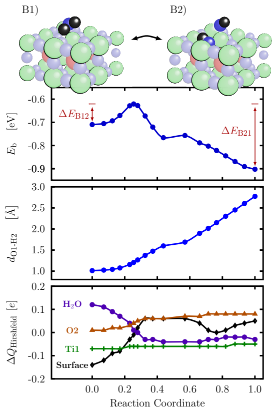
FIG. 6: (Color online) Binding energy, internal O1-H2 bond length and change of the Hirshfeld charges along the reaction pathway from the molecular bound state B1 to the dissociated state B2 at the \text{TiO}_2 -termination. The different atom labels follow the definition given in Fig. 2. The zero reference for the Hirshfeld charges corresponds to gas-phase water and the clean surface.
