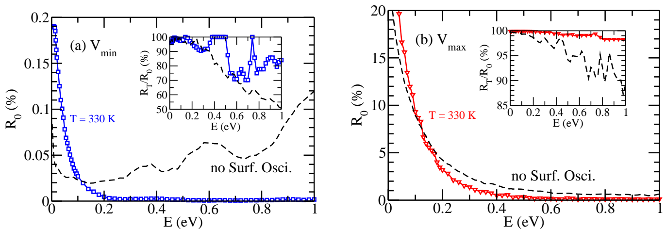
FIG. 7: Reflection coefficient R_0 as function of the incident kinetic energy of singlet oxygen molecules, as calculated by the SH method with a (a) minimal coupling; (b) maximal coupling. The results both within the frozen substrate approximation (dashed lines) and for a three-dimensional surface oscillator (squares and triangles) are shown. In the respective insets, the relative triplet yield R_T/R_0 for both calculations is plotted as well.
