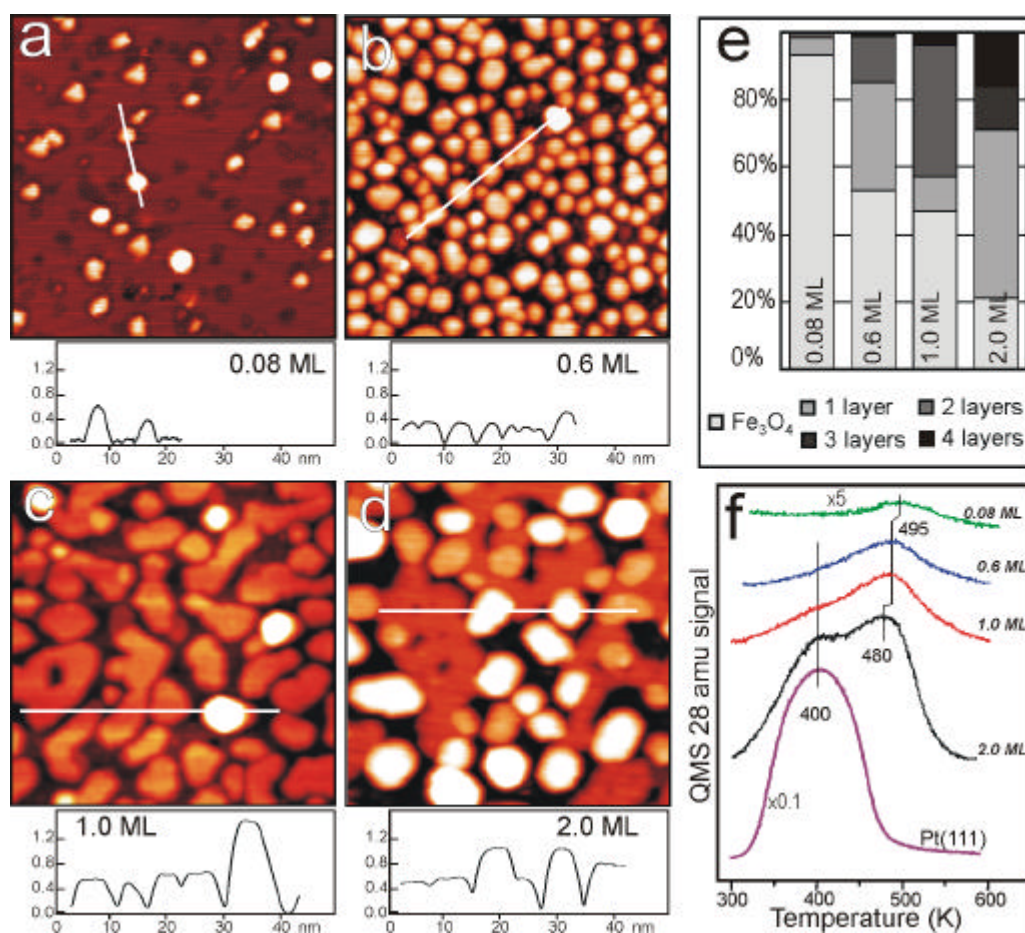
Figure 2. (a-d) STM images (50 nm × 50 nm) of the samples shown in Fig. 1 after subsequent annealing at 600 K for 1 min. Height profiles along the lines are shown below each image. Panel (e) shows each particles' height distribution. TPD spectra of 5 L CO adsorbed at 300 K are shown in (f). The spectrum from the Pt(111) crystal is also shown, for comparison. The spectra are offset for clarity.
