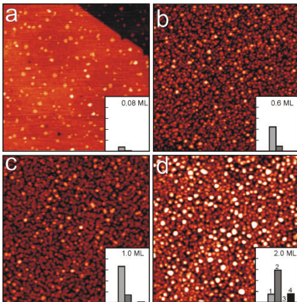
Figure 1. Room temperature STM images (100 nm × 100 nm) of Pt deposited on the Fe 3 O 4 (111) films at ~ 110 K at the Pt coverage as indicated. At the low coverage, the Pt islands are mostly one Pt(111) layer in height. The insets show a normalized particle height histogram indicated in numbers of (111) layers as indicated in the inset (d).
