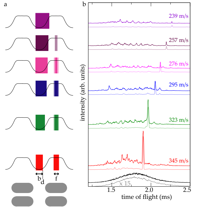
FIG. 7: (Color online) a) Graphical representations of the high-voltage switching parameters b, d , and f , see text for details. b) Deceleration sequence of OH in its low-field seeking ^2\Pi_{3/2}, v = 0, J = 3/2, f state, with the simulated time-of-flight profiles underneath the experimental measurements for different focusing and deceleration parameters. The lowest traces are free-flight profiles. The second (red) traces show the arrival-time distribution for focusing at a constant velocity of 345 m/s. The following traces are TOFs for deceleration from 345 m/s to successively lower final velocities, as noted in the graph.
