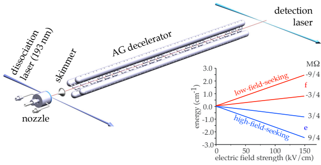
FIG. 2: (Color online) Scheme of the experimental setup. In the inset the Stark shifts of the different M\Omega manifolds of OH radicals in their rovibronic {}^2\Pi_{3/2}, v=0, J=3/2 are shown. See text for details.
