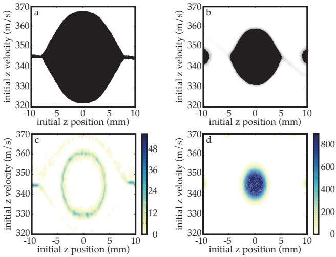
FIG. 6: (Color online) The longitudinal phase-space acceptance for focusing OH radicals in their low-field seeking ^2\Pi_{3/2}, v = 0, J = 3/2, f, M\Omega = -9/4 state. a and b are the acceptance for a one-dimensional model along the molecular beam axis, c and d display the results of the full three-dimensional calculations, where the density (molecules/(mm·m/s)) of the projection of the phase-space acceptance onto the (z, v_z) plane is displayed. In a and c high-voltages are switched analogous to a normal Stark decelerator experiment, whereas in b and d the simulations are performed with the same switching sequence for guiding at 345 m/s as used in the experiments of this work. See text for details.
