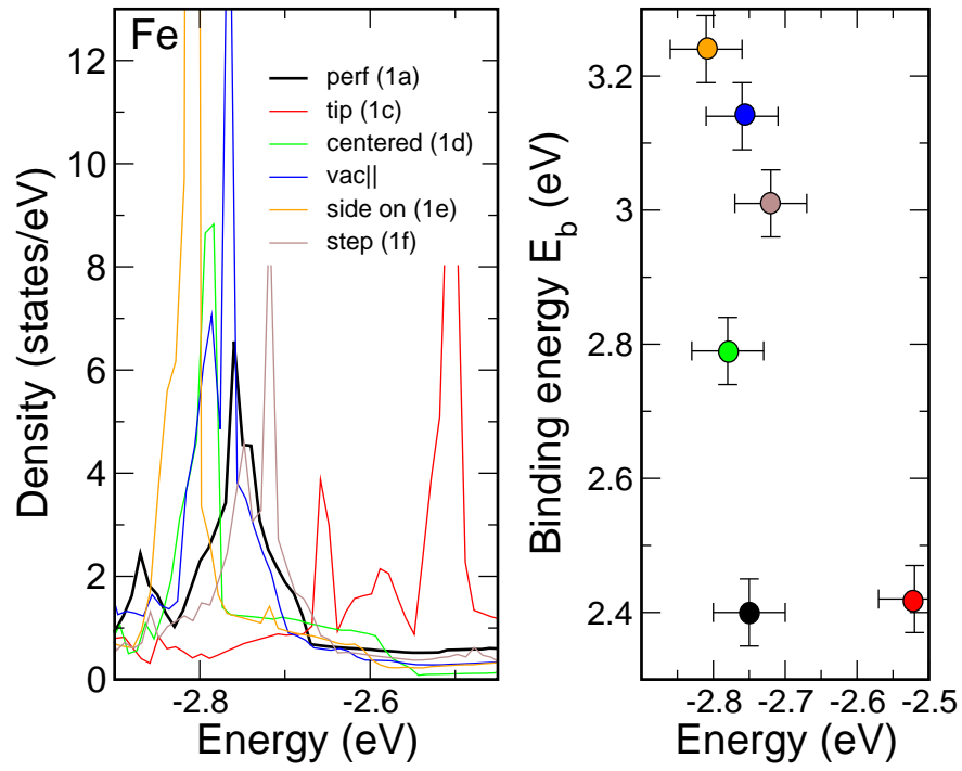
FIG. 3: Left: Projected Fe–DOS of FDT between two perfect and defective Ag(111) contacts. The numbers in the legend are related to Fig. 1. Right: Peak positions of the Fe–peak versus the binding energy for different adsorption geometries. The color code corresponds to the legend, too.
