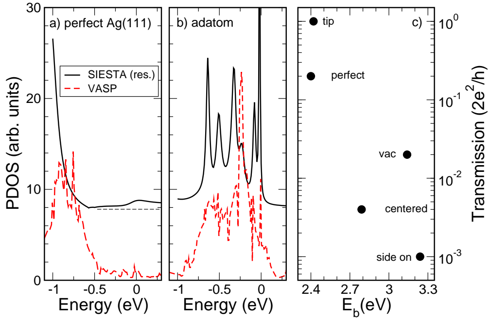
FIG. 5: PDOS of the FDT molecule in between perfect (a) and adatom (b) contacts calculated by both SIESTA (solid line) and VASP (dashed line). For better visibility the SIESTA data were re-scaled (res.) and shifted. c) shows the transmission probability as a function of the binding energy. The transmission for the step configuration has not been calculated.
