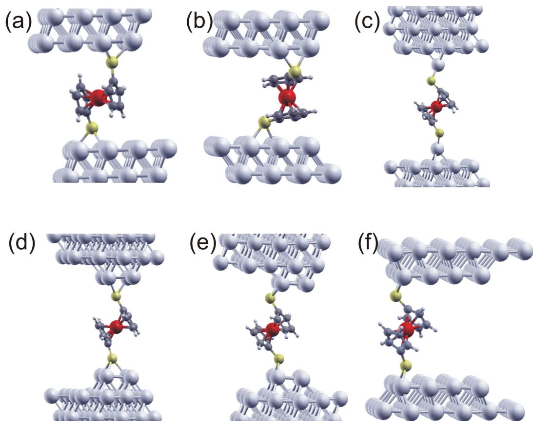
FIG. 1: Optimized structures of FDT between two Ag(111) surfaces: (a) Cp axis parallel to defect-free (111), (b) Cp axis perpendicular to (111). (c) Adsorption on single adatom, (d) centered on 2 \times 2 terraces, (e) side-on the 2 \times 2 structure and (f) at steps. The Ag vacancy structure is not shown.
