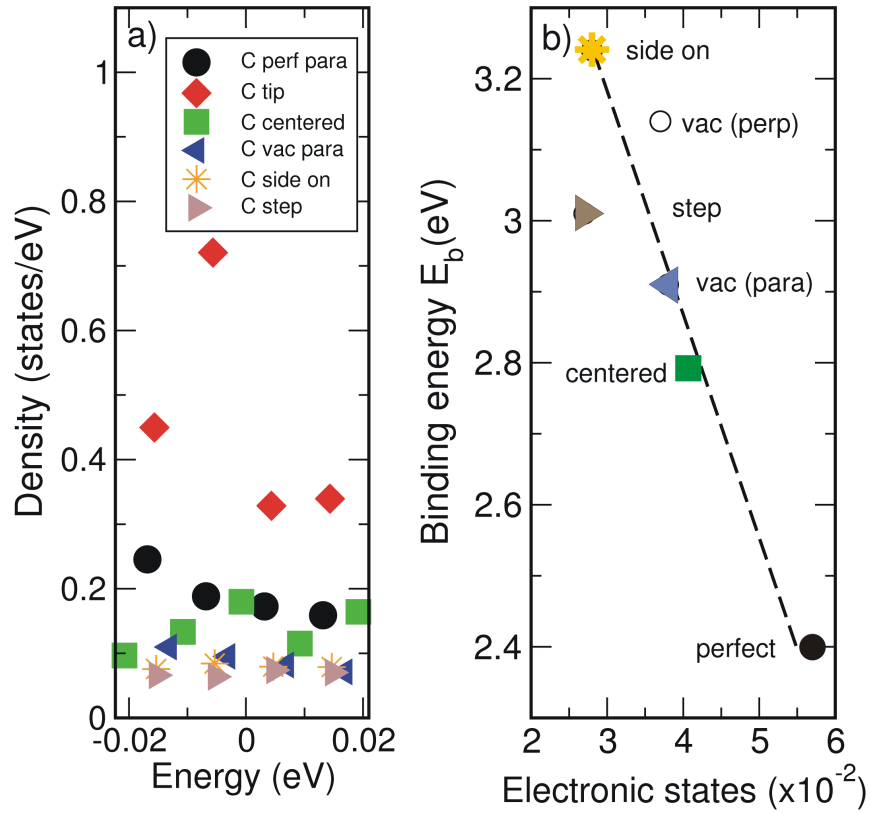
FIG. 4: (a) Density of states, projected onto the Cp rings close to the Fermi energy for the different adsorption configurations listed in Table 1. (b) Correlation between DOS for the different adsorption geometries with a doubly coordinated bond and the binding energy E_b . Here the DOS, obtained with VASP and projected onto the molecule, was integrated over \pm 20 meV around E_F . For better visibility the data point of the tip-configuration states is not shown.
