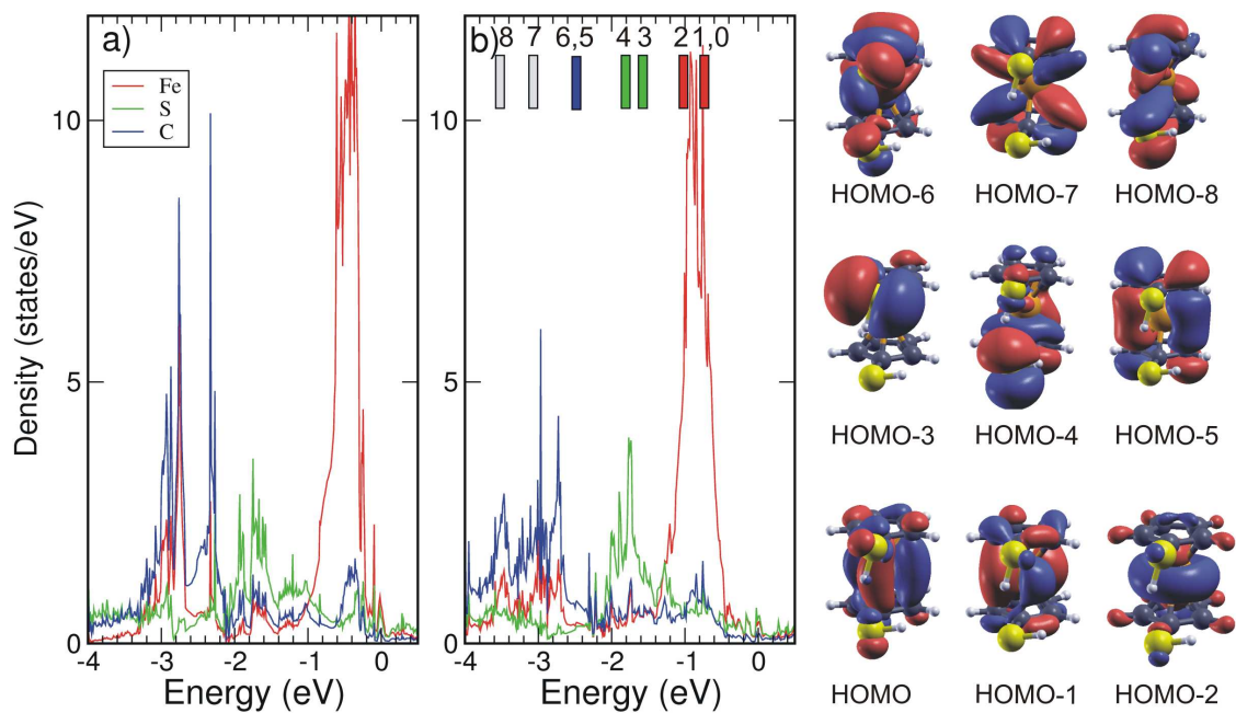
FIG. 2: Projected density of states (DOS) of the energetically optimized configurations of FDT adsorbed between two perfect Ag(111) surfaces. The Cp–Fe–Cp axis is close to the parallel orientation with respect to the Ag(111) surface in (a), perpendicular in (b) (see also Fig. 1a) and b)). The bars in b) show the peak positions of the FDT molecule (not the biradical) in the gas phase after a rigid shift to the topmost state. The numbers at the bars correspond to the occupied Kohn-Sham orbitals. Corresponding isosurfaces are shown on the right.
