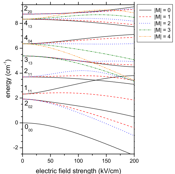
FIG. 2: Stark shift of the lowest rotational lines J_{K-K+} of the v = 0 electronic ground state of \text{SO}_2 . The maximum field strength on the molecular beam axis was about 90 kV/cm, thus well below the crossing of the levels 1_{11} and 2_{11} , M = 0 at about 130 kV/cm.
