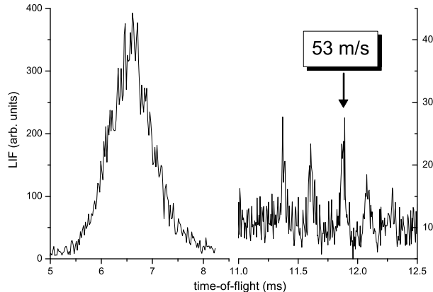
FIG. 4: Time-of-flight spectra of \text{SO}_2 molecules in the rotational state J_{K_-K_+} = 1_{11} , M = 0 . The molecules are decelerated from 285 m/s to 53 m/s (synchronous molecule, arrow) at an phase angle of \phi = 67^\circ and \pm 10 kV.
