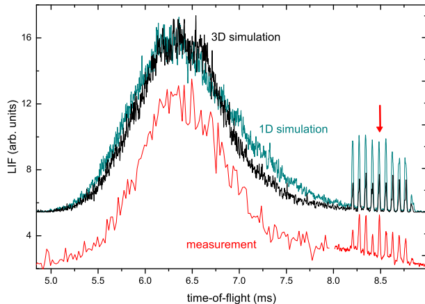
FIG. 3: Measurement (lower curve) and simulations (upper curves) of time-of-flight spectra of \text{SO}_2 molecules in the rotational state J_{K_-K_+} = 1_{11} M = 0 by laser induced fluorescence (LIF). The traces of measurements and simulations are shifted relative to each other for the sake of clarity. The two simulations compare 3D (darker curve) and 1D (lighter curve) trajectory calculations. The molecules are decelerated from 300 m/s to 157 m/s at a phase angle of \phi = 55^\circ . The arrow marks the bunch with the synchronous molecule. The different signal-to-noise ratio in the two parts of the experimental data is due to longer averaging of the part with the decelerated bunches. (Clearly, a 1D simulation is not capable of correctly reproducing the measured intensities.)
