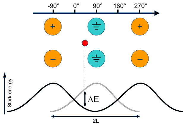
FIG. 1: Schematic of the field configuration and potential energies shortly after switching the electric fields. The electrodes are symbolized by large circles, the polarity is indicated. The smaller circle depicts the synchronous particle. The gray potential curve in the lower part of the figure gives the potential Stark energy before the field configuration is switched, the black curve thereafter. The potential energy loss of the molecule is depicted as \Delta E . The period of the decelerator is twice the stage separation L . At each switching, the potential is shifted by 1/2 of the period. The scale on top shows the position of a particle in the periodic structure of the decelerator in terms of the phase angle \phi . It can be seen that the synchronous particle is located at \phi \approx 50^\circ at the switching time.
