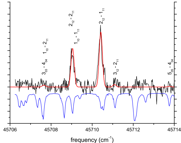
FIG. 5: Measurement of the quantum state distribution behind the decelerator (black curve online) and Monte-Carlo simulation (red) for the main decelerated bunch (10 kV, \phi = 55^\circ ). The inverted curve (blue) shows a reference spectrum before the decelerator with a thermal rotational distribution of about 6.5 K. Quantum numbers of observed and expected transitions are given.
