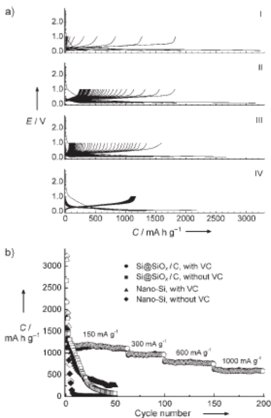
Figure 3. a) Galvanostatic discharge/charge curves (Li insertion, voltage decreases; Li extraction, voltage increases, respectively) of pure Si nanoparticles (I, II) and \text{Si@SiO}_x/\text{C} nanocomposite (III, IV) electrodes cycled at a current density of 150 \text{ mA g}^{-1} between voltage limits of 0.05–1 V in VC-free (I, III) and VC-containing (II, IV) 1 \text{ M LiPF}_6 in EC/DMC solutions. b) Cycling and rate performance of pure Si nanoparticles and \text{Si@SiO}_x/\text{C} nanocomposite electrodes cycled in VC-free and VC-containing 1 \text{ M LiPF}_6 in EC/DMC solutions (solid symbols: charge; empty symbols: discharge.).
