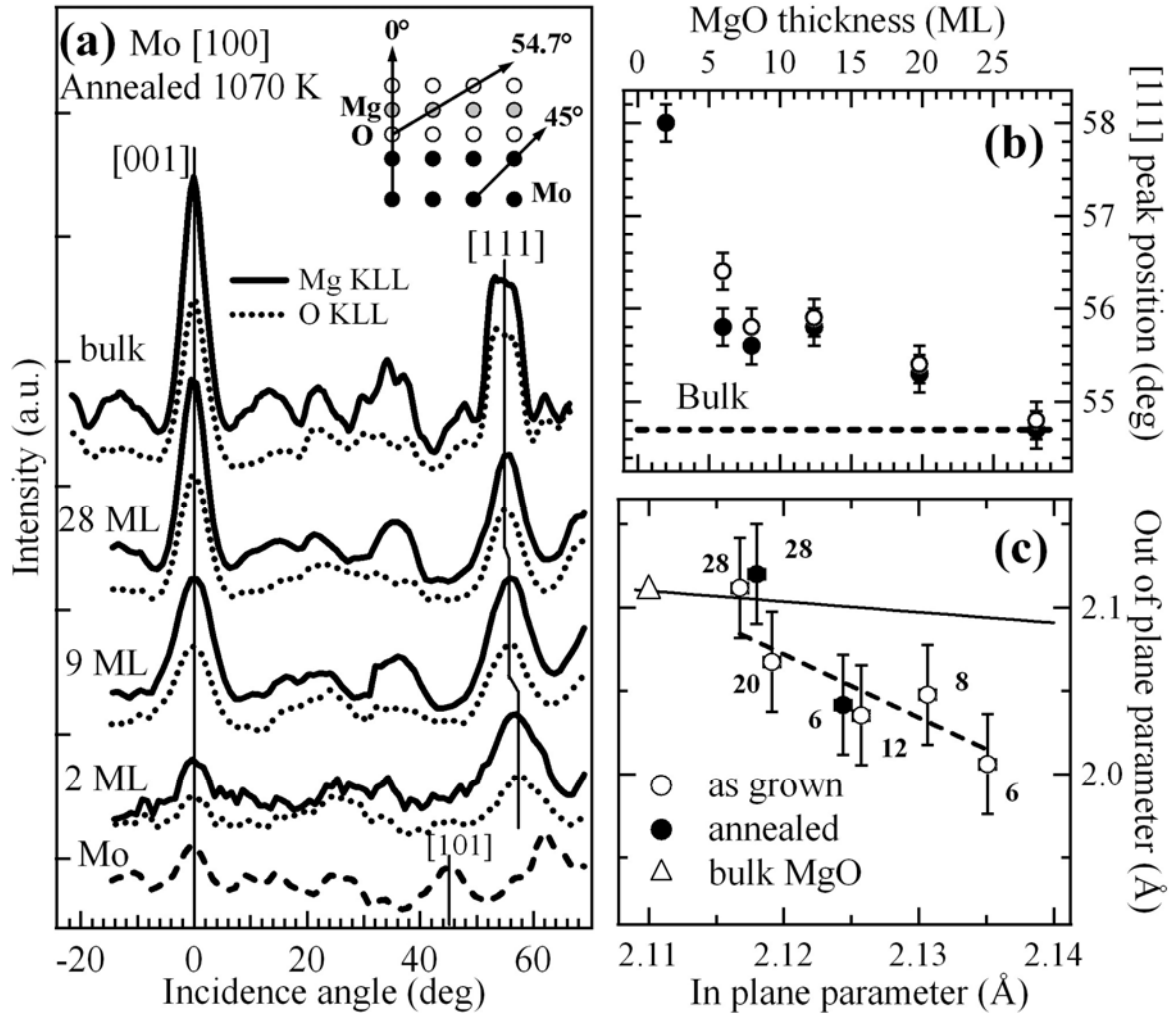
Fig. 2: (a) IADs of Mg KLL (solid line) and O KLL (dotted line) Auger signals along the [100] Mo azimuth for 2-28 ML MgO after annealing at 1070 K. IADs of bulk MgO (top curves) and the Mo MNN IAD of the clean substrate (dashed line) are shown for comparison. Each plot has been scaled to its 0^\circ peak anisotropy. Inset: side view of the rocksalt MgO on the bcc Mo structure cut along the Mo [100]. (b) Angular position of the [111] peak of Mg KLL IAD along the [100] Mo azimuth as a function of MgO thickness for the as-grown (o) and annealed ( \bullet ) samples. (c) Out-of-plane Mg-O distance as a function of in-plane distance obtained by PDMEE and GIXD analysis, respectively. The values for a bulk MgO are shown with an open triangle. The solid line represents the values calculated with the MgO bulk elastic constants ( \gamma = 0.64 , see text for details), while the dashed line indicates the best fit of the experimental data for as grown (o) films ( \gamma = 3.8 ). Numbers next to each point indicate the corresponding MgO thickness in ML.
