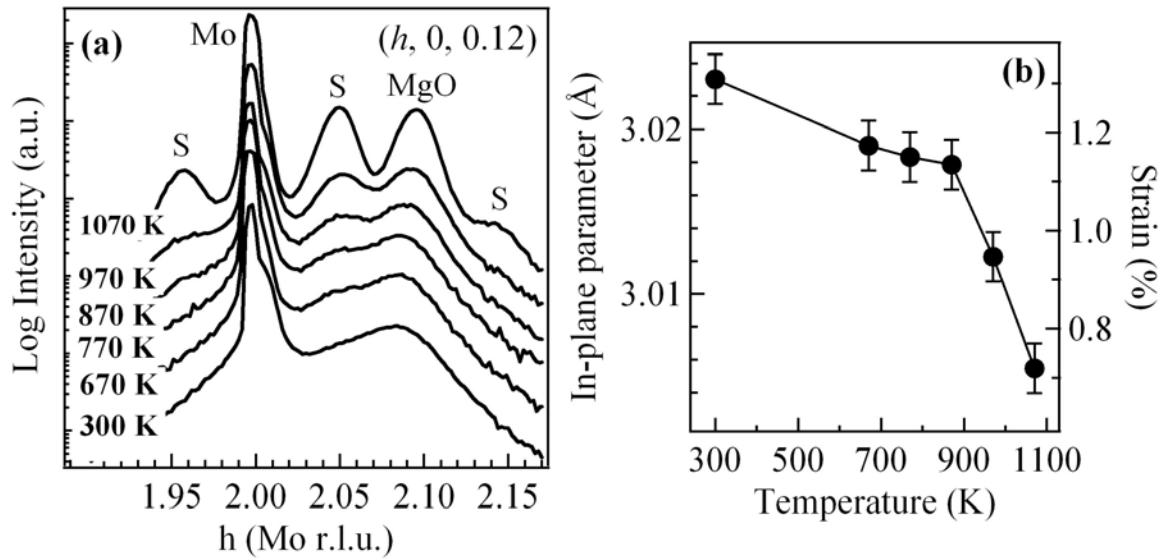
Fig. 6: (a) Radial scans along the (h, 0, 0.12) direction around the (200) Mo Bragg peak for a 7 ML MgO film annealed at increasing temperature. (b) Evolution of the in-plane MgO lattice parameter along the Mo [100] (MgO[110]) direction as a function of annealing temperature.
