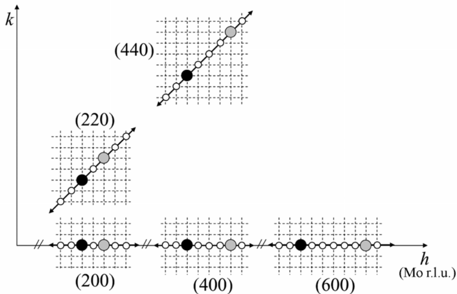
Fig. 7: Schematic representation of the (hk0) plane of the reciprocal lattice of the MgO/Mo(001) interface with an interfacial network of misfit dislocation. Black and grey dots indicate the positions of the Mo and MgO Bragg peaks, respectively. The reciprocal lattice of the dislocation network is represented with dashed lines. White dots represent the location of the satellites as expected for a [110]MgO ([100]Mo) dislocation network.
