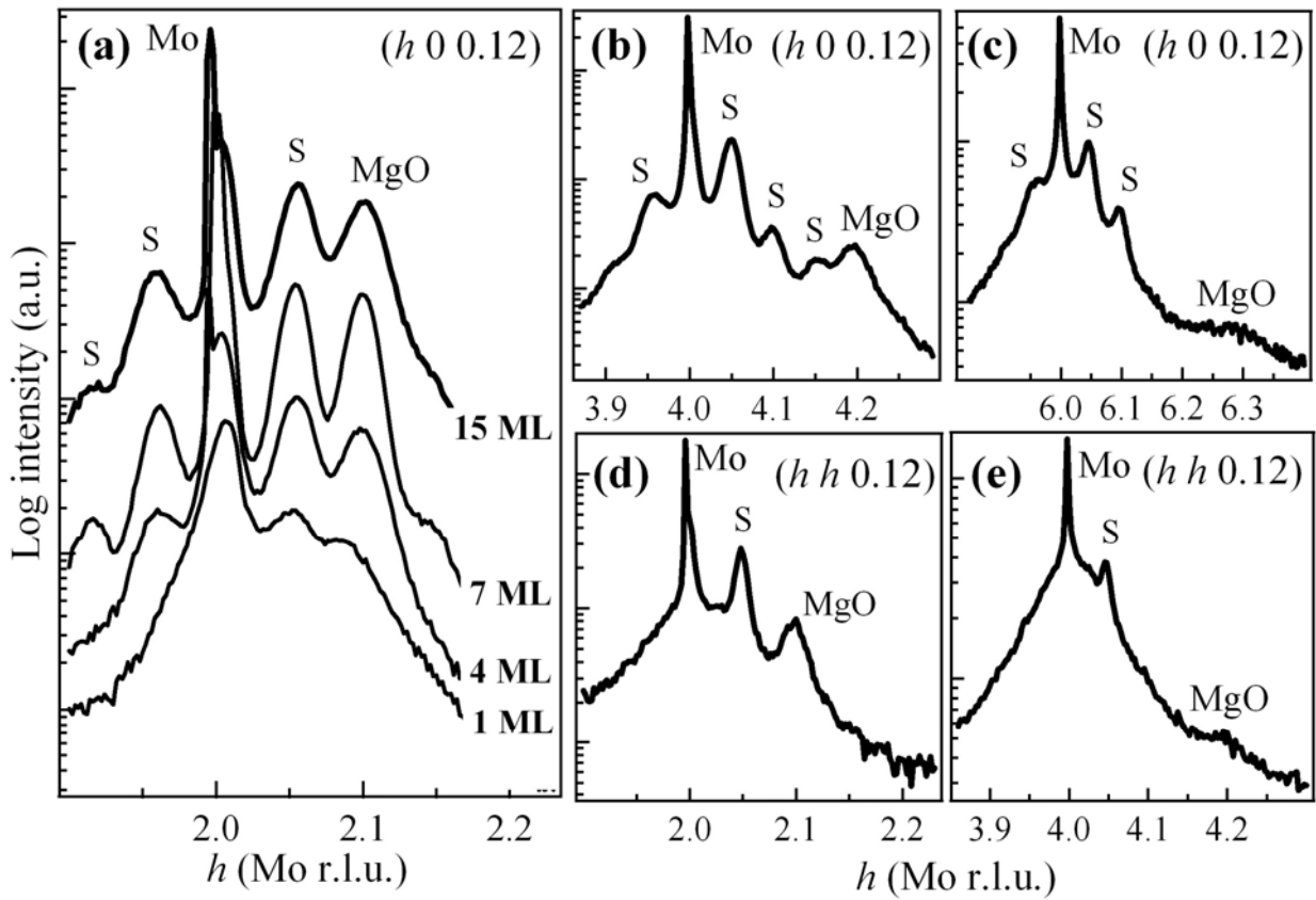
Fig. 5: (a) Radial scans along the (h, 0, 0.12) direction around the (200) Mo Bragg peak for MgO films of increasing thickness annealed at 1070 K. (b-e) Radial scans on a 15 ML MgO film on Mo(001) annealed at 1070 K. Diffraction satellites due to the interfacial dislocation network are indicated with a “S”. The l value of 0.12 has been chosen to maximize the satellite/bulk relative contributions.
