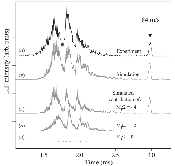
FIG. 3: A measured time-of-flight (TOF) profile of metastable \text{NH} molecules observed in a deceleration experiment (a), compared with the outcome of a numerical simulation (b). The molecules are decelerated from 520 m/s to a final velocity of 84 m/s. The contribution of individual M_J\Omega components to the simulated TOF-profile is shown in the lower part of the figure.
