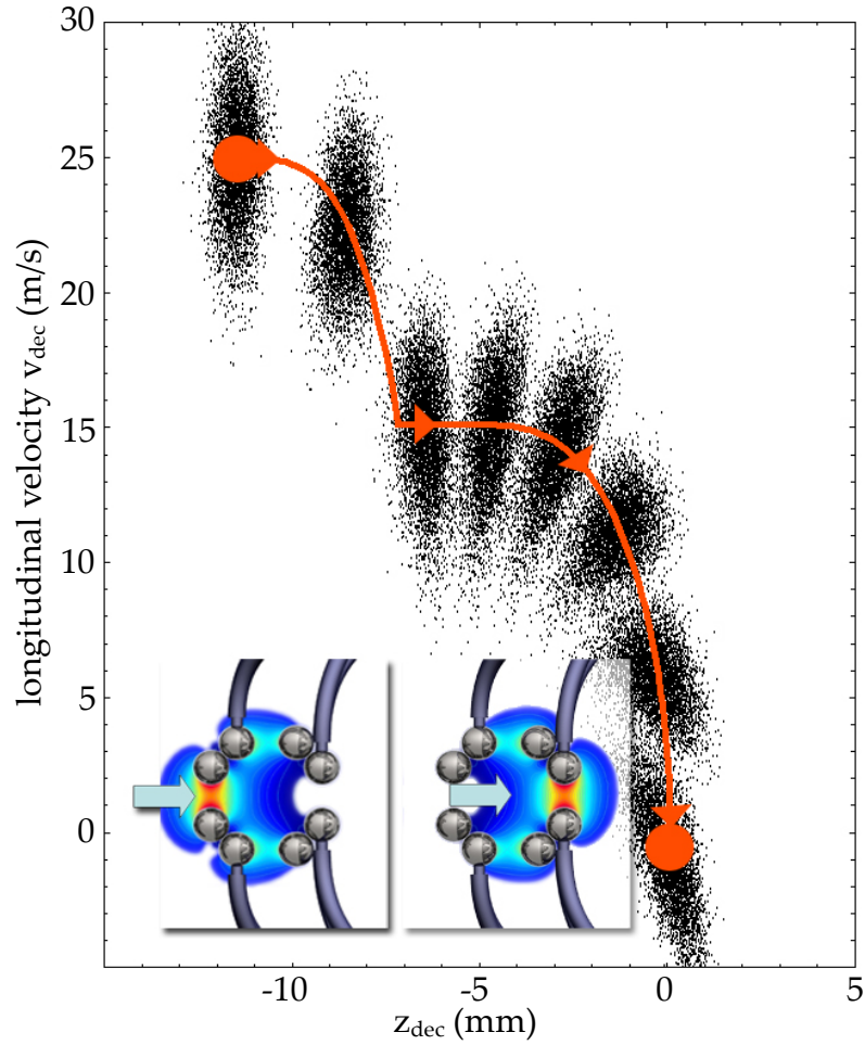
FIG. 7: (color online.) Snapshots in time of the phase-space distribution along the molecular beam axis for deceleration and loading. The individual snapshots are separated by equal time intervals of 100 \mu\text{s} . The two different processes can be nicely distinguished. The initial molecular packet leaving the decelerator and entering the trap has a mean velocity of 25 \text{ m/s} and a velocity spread of \pm 7 \text{ m/s} (FWHM). Its position is 12 \text{ mm} away from the trap center, the position spread is \pm 1 \text{ mm} (FWHM). The motion of the synchronous molecule is indicated by the orange line.
