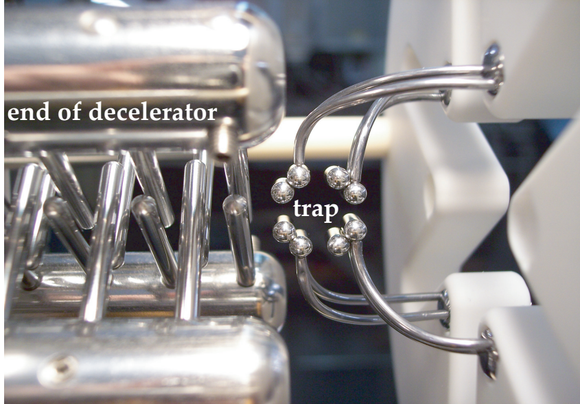
FIG. 1: A picture of the very open linear AC trap combined with the Stark decelerator. The trap is held by bent tantalum wires which are suspended from a ceramic plate.
