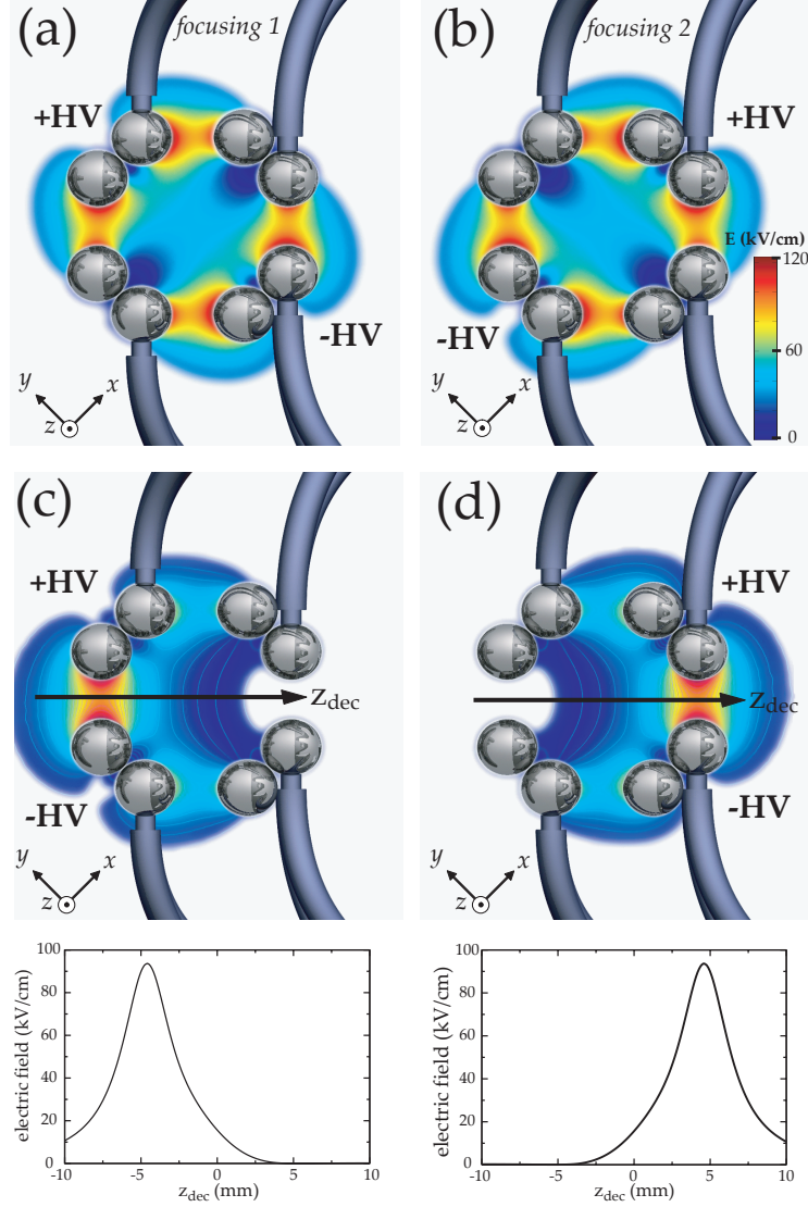
FIG. 2: (Color online.) The four different electric field configurations of the AC trap used in the course of an experiment. Parts (a) and (b) show the two different saddle point configurations ( focusing 1 and focusing 2 ) of the linear AC trap. Trapping in the third dimension along the z -axis is due to fringe field effects of the electric field strength. (c) The electric field strength corresponding to the deceleration stage of the trap. The left electrode pair is energized with high voltages of up to \pm 10 kV while the right pair is grounded. The electric field strength along the molecular beam axis z_{dec} is given below. The trap center is at z_{dec} = 0 mm. This configuration can also be used to load molecules in hfs states into the trap. (d) The loading configuration. The left electrode pair is grounded, while the right one is energized (up to \pm 10 kV). The electric field strength along the molecular beam axis z_{dec} is displayed below. The color scale indicator in part (b) also applies to the electric field configurations shown in (a) and (c)-(d).
