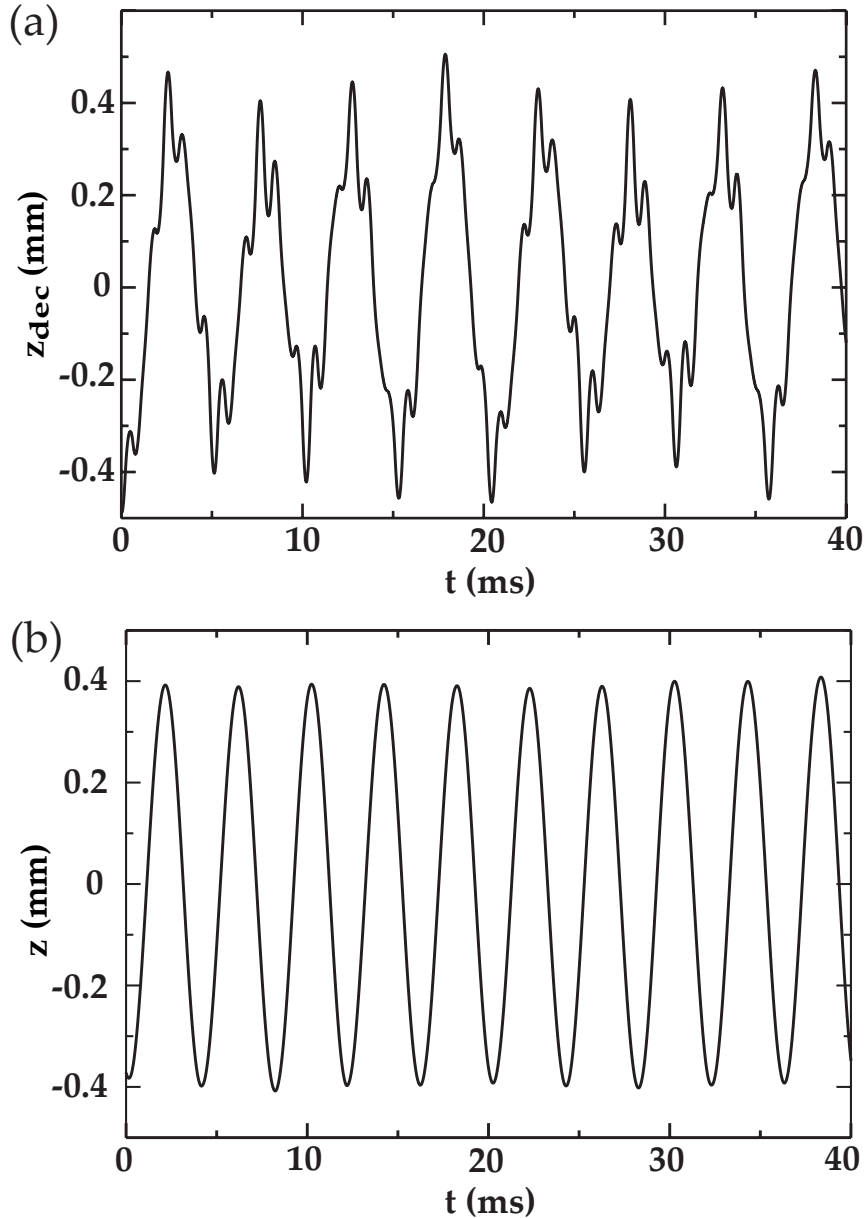
FIG. 4: Trajectory of an ammonia molecule ( ^{15}\text{ND}_3 ) along the molecular beam axis z_{dec} (a) and along the z-axis of the trap (b) as a function of time. The switching frequency is 1150 Hz.
