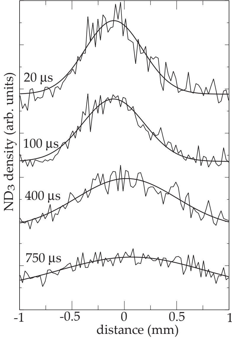
FIG. 10: Spatial distributions of ^{15}\text{ND}_3 molecules in hfs states after expansion for the time indicated in the figure. The molecules are released from the trap after 60 switching cycles with a trapping frequency of 1150 Hz (trap voltage: \pm 6.6 kV). The bold lines show Gaussian fits to the distribution.
