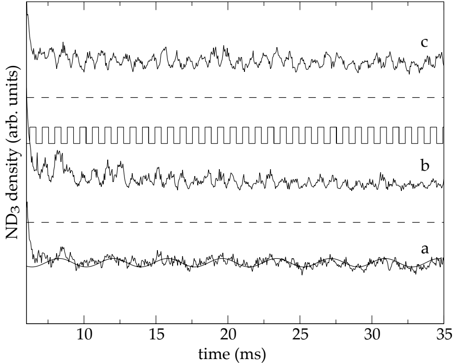
FIG. 9: Evolution of the density of trapped \text{ND}_3 molecules in hfs states as a function of trapping time measured at different positions inside the trap. The dashed lines indicate the zero signal for curves b and c ; zero signal for curve a is the baseline of the figure. For the measurements displayed in curve a the detection laser was located 0.3 mm above the trap center, while for curves b and c it was 0.3 mm above the trap center and, in addition, shifted by \pm 0.23 mm along the molecular beam axis z_{dec} . Switching of the AC trap is indicated as well. The oscillations in curves b and c follow the switching frequency of the trap, but with opposite phase. They are modulated by an additional, slower oscillation of 260 Hz (see text for details). In curve a the amplitude of the fast oscillation is significantly reduced. The 260 Hz oscillation is more pronounced.
