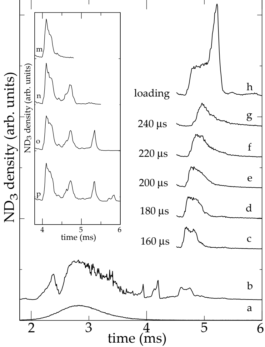
FIG. 6: Time-of-flight (TOF) spectra characterizing the deceleration and loading process. The detection laser is located in the trap center and is tuned to a REMPI-frequency resonant for molecules in lfs states. Curve a shows the Gaussian type distribution of the original beam when no fields are turned on. Curve b was obtained with only the decelerator turned on, resulting in a packet of molecules slowed down to 25 m/s (TOF of 4.7 ms). For curves c-g the deceleration stage of the trap has been turned on for different time intervals, indicated in the figure. Curve h displays the strong focusing effect which is obtained when, in addition to the trap deceleration field (on for 200 \mu s), also the loading field is turned on, for 690 \mu s. The voltages applied to the decelerator and trap electrodes are \pm 10 kV, respectively. The inset shows the TOF spectra for reflection experiments with ^{15}\text{ND}_3 molecules in lfs states using the deceleration and loading fields of the trap (see text). For all curves, the measured signal is zero for larger times approaching 6 ms.
