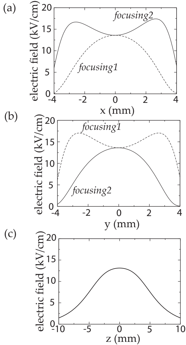
FIG. 3: The electric field for the two focusing configurations in x-, y-, and z-direction. The electric field in z-direction is the same for the two configurations.
