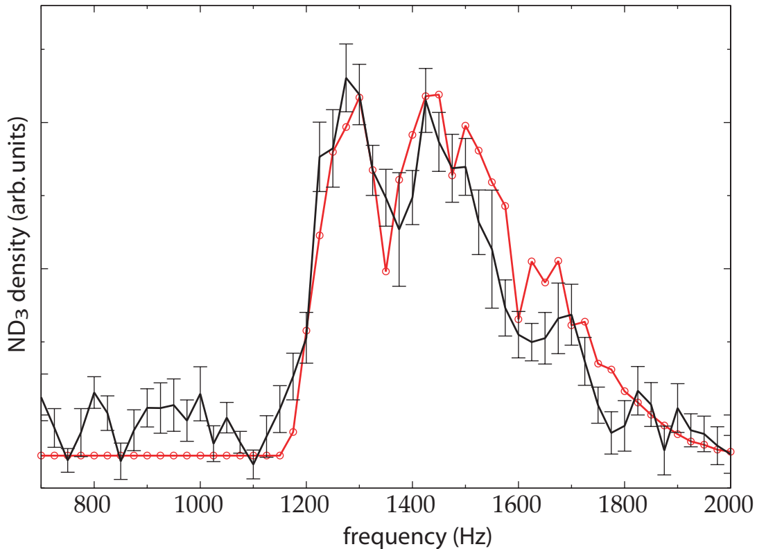
FIG. 8: Frequency dependence of the density of trapped \text{ND}_3 molecules in hfs states for trapping voltages of \pm 10 kV, after the molecules have been stored in the trap for about 60 ms. Both experimental results (with error bars) and simulations (open circles) are shown. The baseline of the figure indicates zero signal.
