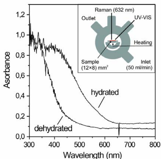
Figure 1: UV-Vis spectra of hydrated and dehydrated V/SBA-15. The inset shows a cross-sectional scheme of the experimental setup illustrating the UV-Vis and Raman capabilities.
