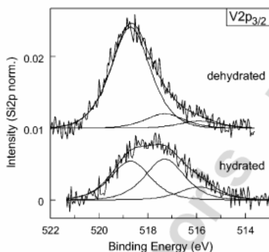
Figure 3: XPS V2p_{3/2} spectra of hydrated (bottom) and dehydrated (top) V/SBA-15 together with the results of the fit analysis. The spectra are offset for clarity. For details see text.
