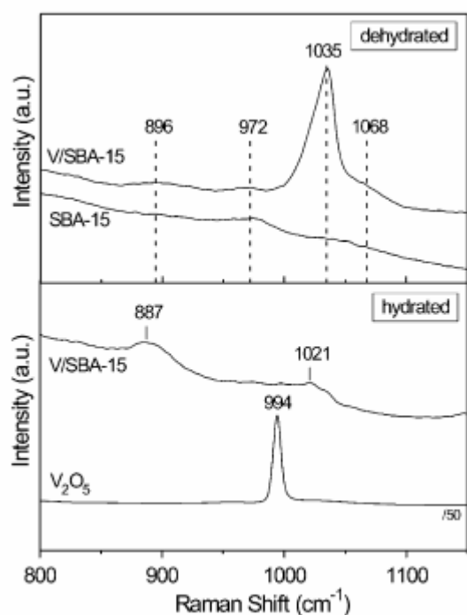
Figure 2: Top panel: Raman spectra of dehydrated V/SBA-15 (top) and bare SBA-15 (bottom). Bottom panel: Raman spectra of hydrated V/SBA-15 (top) and V_2O_5 (bottom). The spectra are offset for clarity.
