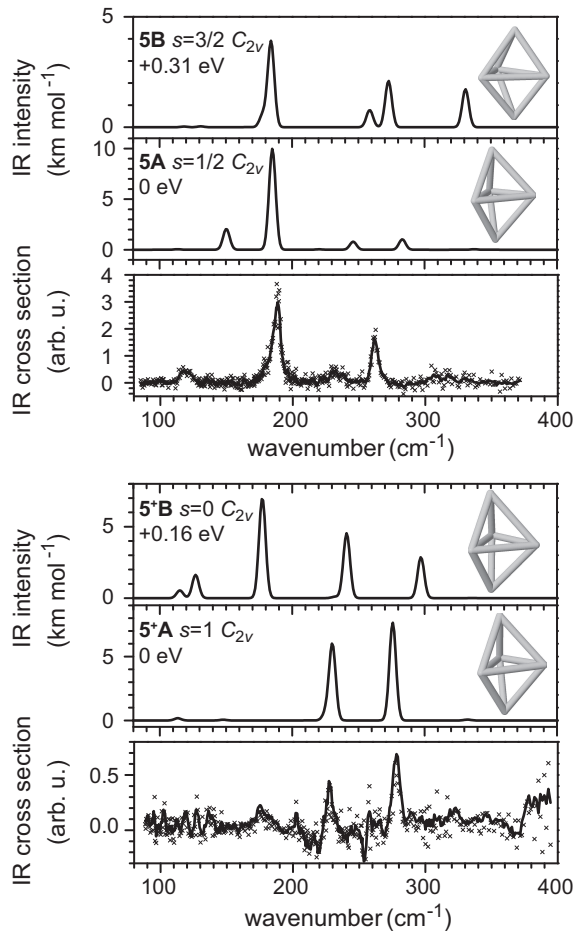
FIG. 2: Vibrational spectra of \text{Nb}_5 (upper panel) and \text{Nb}_5^+ (lower panel). The bottom traces in each panel show the experimental multiple photon dissociation spectra of the corresponding complexes with Ar atoms. They are compared with the calculated vibrational spectra for energetically low-lying isomers. The calculated stick spectra are folded with a Gaussian line width function of 5 \text{ cm}^{-1} full width at half maximum for ease of comparison. The experimental data points are overlaid with a five-point running average to guide the eye.
