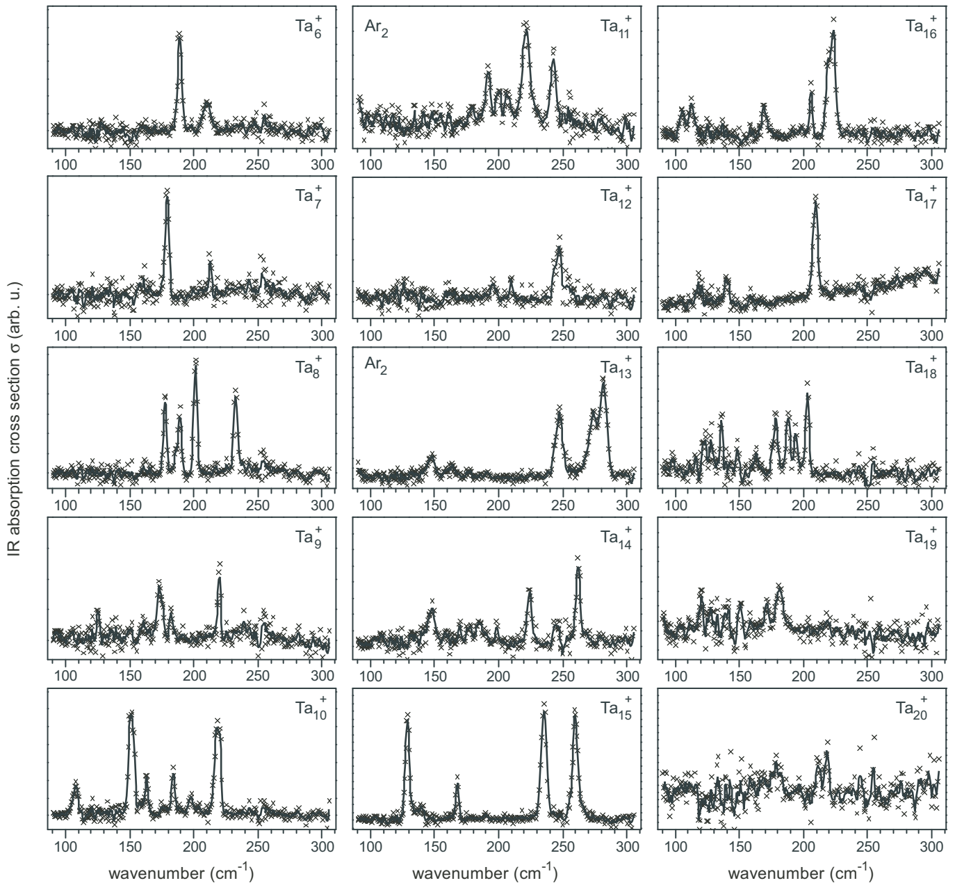
FIG. 3: Far-infrared multiple photon dissociation spectra of Ta_nAr^+ ( n = 6 - 20 ). The gray crosses represent the raw data while the black line interconnects the adjacent three point average of the raw data points. In case of Ta_{11}^+ and Ta_{13}^+ the spectra are obtained upon IR-MPD of their complexes with two argon atoms.
