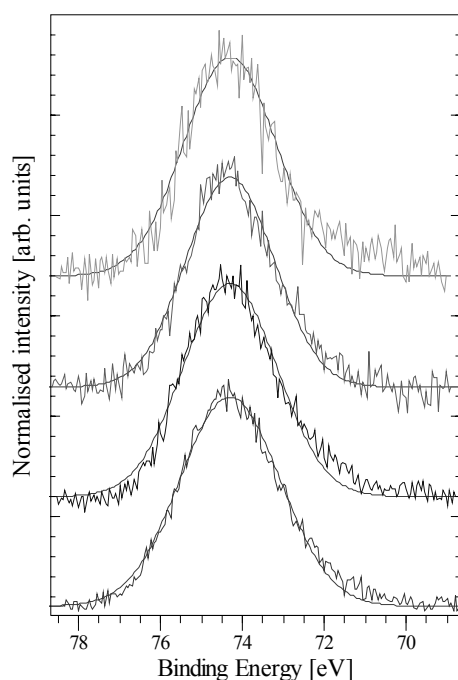
Figure 8: Al 2p peak at analysis depths of a) 10 Å, b) 14 Å, c) 17 Å and d) 21 Å in sample HT under reaction conditions.
