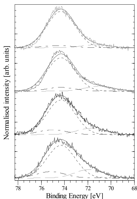
Figure 10: Al 2p peak together with Pt 4f doublet in the samples Pt-2 and Pt-1 at 10 Å analysis depth. a) Pt-2 in reaction mixture, b) Pt-2 in oxygen, c) Pt-2 in hydrogen-steam mixture and d) Pt-1 in reaction mixture, all at 450°C.
