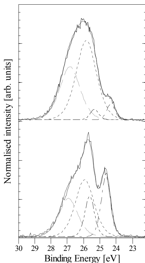
Figure 17: Deconvolution of Sn 4d peak in PtSn 2 alloy at 15 Å analysis depth under following conditions: a) in H 2 at 450°C and b) in reaction mixture at 450°C.
