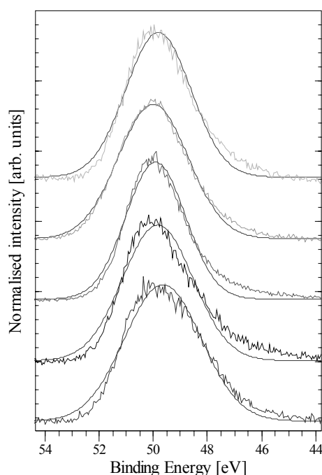
Figure 7.: The Mg 2p peak in samples Pt-2, HT and Pt-1 at 10 Å analysis depth. a) Pt-2 in reaction mixture, b) Pt-2 in oxygen, c) Pt-2 in hydrogen-steam mixture, d) HT in reaction mixture, e) Pt-1 in reaction mixture, all at 450°C.
