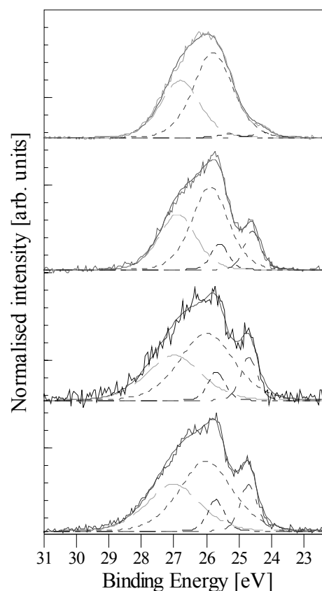
Figure 16: Deconvolution of Sn 4d peak in PtSn 2 alloy at 8 Å analysis depth under following conditions: a) in UHV at RT, b) in H 2 at RT, c) in H 2 at 450°C and d) in reaction mixture at 450°C.
