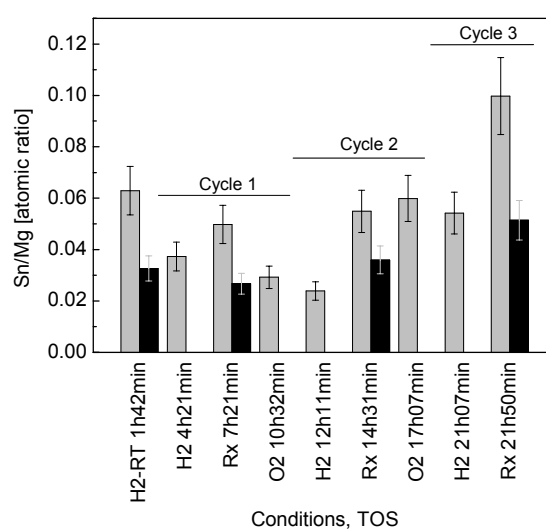
Figure 11: Sn/Mg atomic ratio in sample Pt,Sn-1 at 10 Å (grey bars) and 14 Å (black bars) analysis depth.
