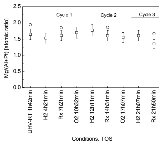
Figure 13: Mg/(Al+Pt) atomic ratio in sample Pt,Sn-1 at 10 Å (▽) and 14 Å (◻) analysis depth.
