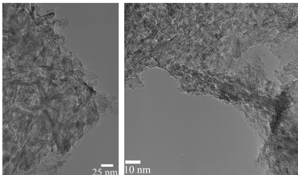
Figure 1: TEM pictures of a) Sample HT and b) Sample Pt-2.
