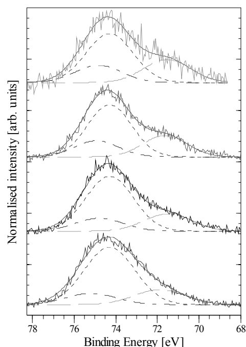
Figure 9: Al 2p peak together with Pt 4f doublet in the sample Pt-2 under reaction conditions at analysis depths of a) 10 Å, b) 14 Å, c) 17 Å and d) 21 Å.
