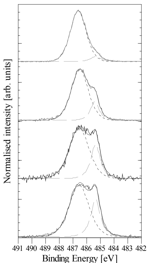
Figure 15: Deconvolution of Sn 3d peak in PtSn 2 alloy at 8 Å analysis depth under following conditions: a) in UHV at RT, b) in H 2 at RT, c) in H 2 at 450°C and d) in reaction mixture at 450°C.
