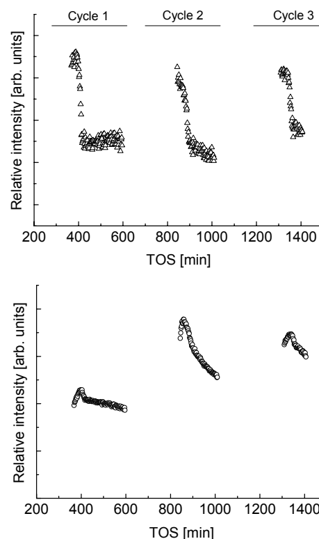
Figure 4: Activation of sample Pt,Sn-1 during in situ XPS measurements under reaction conditions at 450°C. H 2 :C 2 H 6 :H 2 O = 1 : 1.5 : 7.5, total pressure 0.3 mbar. Upper curve: [(m/e 28) : (m/e 30)], representing ethene production. Lower curve: [(m/e 44) : (m/e 30)], representing CO 2 production.
