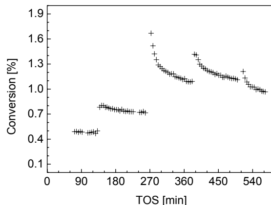
Figure 3: Activation of sample Pt,Sn-1 in a conventional test reactor at 450°C. Reaction conditions: H 2 :C 2 H 6 :CO 2 :Inert = 1:6.3:4.3:51, 450°C, 1 atm, WHSV = 1.6 h -1 .
