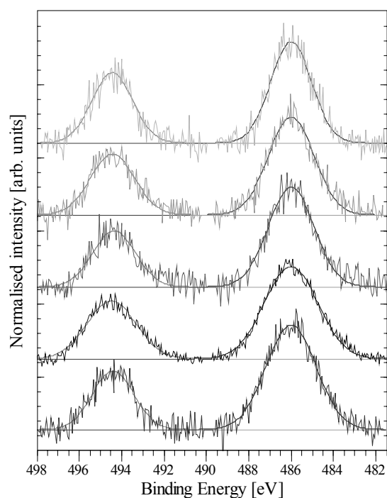
Figure 12: Sn 3d doublet in sample Pt,Sn-1 at two analysis depths and in different gas mixtures, a) 10 Å, H 2 , room temperature b) 10 Å, O 2 , 450°C c) 10 Å, H 2 450°C, d) 10 Å, reaction mixture, 450°C e) 14 Å, reaction mixture 450°C.
