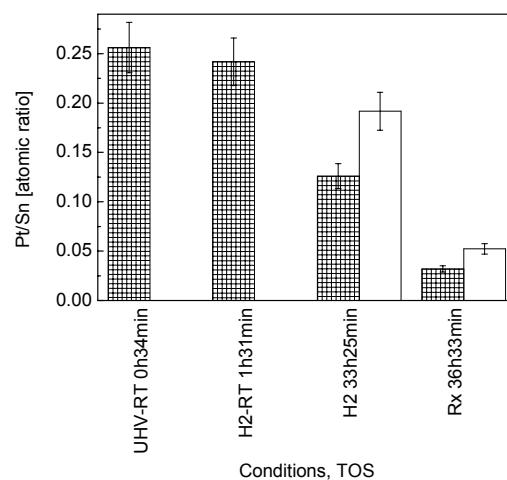
Figure 14: Pt/Sn atomic ratio in PtSn 2 alloy under different conditions (see Table 1 for details) and at two analysis depths: 8 Å (squared bars) and 15 Å (white bars).
