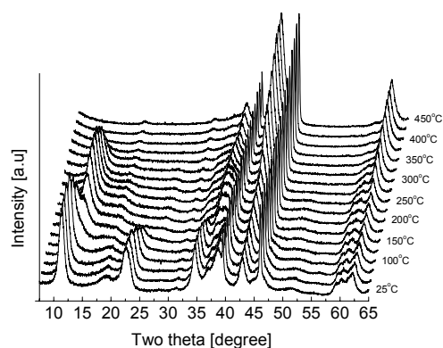
Figure 2: Temperature resolved XRD-patterns of a Mg(Al)O sample after storage in air for several months, during heating to 450°C in air. The reflexes at 2\theta = 39.5^\circ and 46.0^\circ are Pt reflexes from the Pt sample holder.
