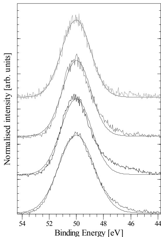
Figure 6: The Mg 2p peak at analysis depth of a) 10 Å, b) 14 Å, c) 17 Å and d) 21 Å in calcined hydrotalcite (sample HT) under reaction mixture at 450°C.
