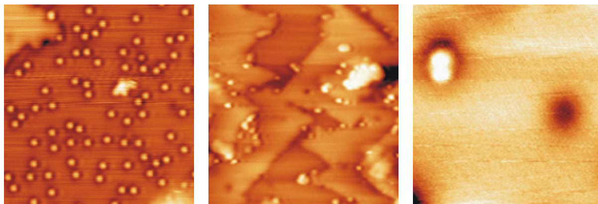
Fig. 3 Low-temperature (5K) STM images of gold atoms on 4 ML MgO(001)/Ag(001): a) Au deposition at 5 K (20x20 nm 2 ). b) Au deposition at 80 K (20x20 nm 2 ). c) Au deposition at 5 K, nucleation on defect (5x5 nm 2 ).
