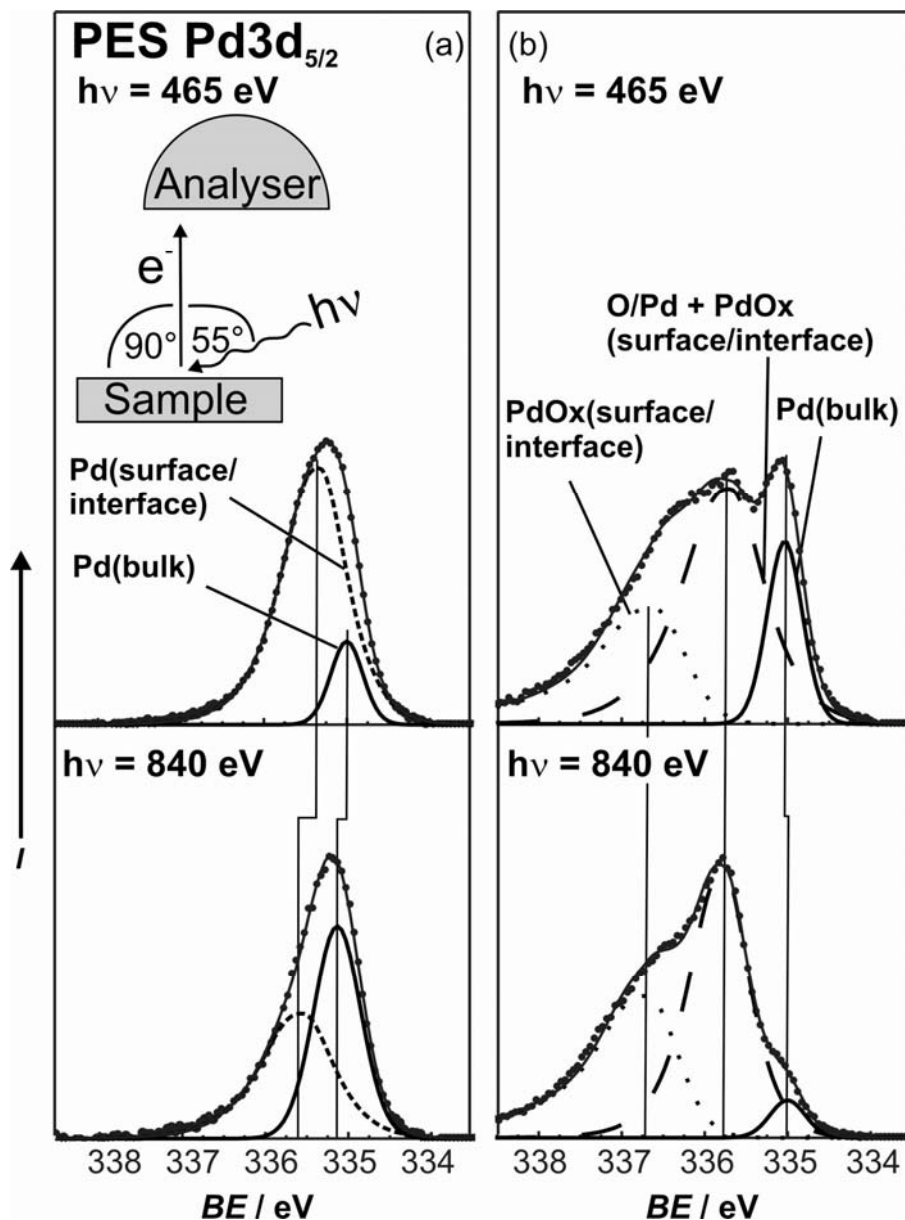
Fig. 7 High resolution core level spectra of Pd 3d_{5/2} region after preparation of the model catalyst at different photon energies: (a) immediately after Pd deposition and annealing in UHV to 600 K; (b) after oxygen exposure at 600 K (oxygen dose: 800 L).
