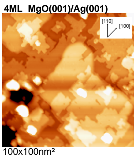
Fig. 1 (a) Scanning tunneling microscopy (STM) of an MgO(100) film grown on Ag(100) and imaged at 4 K
