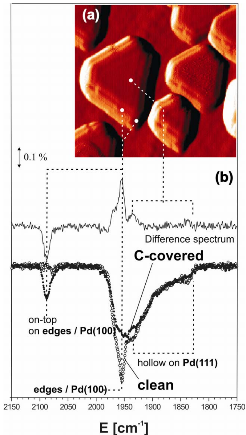
Fig. 5 (a) STM image of the Pd particles grown at 300 K on \text{Al}_2\text{O}_3/\text{NiAl}(110) ( 20 \times 20 nm). (b) RAIR spectra for CO adsorbed on Pd/ \text{Al}_2\text{O}_3/\text{NiAl}(110) taken at a sample temperature of 100 K after CO exposure at 300 K ( \sim 20 L). Open symbols: immediately after preparation; solid symbols: after extended exposure to methanol at 440 K (7000 L); solid line: difference spectrum for the two situations.
