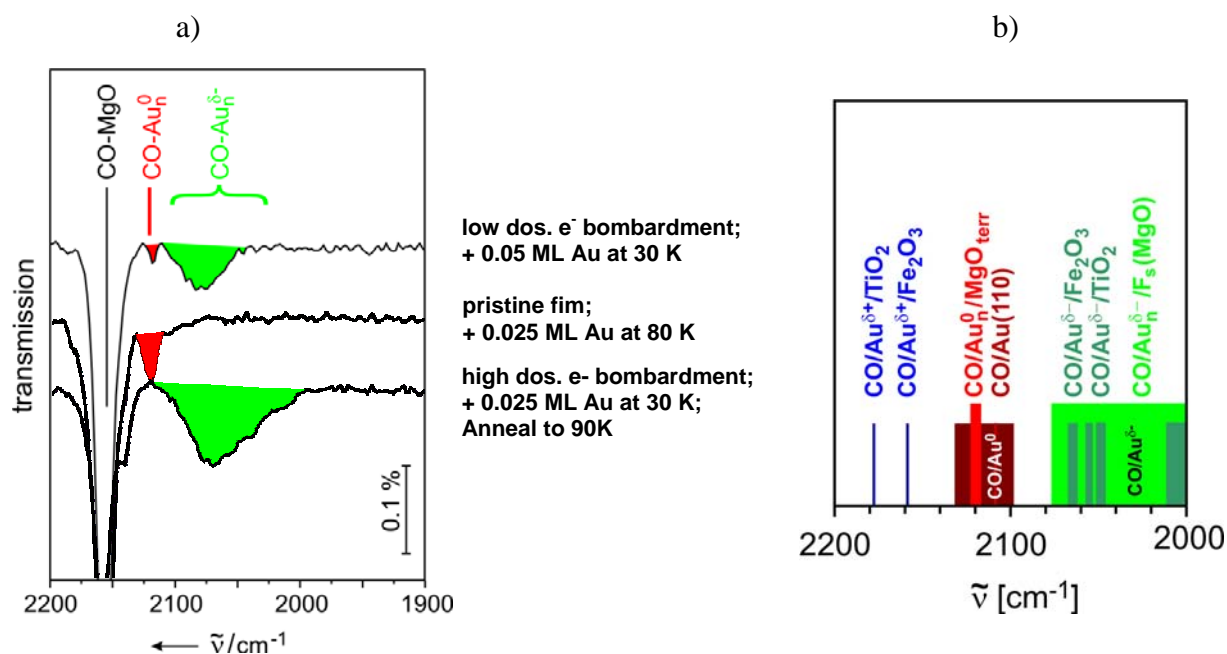
Fig. 4 (a) IR spectra of 1 L CO adsorbed at 30 K on Au deposits (b) comparison of the stretching frequencies from a with data reported in the literature for Au catalysts [27]
