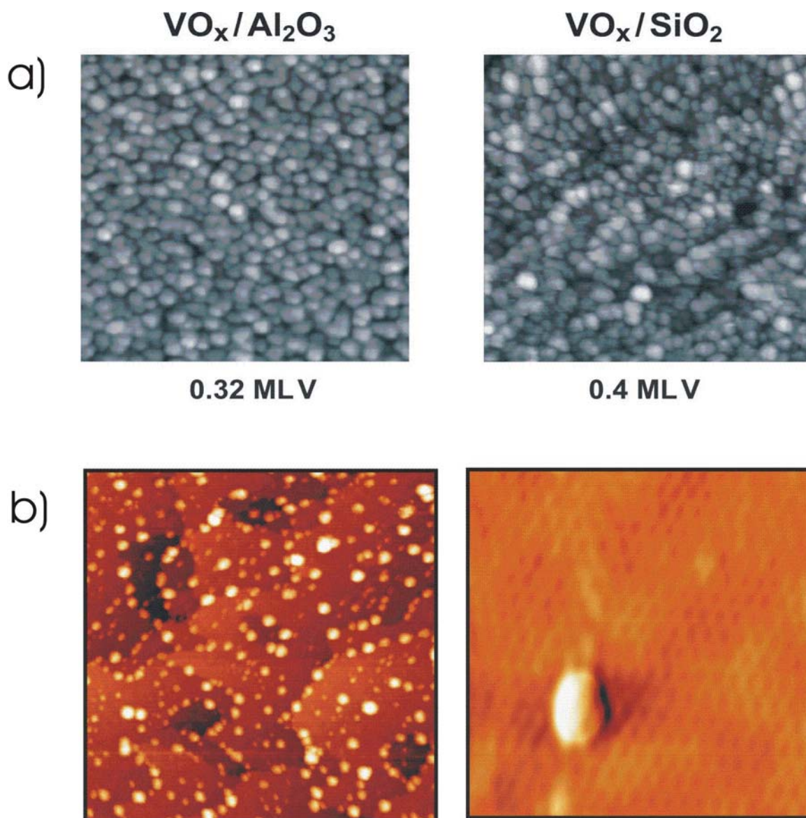
Fig. 9: a) Comparison of two STM images (50 nm x 50 nm) measured for alumina- and silica-supported vanadia particles of similar V-content. Tunneling was performed at the following conditions: U=2.2 V, I=0.07 nA ( \text{VO}_x/\text{Al}_2\text{O}_3 ); U=3.3 V, I=0.12 nA ( \text{VO}_x/\text{SiO}_2 ). In both cases, particle number densities between \sim 1.8 - 1.9 \times 10^{13} particles per \text{cm}^{-2} were determined. b) STM images of \text{VO}_x/\text{SiO}_2 at lower \text{VO}_x coverage. The right panel shows a single \text{VO}_x cluster on the atomically resolved \text{SiO}_2 substrate.
