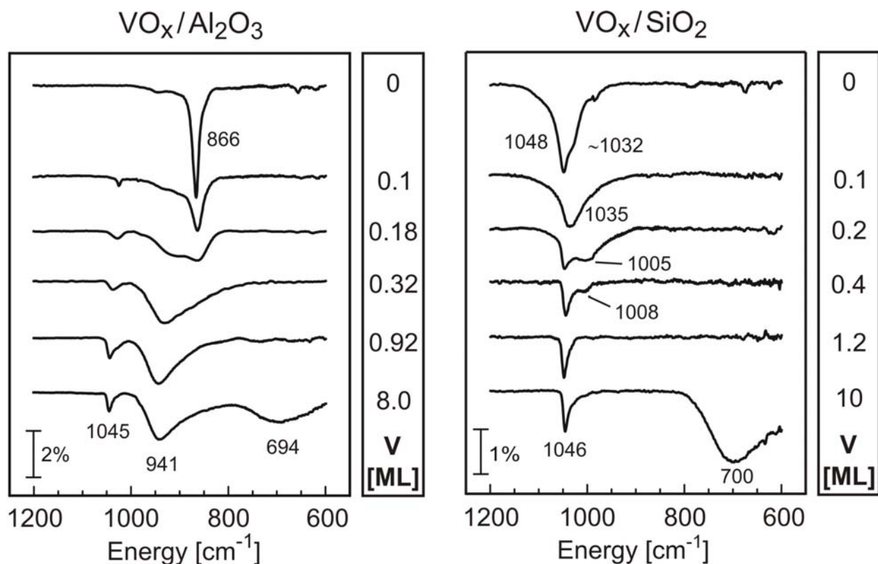
Fig. 10 IR spectra from alumina- and silica-supported vanadia particles as a function of V-coverage. All spectra were measured at 300 K and referenced to the underlying NiAl and Mo metal substrates, respectively.
