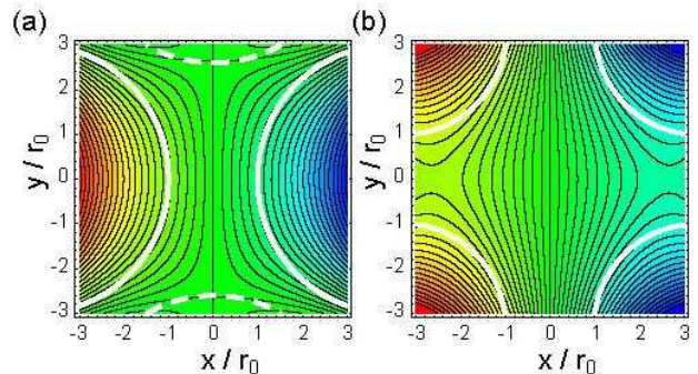
FIG. 3: Electrostatic equipotentials of equation (8) for the cases (a) a_3/a_1 = +1/7 , a_5 = 0 and (b) a_3/a_1 = -1/7 , a_5 = 0 . Red and blue colourings correspond to positive and negative potentials respectively. The white lines show electrode surfaces designed to follow these contours.
