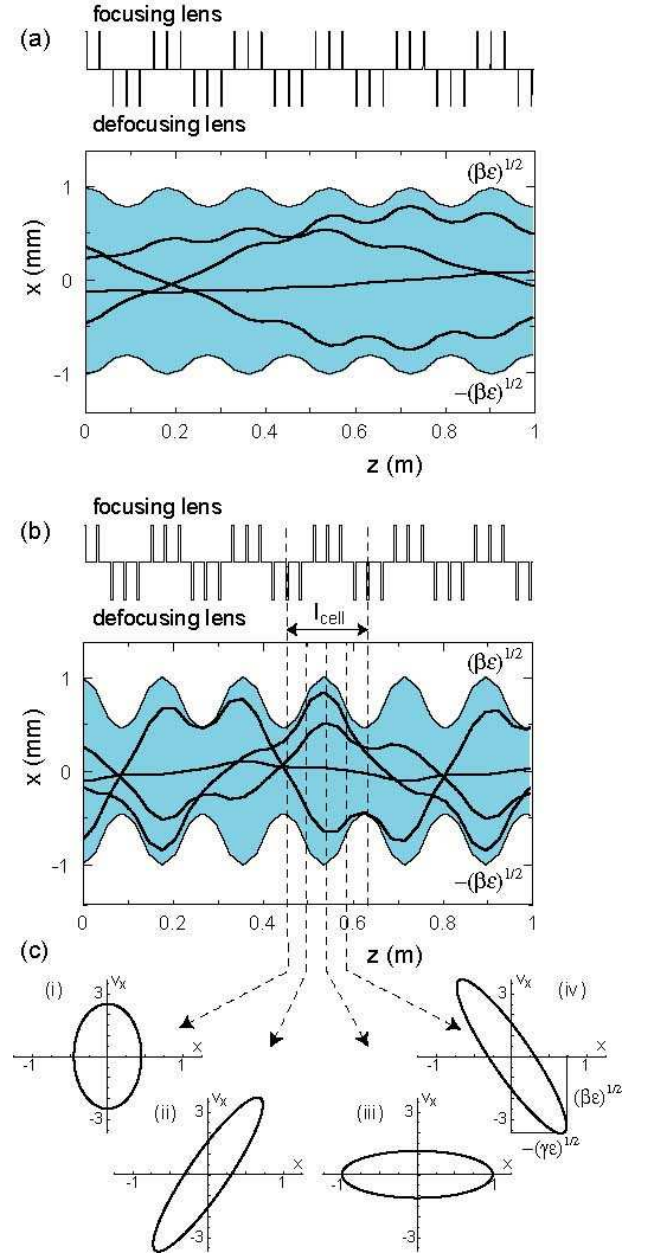
FIG. 6: (a) Trajectories of metastable CO molecules flying with a forward speed of 315 m/s through a (FO)^3(DO)^3 array. The parameters are \kappa=38.7 \text{ m}^{-1} , L=2 \text{ mm} and S=28 \text{ mm} , corresponding to \Phi = \pi/6 . The shaded area shows the beam envelope bounded by \pm\sqrt{\beta\epsilon} , for a constant aperture of d=2 \text{ mm} . (b) As (a), but with L=6 \text{ mm} and S=24 \text{ mm} corresponding to \Phi = \pi/2 . (c) Phase-space area occupied by the beam at four positions in the unit cell with the position spread in mm and the velocity in m/s. (i) Centre of the defocusing set, (ii) between the defocusing and focusing sets, (iii) centre of the focusing set and (iv) between the focusing and defocusing sets.
