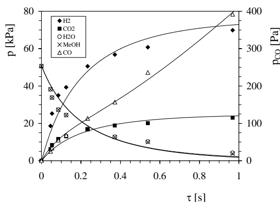
Figure 9: Partial pressures of the components in the reaction mixture during SRM on CZC15, experimental data and fitting results m = 0.6726 g, T = 543 K, p = 10^5 Pa, MeOH:H 2 O = 1:1
