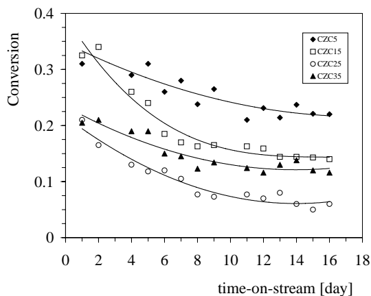
Figure 3: Methanol conversions during SRM of four CZC catalysts as a function of time-on-stream ( m_{\text{CuO}} = 0.0225 g, T = 523 K, p = 10^5 Pa, w = 0.07 cm 3 min -1 , MeOH:H 2 O = 1:1)
