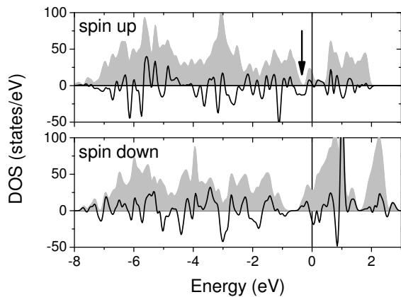
FIG. 4: Total density of states (DOS) of \text{Fe}_3\text{O}_4(001) terminated by a modified B-layer for the majority (minority) spin channel in the upper (lower) panel is shown in grey. The difference of the DOS of the modified B-termination and the bulk-terminated B-layer is given with a black line. A Gauss broadening of 2\sigma = 0.05 eV is used.
