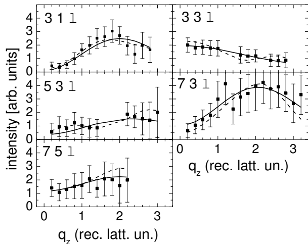
FIG. 3: Results of the XRD-analysis. The experimental data is marked by squares. Solid and dashed lines correspond to fits assuming the modified B-termination and 0.5 ML Fe A -termination, respectively.
