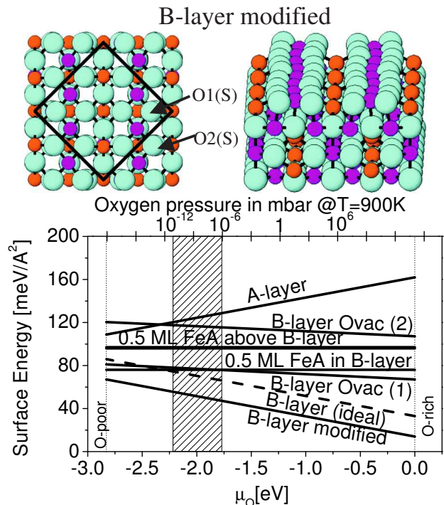
FIG. 2: Calculated surface free energy \gamma(T, p) as a function of the chemical potential of oxygen (bottom x -axis) for all studied terminations. In the top x -axis the \mu_{\text{O}} is converted into a pressure scale at T = 900 K. The vertical lines mark the oxygen-poor and oxygen-rich limits of the oxygen chemical potential, with 1/2E_{\text{O}_2}^{\text{total}} used as zero reference. The dashed region marks the range of pressures that were used during sample preparation in the experiment. The B-termination with bulk atomic positions and modified positions with a (\sqrt{2} \times \sqrt{2})R45^\circ -periodicity are marked as ideal and modified, respectively. The B-layer with oxygen vacancies above an octahedral iron and next to a tetrahedral iron are denoted by (1) and (2), respectively. Top and side view of the modified B-layer is given at the top. Surface oxygens with and without a \text{Fe}_A neighbor are denoted by O2(S) and O1(S). For the color code see Fig. 1.
