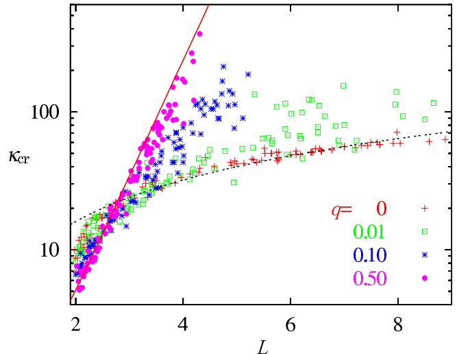
FIG. 3: (color online) Dependence of the entrainment threshold on the depth L for an ensemble of small-world networks with N = 100, k = 3 and different randomness q . The solid line is the same exponential function as that fitted to the data with pN = 6 (= 2k) in Fig. 2. The dotted line is linear fitting for the regular lattice ( q = 0 ).
