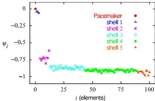
FIG. 1: (color online) Phases of elements in the entrained state; N = 100 , p = 0.05 , N_1 = 3 , \kappa = 100 and \mu = 1000 .
