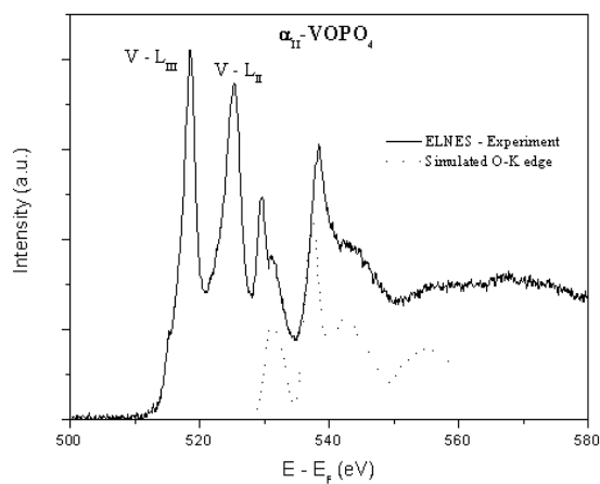
Fig. 6. EELS spectrum recorded from \alpha_{II} -VOPO 4 .
