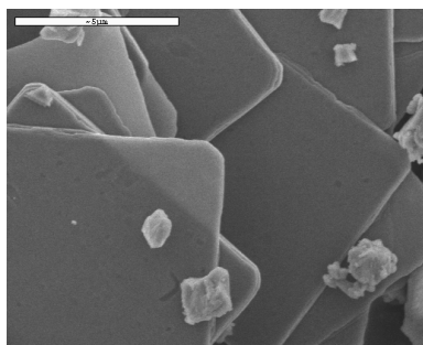
Fig. 1. SEM image of \alpha_{II} -VOPO 4
