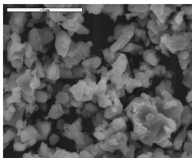
Fig. 2. SEM image of \beta -VOPO 4
