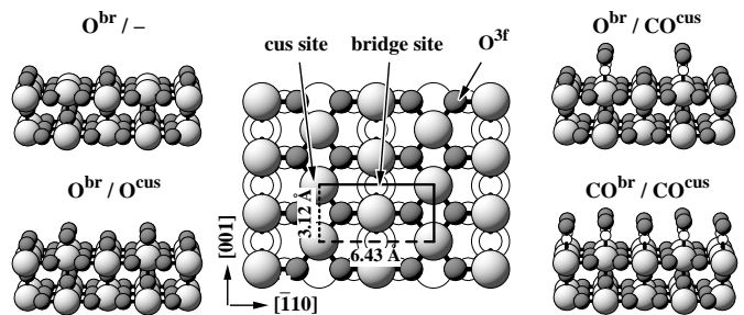
FIG. 2: Top view of the RuO 2 (110) surface explaining the location of the two prominent adsorption sites (bridge and cus), which continue the bulk-stacking sequence (central panel). Also shown are perspective views of the two most stable terminations involving only O (left panel) and involving O and CO (right panel). Ru = light, large spheres, O = dark, medium spheres, C = white, small spheres. Atoms lying in deeper layers have been whitened in the top view for clarity.
