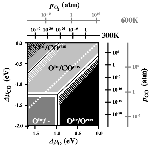
FIG. 5: Surface phase diagram of stable and metastable structures of RuO_2(110) in (\mu_O, \mu_{CO}) -space. The additional axes at the top/right give the corresponding pressure scales at T = 300\text{ K} and 600\text{ K} . The white regions close to the boundaries between different stable phases mark phase coexistence conditions, where at least 10% of the respective other phase is also present at the surface at T = 300\text{ K} . Regions marked by white hatching are particularly strongly affected by kinetics (see text). The white dotted line marks the stability limit of bulk RuO_2 with respect to CO-induced decomposition: In the upper left part above this line, RuO_2 is only metastable.
