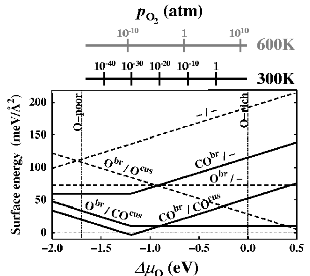
FIG. 3: Surface free energies of the three only O involving \text{RuO}_2(110)-(1 \times 1) terminations (dashed lines) and of three O and CO involving surface geometries (solid lines). Corresponding geometries are explained in the left and right panels of Fig. 1, respectively. The dotted vertical lines indicate the allowed range of oxygen chemical potential, cf. eq. (9), while \Delta\mu_{\text{CO}} = 0.0 \text{ eV} , corresponding to very CO-rich conditions. In the top x -axis, the dependence on \Delta\mu_{\text{O}}(T, p_{\text{O}}) has been cast into pressure scales at fixed temperatures of T = 300 \text{ K} and T = 600 \text{ K} .
