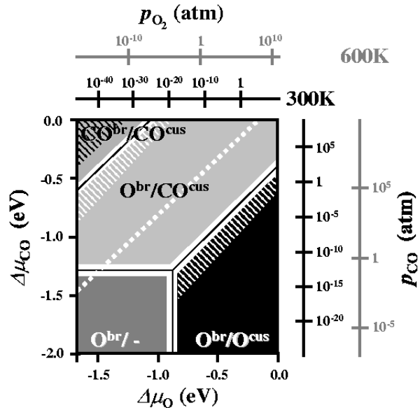
FIG. 6: Same as Fig. 4, but now computed using the LDA exchange-correlation functional.
