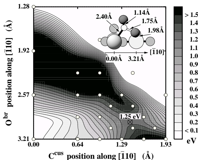
FIG. 7: Potential energy surface for the reaction \text{CO}^{\text{cus}} + \text{O}^{\text{br}} \rightarrow \text{CO}_2 . The lateral positions of \text{C}^{\text{cus}} and \text{O}^{\text{br}} along the [\bar{1}10] direction connecting the cus site with the neighboring bridge site, cf. the dashed line in Fig. 1, have been constrained, fully relaxing all remaining degrees of freedom. Actually calculated points are indicated by white circles. The energy zero corresponds to the initial state at (0.00 Å, 3.21 Å) and the transition state geometry is shown in the inset (only the atoms lying in the reaction plane itself are drawn as threedimensional spheres).
