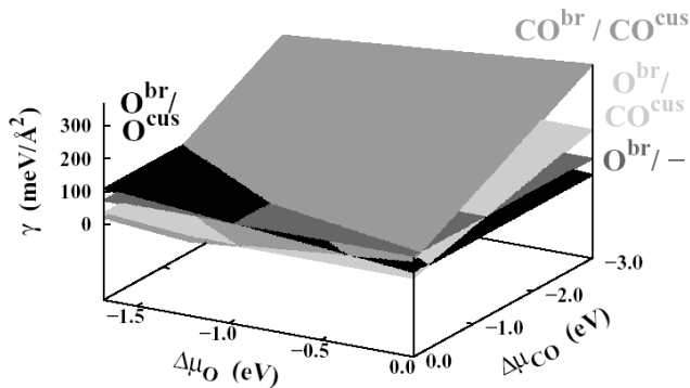
FIG. 4: Surface free energies of the four stable geometries shown in Fig. 1, as a function of (\Delta\mu_O, \Delta\mu_{CO}) .
