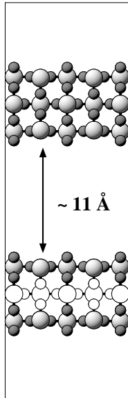
FIG. 1: Sideview of the chosen supercell setup (Ru = light, large spheres, O = dark, medium spheres). Each slab consists of three O-(RuO)-O trilayers, and the atoms of one such trilayer have been whitened in the lower slab. Consecutive slabs are separated by a vacuum region of \approx 11 \text{ \AA} .
