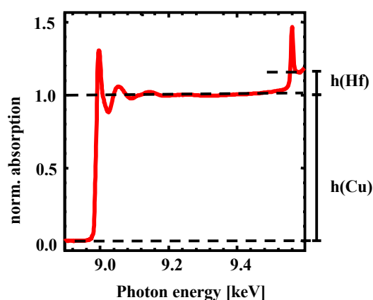
Fig. 3. Normalized Cu K edge absorption spectra of \text{Cu}/\text{ZrO}_2 together with the Hf L_{3-} edge.
