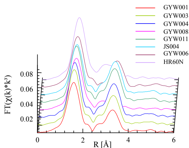
Fig. 1. Zr K edge radial distribution functions of various \text{Cu}/\text{ZrO}_2 catalysts.
