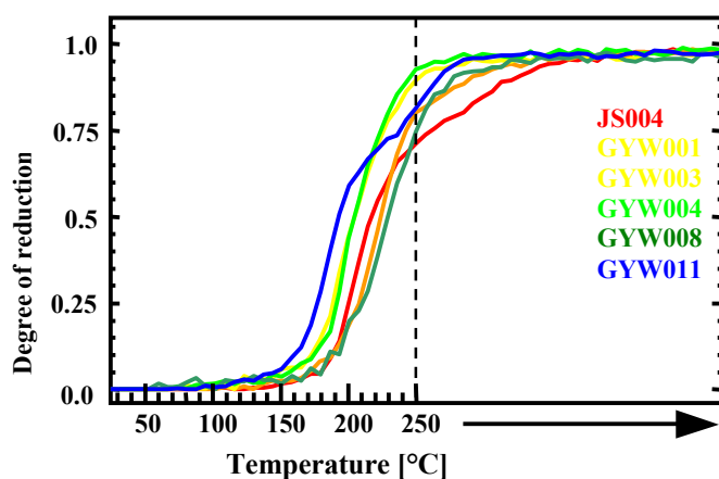
Fig. 2. In situ Cu K XANES measured during TPR of Cu in differently prepared \text{Cu}/\text{ZrO}_2 catalysts (heating rate 10K/min to 250°C in 2 % \text{H}_2/\text{He} ).
