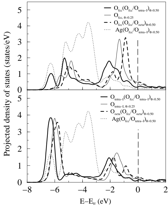
FIG. 7. Total projected density of states (PDOS) for the favorable (O_{\text{fcc}}/O_{\text{tetra-I}})_{\theta=0.50} and unfavorable (O_{\text{fcc}}/O_{\text{octa}})_{\theta=0.50} structures. PDOS for O_{\text{fcc}} (upper figure) and O_{\text{tetra-I}} (lower figure) are shown by thick solid lines, and the silver atoms shared by the two oxygen atoms are shown as dotted lines. For comparison, O_{\text{fcc}} without the presence of sub-surface oxygen (thin solid line) and with sub-surface oxygen in the octa site (thick dashed line) are shown in the upper figure. Also for comparison (lower figure) are the PDOS for O_{\text{tetra-I}} without on-surface oxygen (shown as thin solid line) as well as sub-surface O in the octa site of the unfavorable structure (thick dashed line). The energy zero is the Fermi energy.
