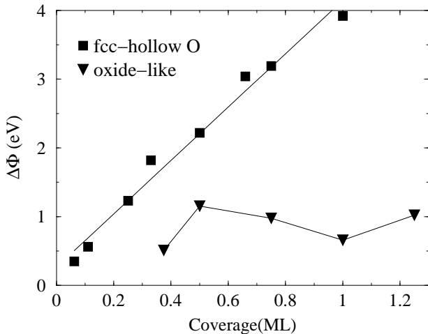
FIG. 11. Work function change for on-surface O adsorption in the fcc site (squares) (from Ref. 34) and of the (4 \times 4) and the oxide-like structures with higher oxygen concentrations (triangles).
