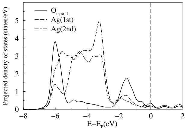
FIG. 4. Total projected density of states (PDOS) for oxygen in the sub-surface tetra-I site for coverage 0.25 ML. The Ag PDOS of the first and second metal layer atoms that are bonded to oxygen are indicated by dashed and dot-dashed lines, respectively, and the O PDOS is indicated by a solid line. The vertical dashed line marks the Fermi energy.
