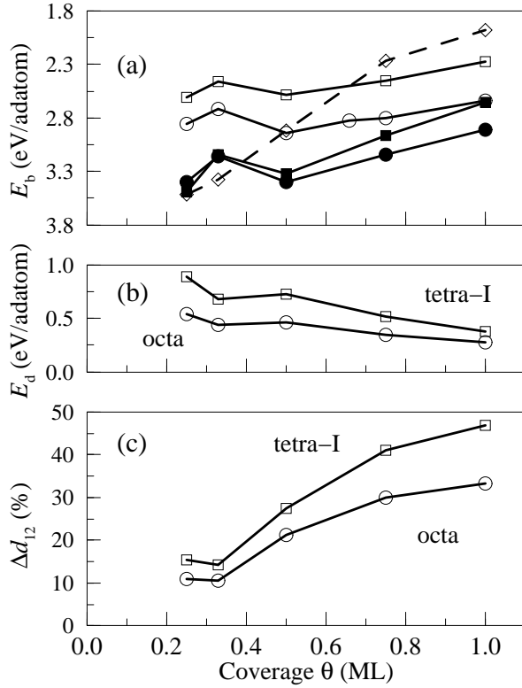
FIG. 2. (a) Binding energies of O on the pre-distorted substrate, E_b , in the octa (filled circles) and tetra-I sites (filled squares) and the corresponding adsorption energies, E_{ad} , of O in the octa (open circles) and tetra-I (open squares) sites. The adsorption energies of on-surface fcc-O are also shown (open diamonds). (b) Energy cost, E_d , of distorting the substrate lattice to the geometry induced by sub-surface oxygen (but without the presence of oxygen) for the octa (open circles) and tetra-I (open squares) sites. (c) Percentage change of the first metal interlayer distance compared to the bulk value for the octa (circles) and tetra-I (squares) sites.
