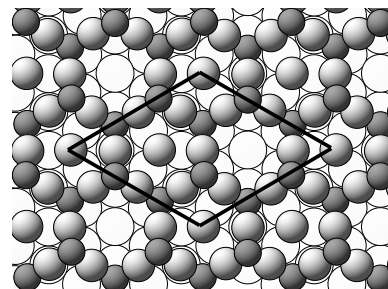
FIG. 9. Sketch of the atomic structure proposed in the STM study of Ref. 32 for the (4 \times 4) phase. The surface unit cell is indicated. The oxygen atoms are represented by small dark circles, the uppermost Ag atoms by grey circles, and the intact plane of \text{Ag}(111) atoms lying below the ‘O-Ag-O’ trilayer are represented as the open circles.
