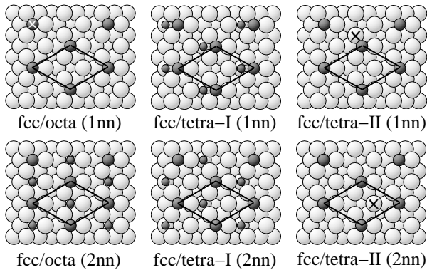
FIG. 6. Schematic geometry of the (2 \times 2) surface unit cells with on-surface oxygen in the fcc site, O_{\text{fcc}} , (larger dark circles) for a coverage of 0.25 ML. The various sub-surface sites are depicted as the small dark circles and the resulting on-surface+sub-surface geometries defined by the label (e.g. fcc/octa (1nn)). There are two different types of sub-surface sites; ones that are closest to O_{\text{fcc}} , denoted ‘1nn’ and ones that are further away, denoted ‘2nn’. Note, as indicated by the ‘x’ on the atoms, the 1nn- O_{\text{octa}} site is located directly below O_{\text{fcc}} and the tetra-II site is located directly below surface Ag atoms.
