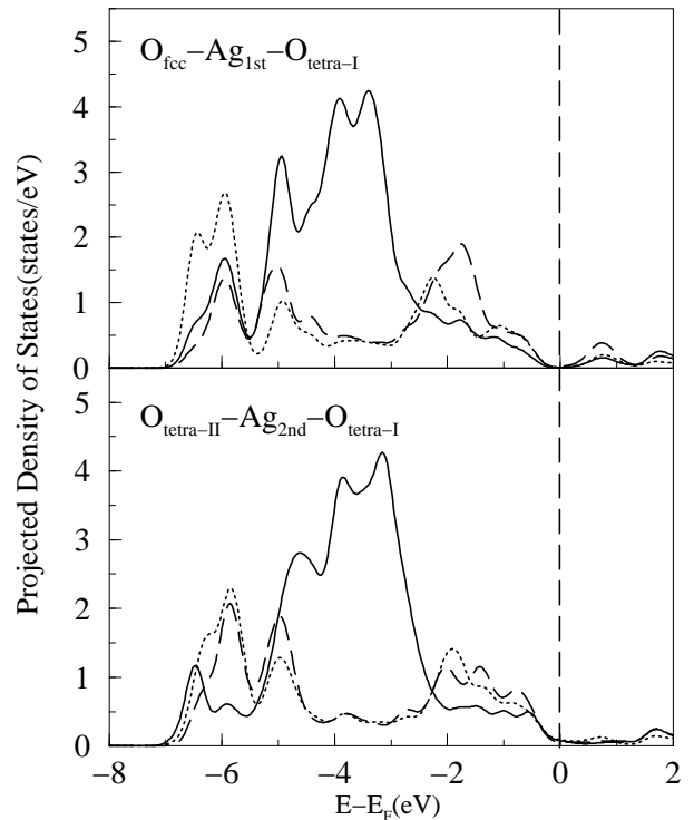
FIG. 12. Total projected density of states for the oxide-like structure (O_{\text{fcc}}/O_{\text{tetra-I}}+O_{\text{tetra-II}}/O_{\text{tetra-I}}+O_{\text{tetra-II}})_{\theta=1.25} . The upper figure shows the PDOS for O_{\text{fcc}} (dashed line), the uppermost Ag atoms bonded to both O atoms (solid line) and O_{\text{tetra-I}} (dotted line) under the first layer. The lower figure shows the PDOS for O_{\text{tetra-II}} (dashed line) under the first metal layer, the shared Ag atom (solid line) and O_{\text{tetra-I}} (dotted line) under the second metal layer. The Fermi energy is indicated by the vertical dashed line.
