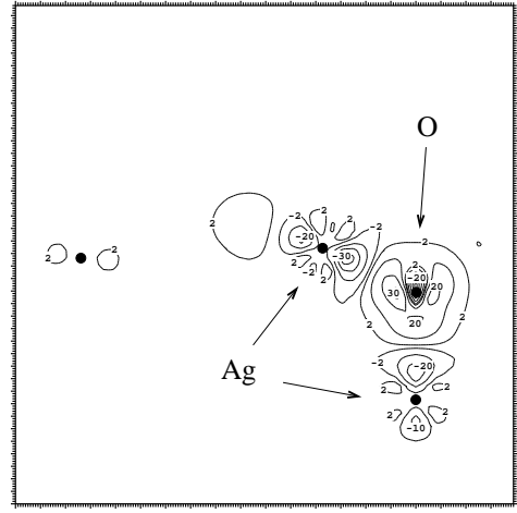
FIG. 3. The difference electron density, n(\mathbf{r})^\Delta , (see the definition in Ref. 34) for oxygen in the sub-surface tetra-I site for coverage 0.25 ML. The contour plane is in the [211] direction and is perpendicular to the Ag(111) surface. The unit is 10^{-3} Bohr ^{-3} . The positions of the O and Ag atoms are indicated by the arrows.
