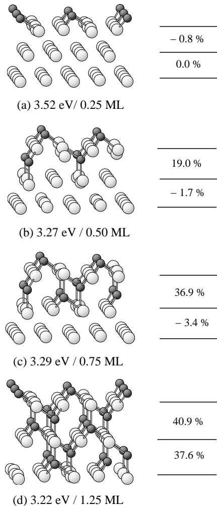
FIG. 10. Atomic geometry of energetically favorable structures for increasing oxygen concentrations: (a) on-surface fcc oxygen, (b) fcc oxygen plus sub-surface oxygen in the tetra-I site, (c) as for (b) but with additional oxygen in the tetra-II site, (d) as for (c) but with additional oxygen under the second Ag layer in the tetra-I and tetra-II sites. The average adsorption energy with respect to the clean Ag(111) substrate and free oxygen atoms, as well as the corresponding coverage, are given at the bottom of each figure. The relative variation of the first and second interlayer spacings with respect to the bulk value is also given to the right of the figures. Large pale grey and small dark circles represent silver and oxygen atoms, respectively.
