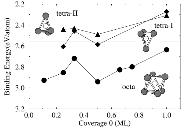
FIG. 1. Calculated adsorption energy of oxygen (with respect to atomic oxygen) under the first Ag(111) layer in octa (circles), tetra-I (diamonds), and tetra-II (triangles) sites, as a function of coverage. The horizontal full line represents half the experimental value of the binding energy of \text{O}_2 (2.56 eV). The solid lines connecting the calculated adsorption energies are to guide the eye.
