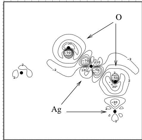
FIG. 8. The difference electron density, n(\mathbf{r})^{\Delta} (see the definition in Ref. 34) for (O_{\text{fcc}}/O_{\text{tetra-I}})_{\theta=0.50} . The contour plane is in the [211] direction and is perpendicular to the \text{Ag}(111) surface. The unit is 10^{-3} \text{ Bohr}^{-3} . The positions of the O and Ag atoms are indicated by the arrows.
