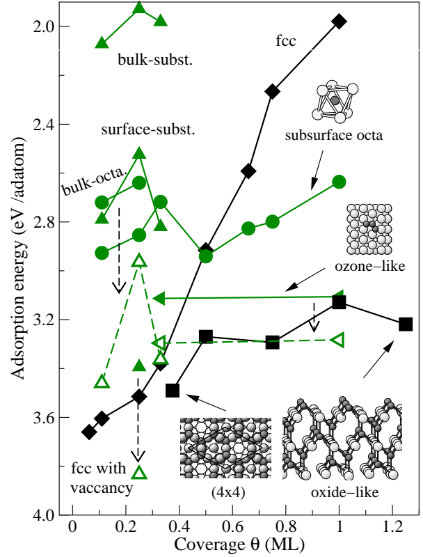
FIG. 14. Average adsorption energy (with respect to atomic O) versus coverage for the different structures considered: pure on-surface oxygen in fcc-hollow sites (diamonds), surface- and bulk-substitutional adsorption (triangles), pure sub-surface oxygen in octahedral sites under the first (subsurface-octa.) and second (bulk-octa.) Ag layers (circles), an ozone-like molecule adsorbed at a surface Ag vacancy (left-pointing triangles), and surface oxide-like structures (squares), as illustrated in Fig. 10. The vertical downward pointing arrows directed at dashed lines with open symbols, indicate the corresponding binding energies of the structures involving surface Ag vacancies, i.e. the vacancy formation energy, E_f^{\text{vac}} (see Ref. 34 for the definition), is not taken into account. The adsorption energy of O in the fcc site (triangle) with a neighboring surface Ag vacancy is also shown for \theta = 0.25 ML, as well as the corresponding binding energy.
