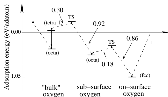
FIG. 5. Adsorption energy of oxygen at a coverage of 0.11 ML for penetration into the sub-surface octa site from the on-surface fcc-hollow site through the first Ag layer, and from the octa site to the “bulk” tetrahedral site, through the second Ag layer (from right to left). From the tetra-I site O will move to the more favorable “bulk” octa site under the second Ag layer. The short lines indicate the adsorption energy with respect to half of the binding energy of the oxygen molecule (experimental value). “TS” represents the transition states, and the numbers on the arrows indicate the energy barriers.
