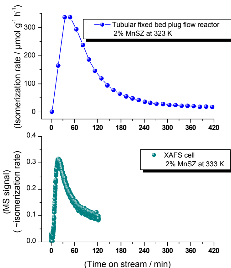
Figure 3. Time on stream profiles for 2% Mn promoted sulfated zirconia catalyst in 1% n -butane in a fixed bed reactor (above) and in the XAS cell (bottom).
