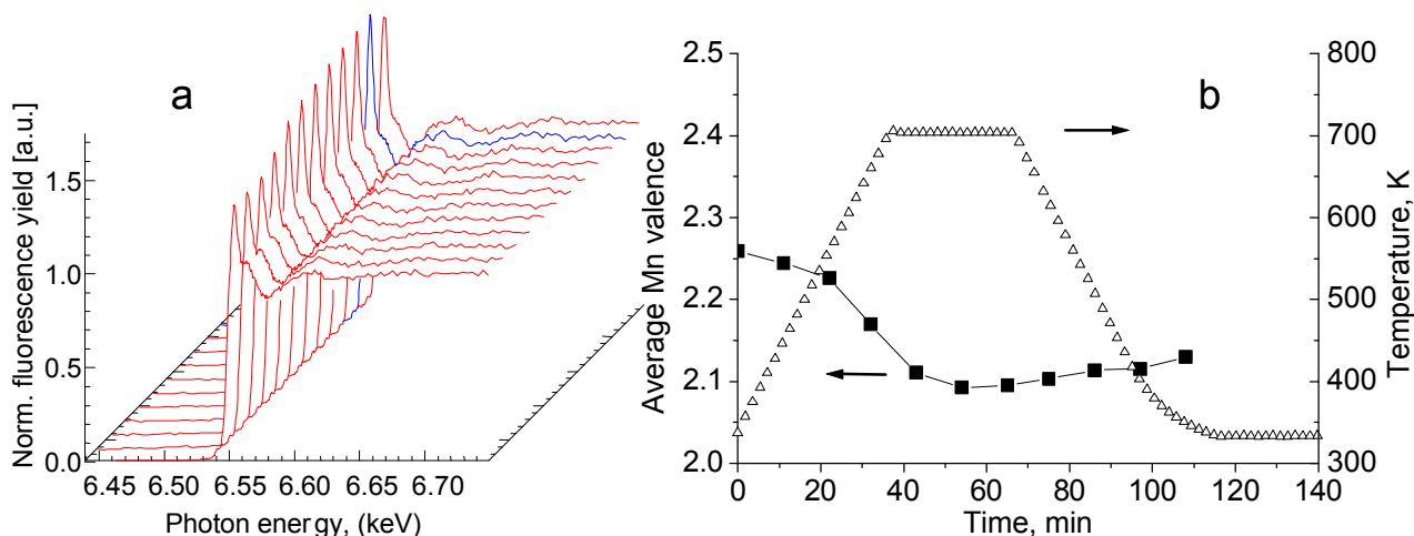
Figure 2. a) Mn K-edge X-ray absorption spectra of a 2% Mn promoted sulfated zirconia catalyst during reduction in 50% hydrogen for 30 minutes at 703 K. b) Average Mn valence during reduction calculated from data presented in 3a.
