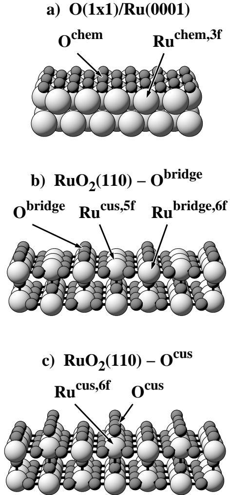
FIG. 1. Surface structures of domains on O-rich Ru(0001): a) Chemisorbed O(1 × 1)/Ru(0001) with threefold O chem coordinated Ru chem,3f surface atoms. b) Stoichiometric RuO 2 (110)-O bridge termination with five-, six- and twofold coordinated Ru cus,5f , Ru bridge,6f and O bridge atoms respectively. c) High-pressure RuO 2 (110)-O cus termination, where additional O cus atoms sit atop the formerly undercoordinated Ru cus,6f atoms (Ru = large, light spheres, O = small, dark spheres).
