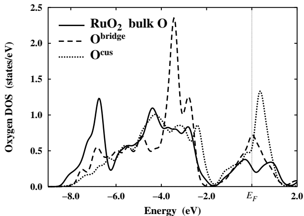
FIG. 2. Calculated DOS for bulk O in \text{RuO}_2 (solid line), as well as for \text{O}^{\text{bridge}} and \text{O}^{\text{cus}} atoms (dashed and dotted lines respectively) in the \text{RuO}_2(110)\text{-O}^{\text{cus}} termination. The \text{O}^{\text{bridge}} DOS in the \text{RuO}_2(110)\text{-O}^{\text{bridge}} termination is almost identical to the one shown here. The energy zero is at the Fermi level.
