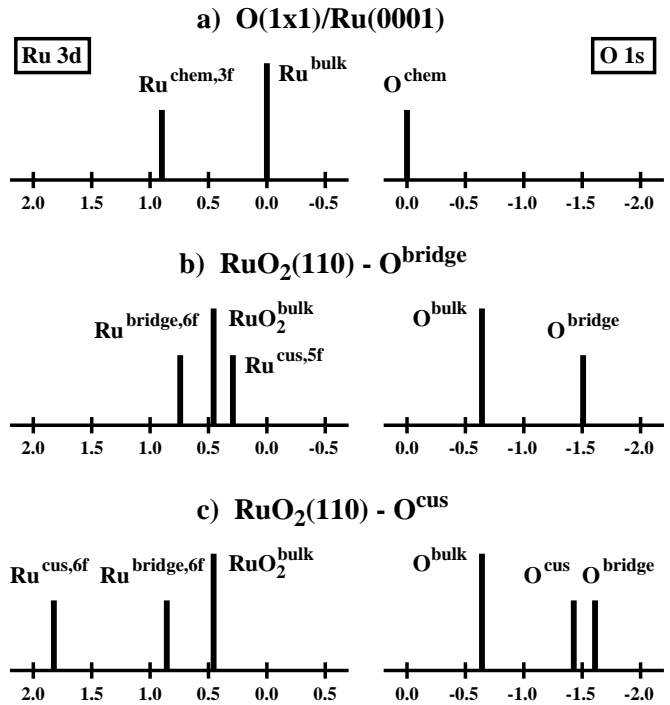
FIG. 3. Computed fully-screened Ru 3d and O 1s SCLSs for the three domain types on an oxygen-rich Ru(0001) surface. Ru in the metallic bulk and O in the \text{O}(1 \times 1)/\text{Ru}(0001) phase are used as zero reference. Units are eV.
