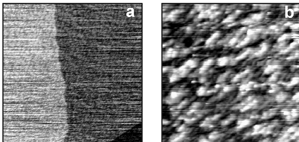
Fig. 2. 5,000 \times 5,000 \text{ \AA}^2 (a) and 750 \times 750 \text{ \AA}^2 (b) STM images of the Pt(100) surface after deposition of \sim 1\text{ML} of metallic iron. The surface is roughened with an average corrugation of \sim 1.5 \text{ \AA} , as shown on (b). Monoatomic steps of the original Pt substrate are visible on image (a).
