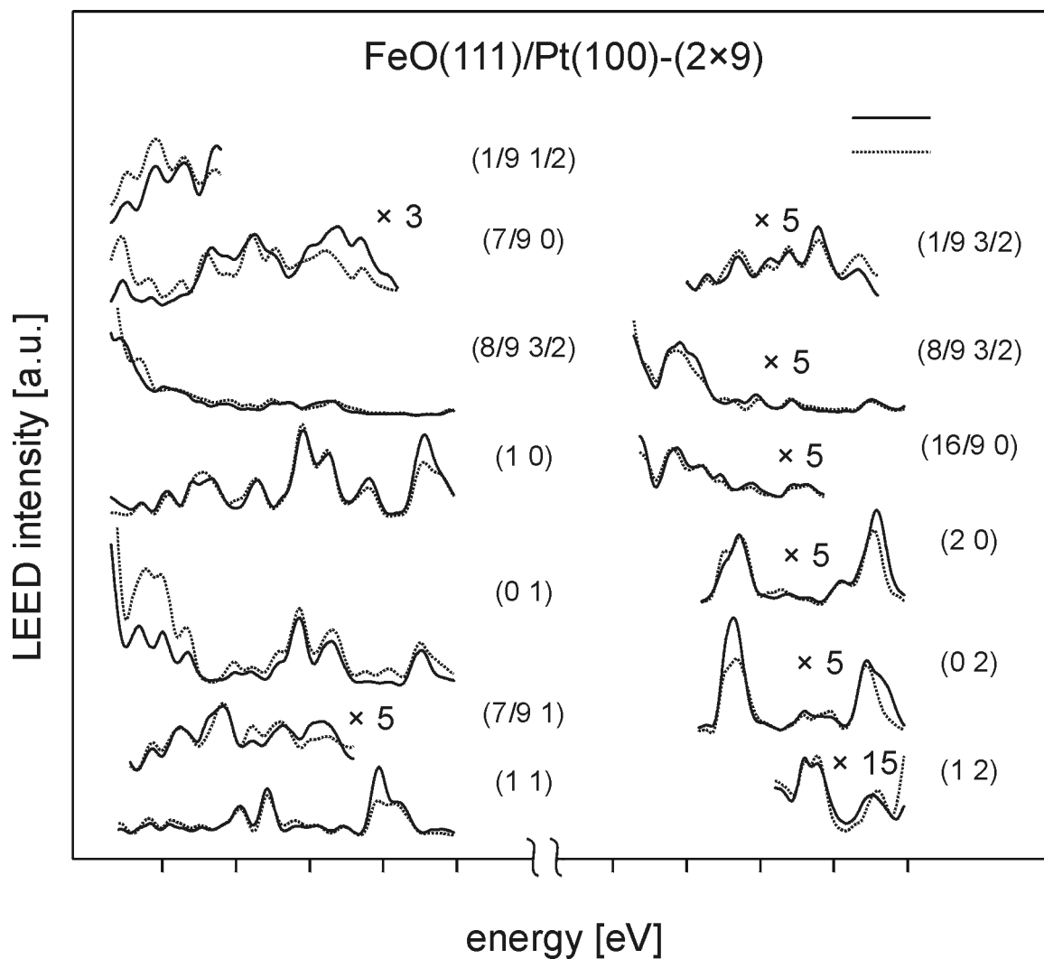
Fig. 6. Comparison of the experimental and simulated I-V curves for the best fit structure obtained on the FeO(111)/Pt(100)-(2x9) surface. The data set covers a total energy range of 2200 eV. The best fit has a Pendry R-factor of 0.15 ( \pm 0.02 ).
