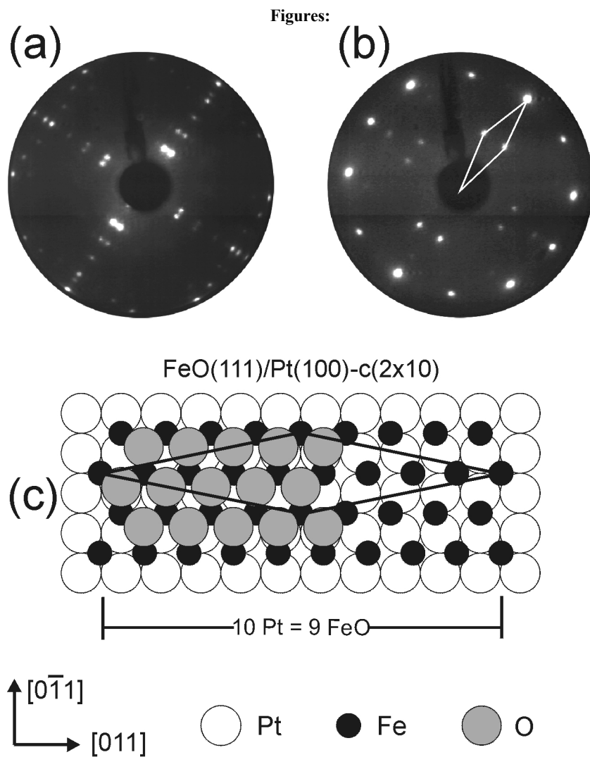
Fig. 1. LEED patterns of the Pt(100)-hex (a) and of the FeO(111)/Pt(100) (b) surfaces at electron energy of E=50 eV. The arrows indicate the spots coming from two orthogonal domains. (c) Top view of the model illustrating a FeO(111)/Pt(100)-c(2x10) coincidence structure. For clarity, not all top atoms are drawn.
