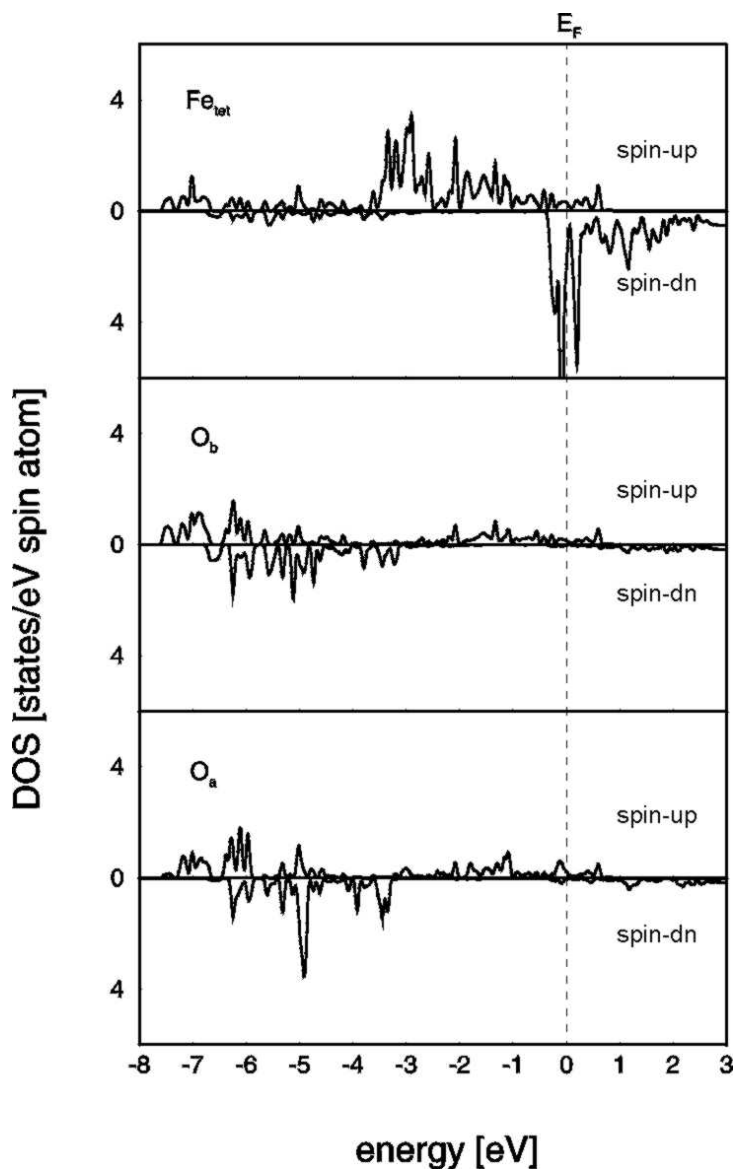
Fig. 3: Partial electron density of states for the first two atom layers of the \text{Fe}_3\text{O}_4(111) surface termination depicted in Fig. 1, obtained from ab-initio spin density functional theory calculations. Near the Fermi level E_F the DOS is dominated by 3d states related to \text{Fe}_{\text{let}1} surface atoms, 2p states related to the two symmetrically inequivalent \text{O}_a and \text{O}_b atoms dominate at binding energies below -4 eV.
