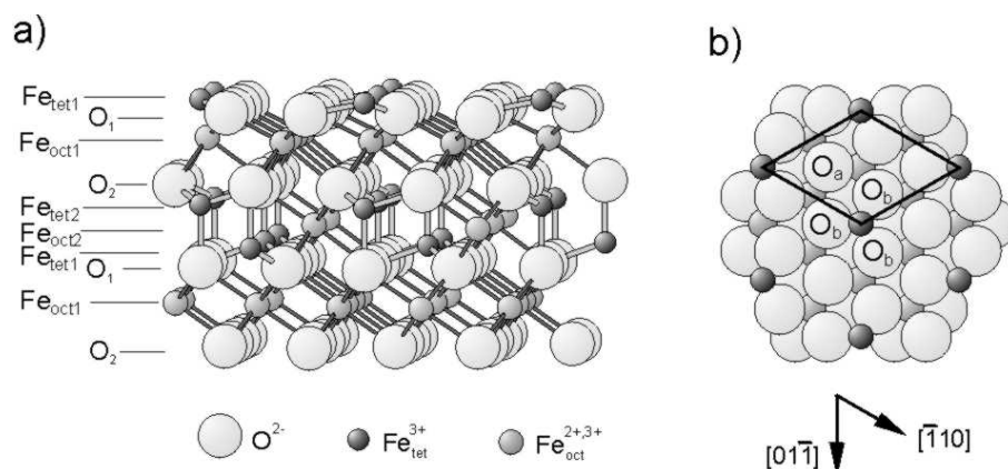
Fig. 1: Slightly tilted side view (a) and top view (b) of the \text{Fe}_3\text{O}_4(111) surface structure as determined by the LEED intensity analysis. On the left side the (111) layer sequence with tetrahedrally coordinated \text{Fe}_{\text{tet}1} or \text{Fe}_{\text{tet}2} atoms, with octahedrally coordinated \text{Fe}_{\text{oct}1} or \text{Fe}_{\text{oct}2} atoms, and with \text{O}_1 and \text{O}_2 layers is indicated. In (b) the surface unit cell with a lattice constant of 5.94 \text{ \AA} and the two symmetrically inequivalent oxygen atoms \text{O}_a and \text{O}_b are indicated. In the side view the ionic radii are reduced by a factor of 0.5, the top view is drawn with the full ionic sizes.
