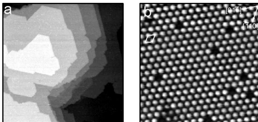
Fig. 2: a) 3000 \times 3000 \text{ \AA}^2 STM image showing the characteristic morphology of the \text{Fe}_3\text{O}_4(111) films. Atomically flat terraces up to 1000 \text{ \AA} wide are separated by atomic steps \sim 5 \text{ \AA} high. U_t = 1.4 \text{ V} , I_t = 0.8 \text{ nA} . (b) 90 \times 90 \text{ \AA}^2 STM image of the regular \text{Fe}_3\text{O}_4(111) surface. Protrusions form a hexagonal lattice with the 6 \text{ \AA} periodicity indicated by the unit cell. They are attributed to the topmost layer \text{Fe}_{\text{tet}1} atoms (see. Fig. 1b), the missing protrusions to \text{Fe}_{\text{tet}1} vacancies. U_t = -0.9 \text{ V} , J_t = 0.5 \text{ nA} .
