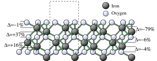
FIG. 1. Upper half of the slab for the unrelaxed \text{O}_3 -terminated surface. The cross section of the upper half of the supercell is noted by the dashed rectangle. The \Delta indicate the calculated interlayer relaxations in % relative to an unrelaxed surface, i.e., a truncated bulk geometry.
