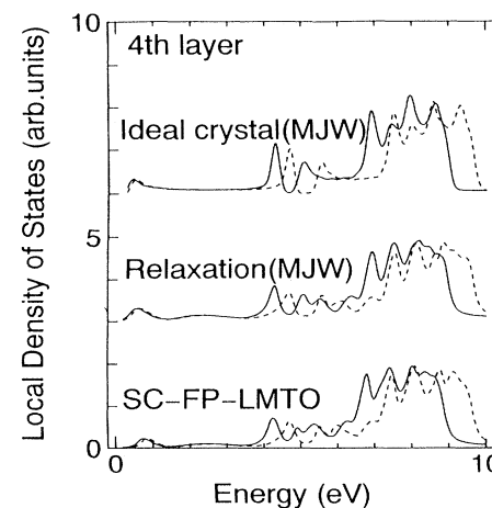
FIG. 5. Comparison of the three calculated local density of states for electron of Ni(100) surface for the fourth layer. The energy is measured from the muffin-tin-zero \bar{\Gamma} point. The solid lines are for electron having majority spin and dashed lines are for electron having minority spin.
