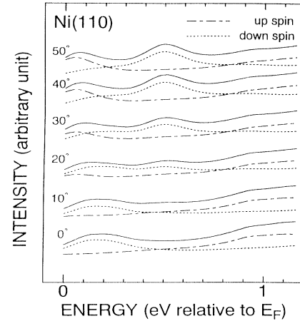
FIG. 13. Spin-resolved calculated inverse photoelectron spectra for Ni(110) surface with various emission direction. The dash-dotted and the dotted lines correspond to the majority and the minority spin spectrum using potentials obtained by self-consistent full-potential LMTO calculation. The solid lines are for the sum of the up spin and the down spin. The experiment condition is the same as that of Fig. 12.
