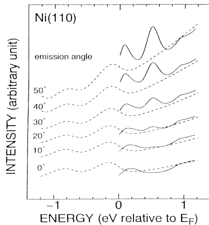
FIG. 12. Calculated inverse photoelectron spectra for Ni(110) surface with various emission direction. The solid lines are for using potentials obtained by self-consistent full-potential LMTO calculation and dashed lines for four using bulk potential. The incident electron energy and incident angle are 9.4 eV and 25^\circ , respectively.
