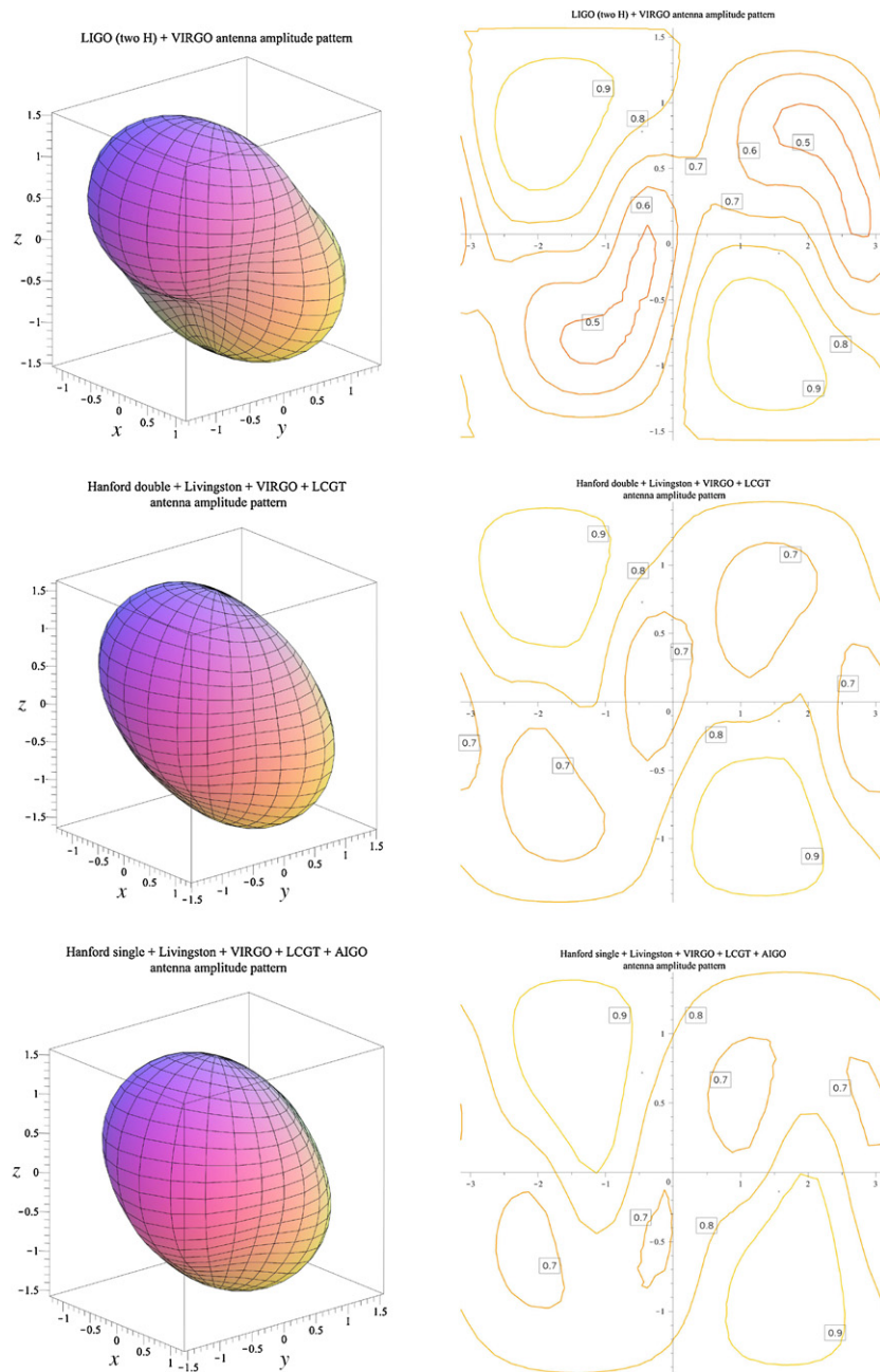
Figure 5. Three network amplitude patterns, which show the true spatial shape of the detection volumes. As in figure 3, two views are shown, one in perspective and the other as a contour plot. The networks are: (top row) the basic network of two instruments at Hanford, one at Livingston, and one at Pisa; (middle row) the basic network with LCGT in Japan added; (bottom row) the same after moving one of the Hanford detectors to Australia. Note that all these networks have roughly the same maximum range (HHLV: 1.74; HHJLV: 1.82; AHJLV: 1.76), and these are the values to which the contour levels are scaled. They have different volumes (HHLV: 8.98; HHJLV: 12.1; AHJLV: 12.1) because of their different isotropy, shown in figure 6. (The numbers are taken from table 2.)
