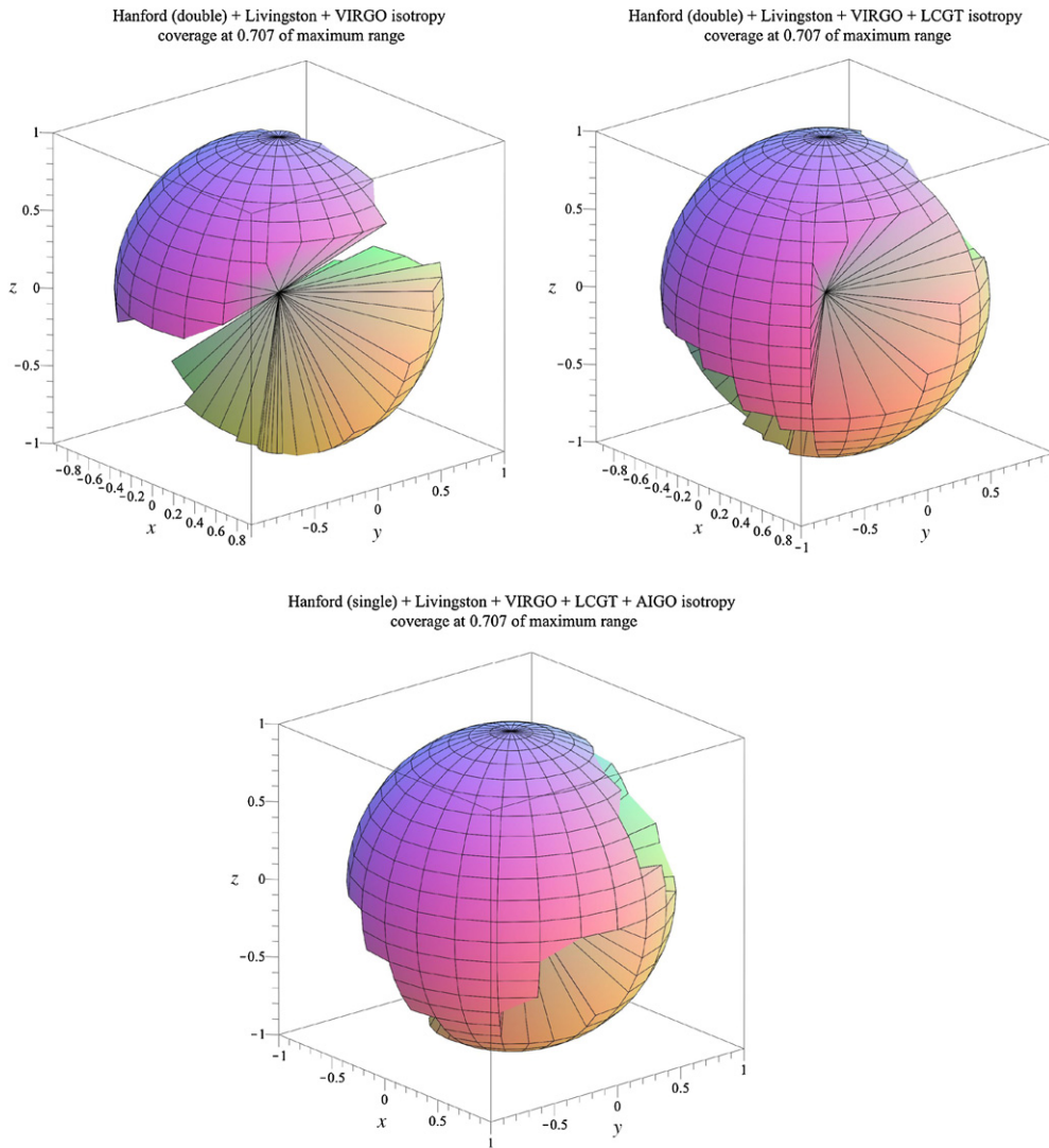
Figure 6. Three network isotropy patterns, which show the parts of the unit sphere where the amplitude sensitivity of the detector is better than \sqrt{2} of its best sensitivity. The networks are the same as in figure 5.
