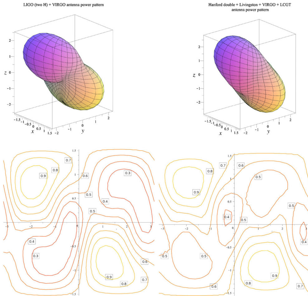
Figure 3. The antenna power patterns of the LIGO and VIRGO detector network with two detectors at Hanford (HHLV: left panel) and of the network after including the Japanese detector LCGT (HHJLV: right panel). All detectors are assumed to be identical. As in figure 2, the sensitivity is averaged over polarizations of the incoming wave. Top row: the coordinate system is oriented with z aligned with geographic north and the x -axis at geographic longitude 0^\circ . In all such plots from now on, the viewer is located at longitude 40^\circ W and 20^\circ N, above the mid-Atlantic. Note that all antenna patterns are reflection symmetric through the center of the earth, so that the hidden side is a mirror image of the side shown in the diagram. Bottom row: the same data plotted as contour plots. Contours are labeled with values relative to the maximum. For HHLV on the left, the maximum is 3.03 (square of the mean horizon distance from table 2). For HHJLV on the right, the maximum is 3.31.
