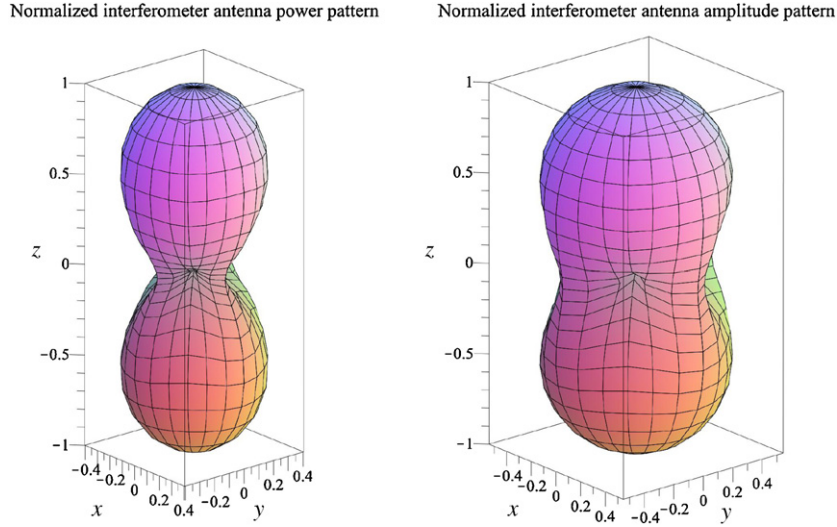
Figure 2. The antenna power pattern (left panel) and its square root (amplitude pattern: right panel) of a single interferometer oriented with axes in the x - y plane, averaged over polarizations of the incoming wave. The amplitude pattern represents the shape of the detection volume of the instrument, or its maximum detection reach in different directions.
