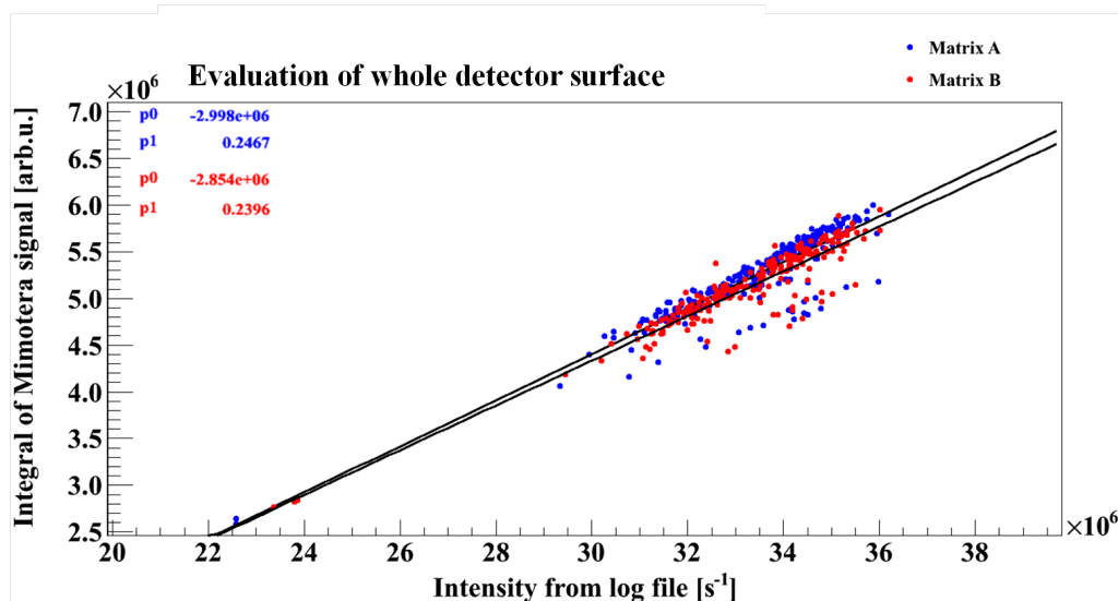
Figure 4.6: Integral taken over the whole detector surface compared to log file.
