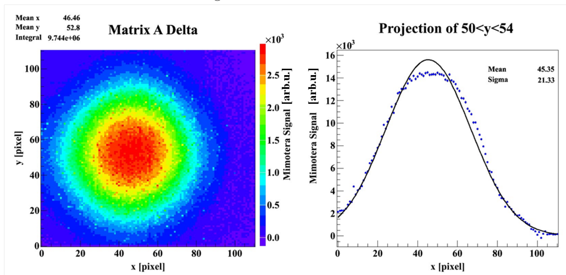
Figure 4.1: Profile PCB1.
