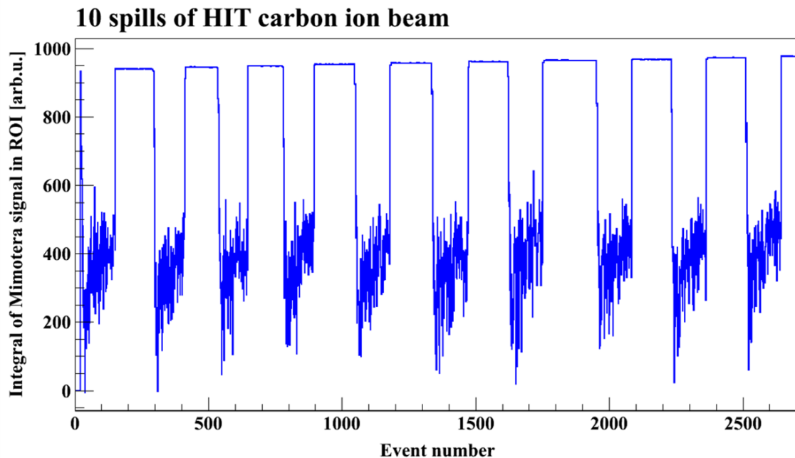
Figure 5.3: Spill structure of a carbon ion beam at HIT as measured by the Mimotera. The length of each spill is 5 s. Lower y-values correspond to a higher signal in the detector. The fluctuations during one spill go up to \pm 30\% .
