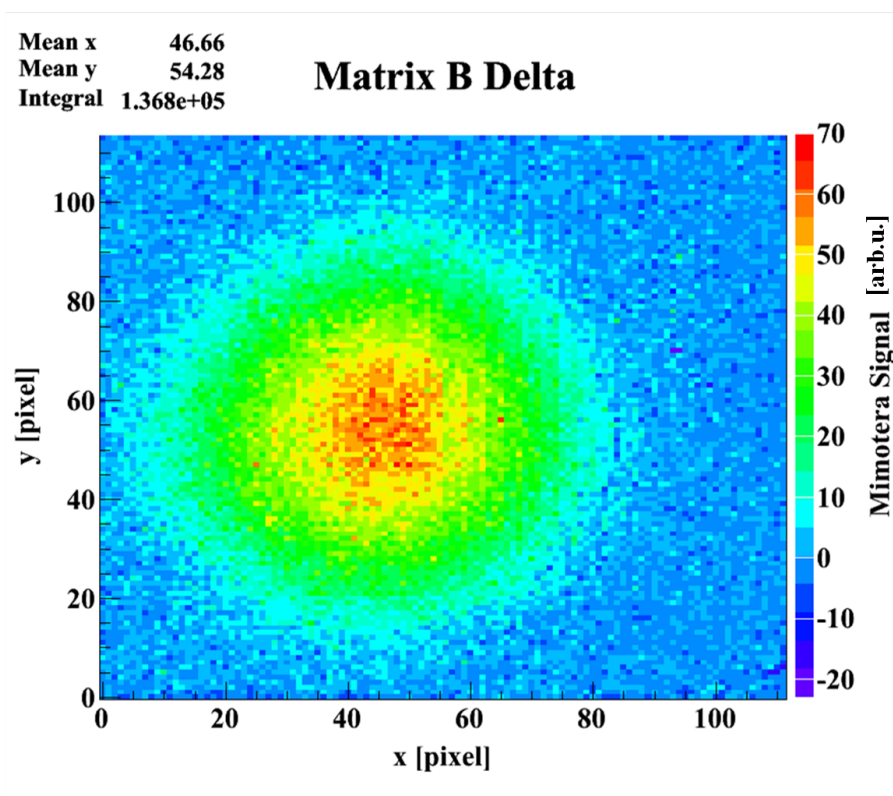
Figure 6.4: Difference of the Mimotera signal during 90 s after the beam spill, for the matrix in which the beam was recorded.
