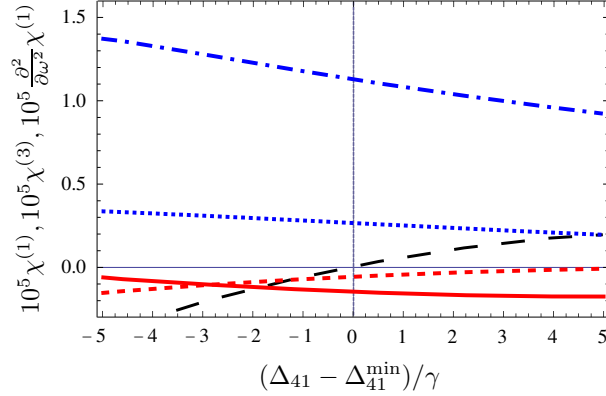
Figure 1.5: A magnification of Fig. 1.4 (d) around the probe field frequency \Delta_{41}^{\min} with vanishing group velocity dispersion [see Eq. (1.28)] is shown. The frequency axis is shown in units of the natural decay rate \gamma , which for the considered Sodium D1 transition is 2\pi \times 9.76 MHz. The parameters are the same as for Fig. 1.4 (d).
