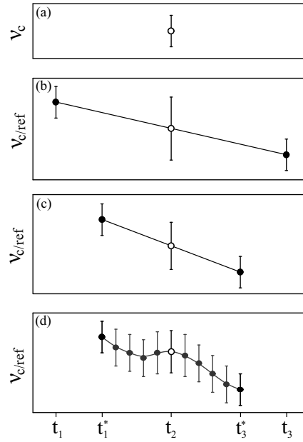
Figure 7.4: A measurement cycle of the new trap setup. Before ( t_1 ) and after ( t_3 ) a frequency measurement of the ion of interest at time t_2 (a), a reference ion is used to calibrate the magnetic field (b). The required linear extrapolation to the desired time increases the uncertainty (empty data point in the middle). This time period is significantly reduced, when both ion species are stored simultaneously in the trap setup. To avoid ion-ion interactions they are spatially separated and prepared in different trapping regions. Thus, they can be exchanged quickly during the measurement cycle (time t_1^* and t_3^* ) (c). A further reduction of the uncertainty can be achieved by a continuous B -field observation in the so called monitor traps. The relative magnetic field shifts are adopted to shifts in the precision trap (d).
