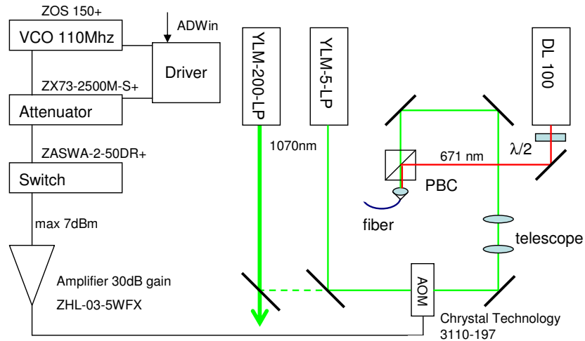
Figure 5.3: Preparation of the microtrap beam. 1070nm light from a our fiber laser is feed through an AOM for intensity stabilization and switching. After combining with an 671nm beam the light is coupled into an optical fiber. Additionally the AOM driver, which creates an adjustable rf signal for the piezo oscillation, is depicted.
