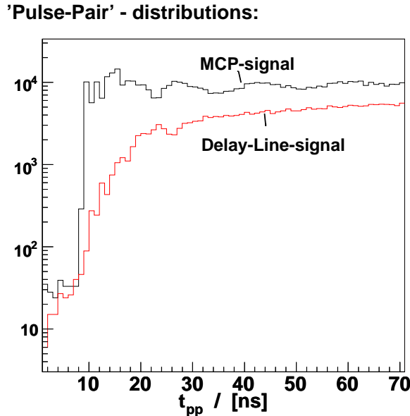
Figure 3.11: Number of recorded double-hits as a function of the time difference t_{pp} between two signal pulses, displayed for the MCP-signals and signals from one delay-line layer end. The so-called 'pulse-pair'-spectrum shows the deadtime of the electronic circuit.
