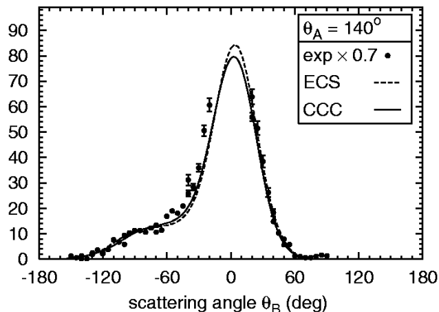
Figure 2.6: Absolute fully differential cross section (in 10^{-20} \text{ cm}^2 \text{ sr}^{-2} \text{ eV}^{-1} ) for single ionization of hydrogen at 17.6 eV impact energy and for equal energy sharing of the outgoing electrons. (From [Bra02])
