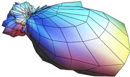
Figure A.2: Comparison of three dimensional cross section images (left) and the cuts in the scattering and perpendicular plane (right) for the two different ways of determining the momentum transfer.
