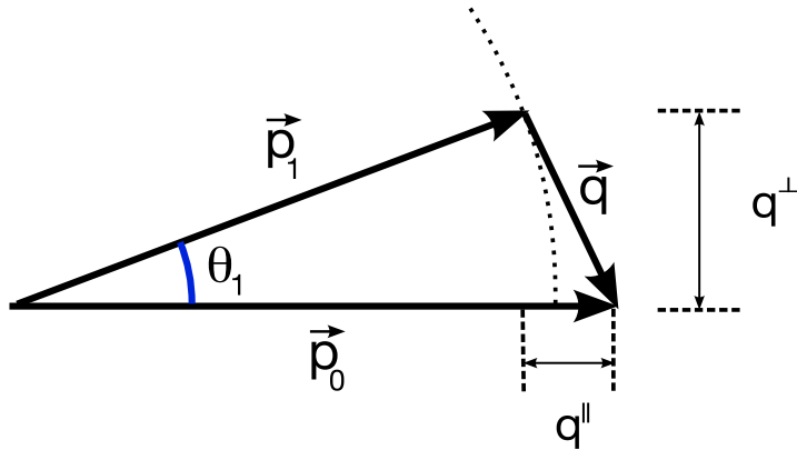
Figure A.1: Figure showing the kinematics of the scattered projectile in electron impact ionization and the asymmetric scattering geometry.
